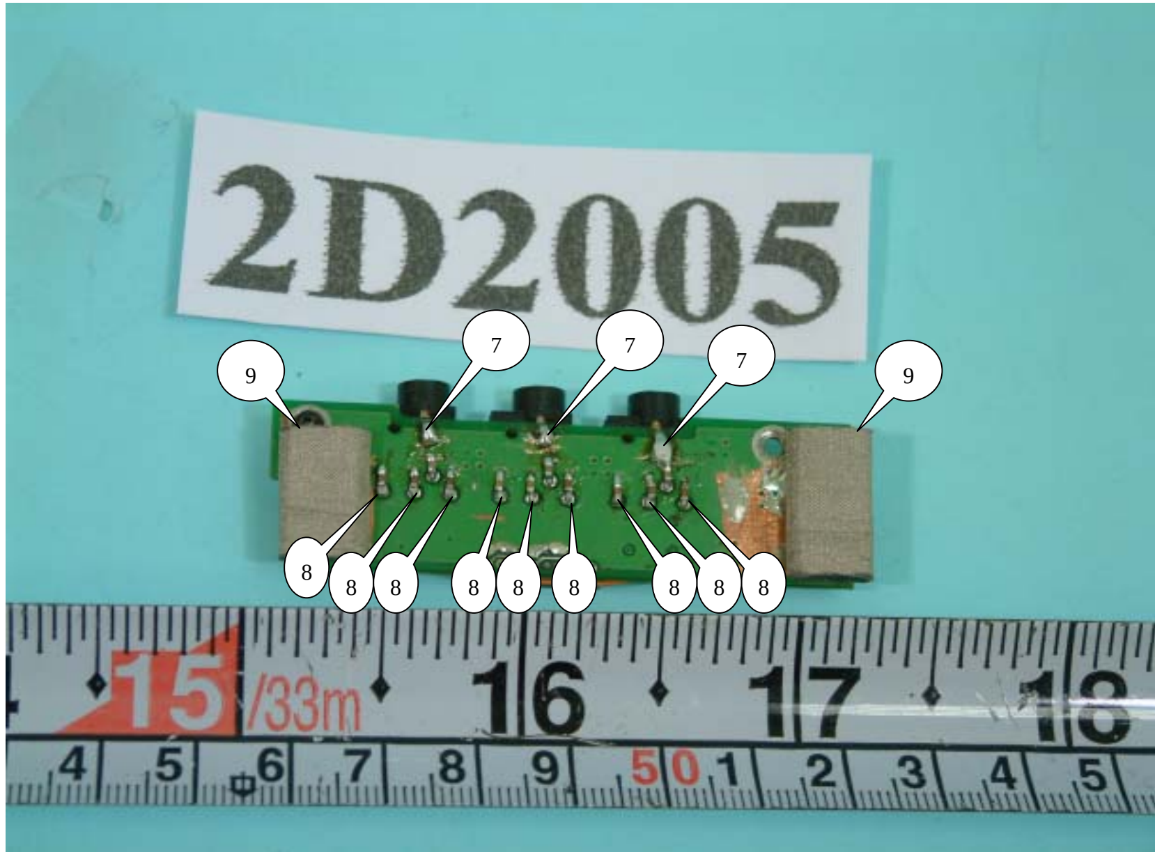
Rear side of audio board
