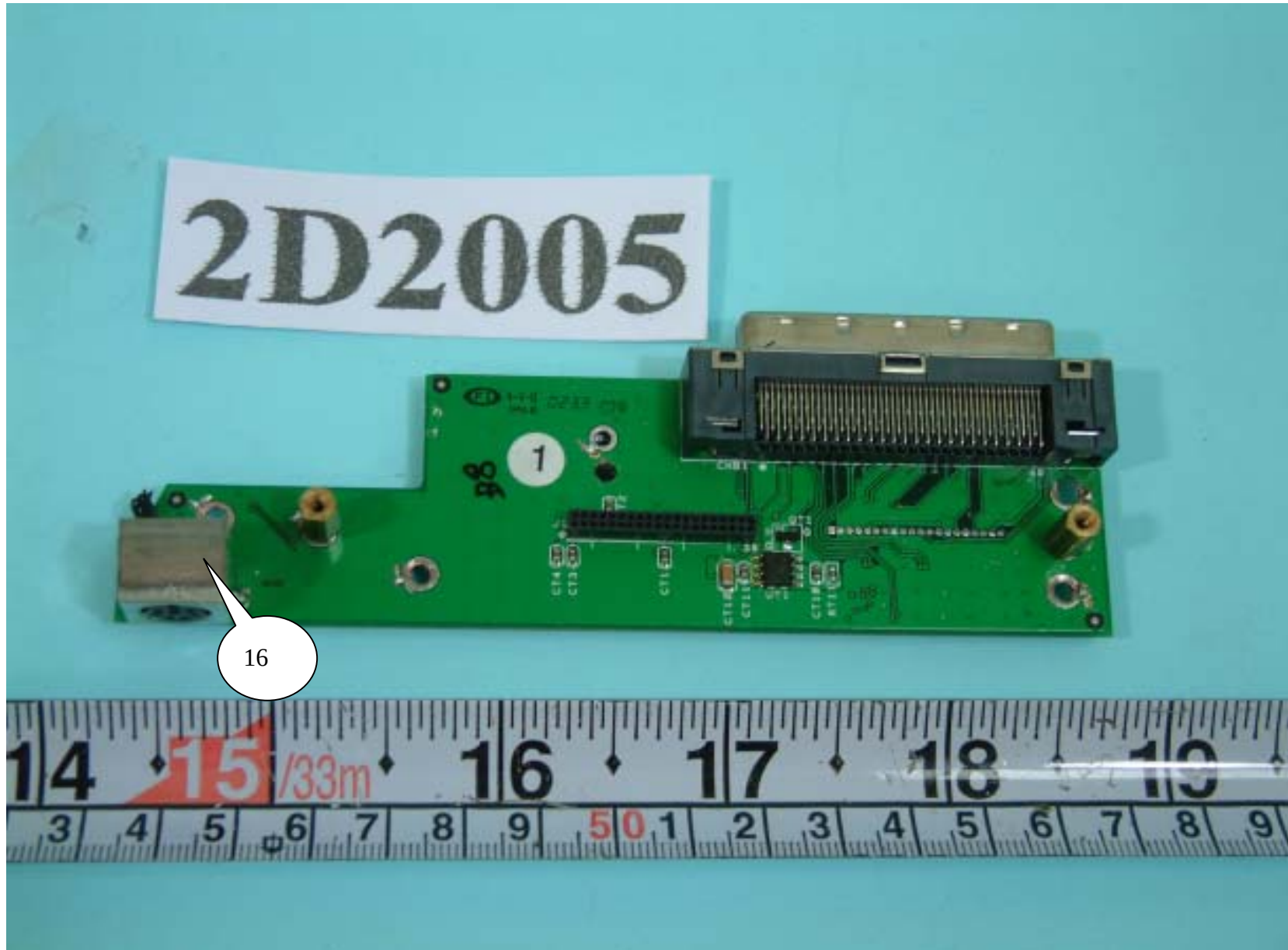
Front side of I/O stick's PS2 & connect port board
