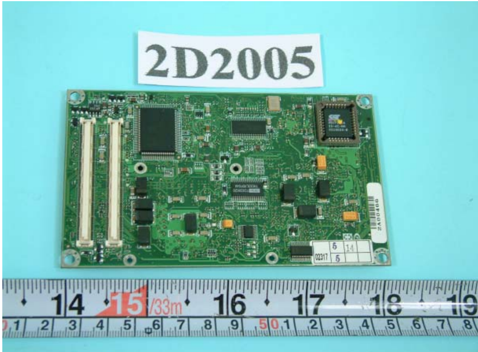
Rear side of cpu board
