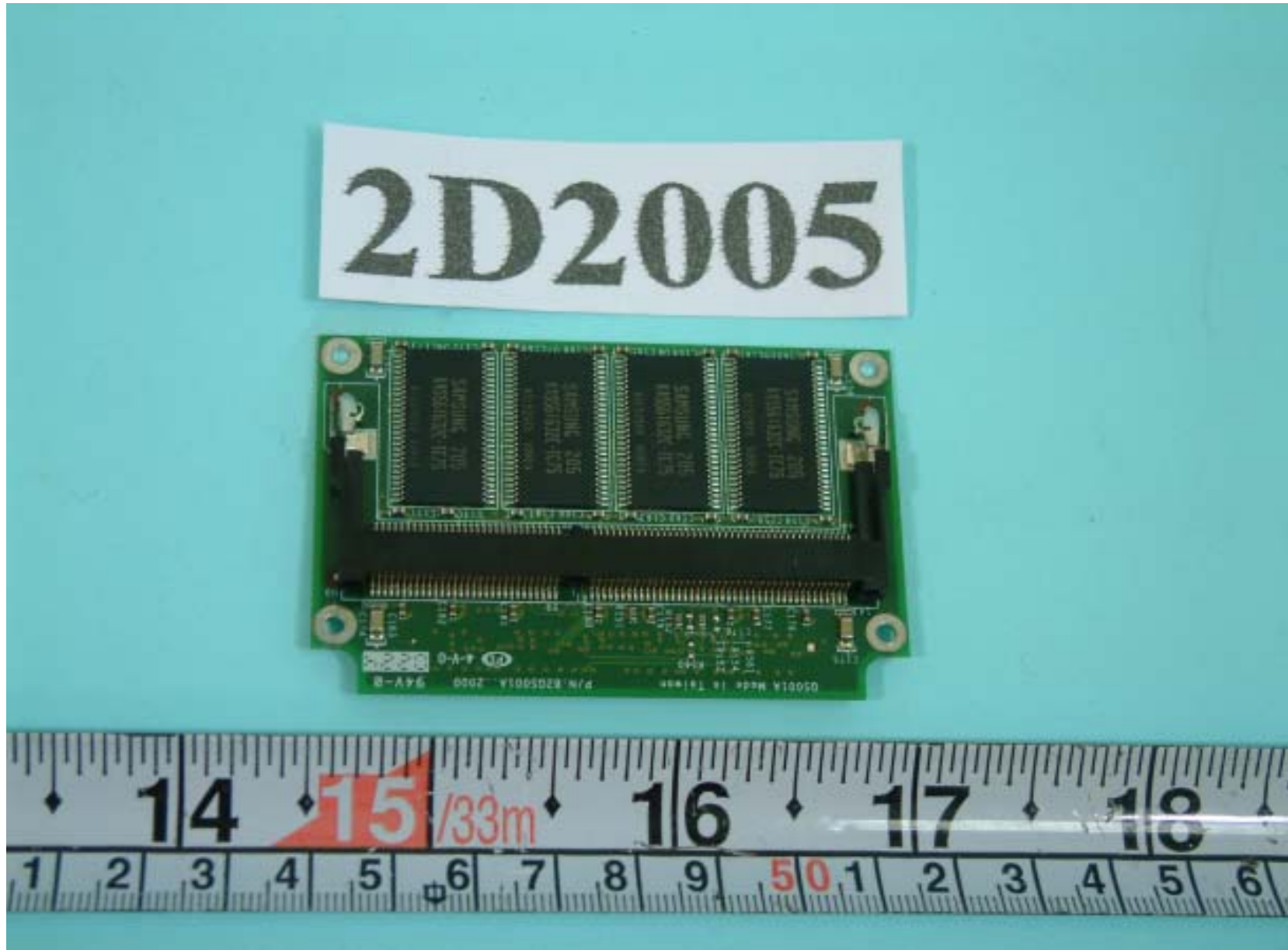
Front side of memory module
