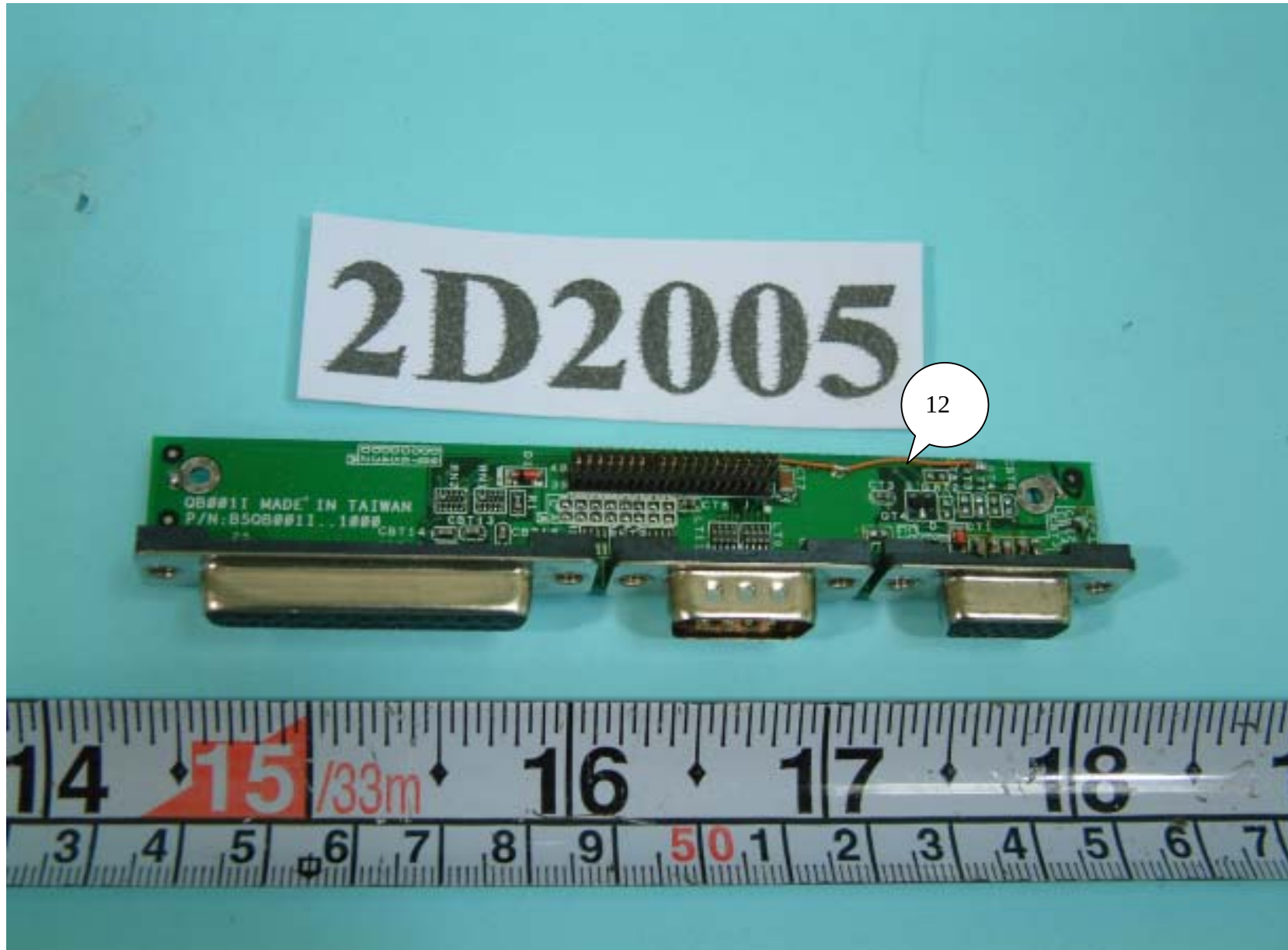
Front side of I/O stick's VGA, COM, PRINTER board
