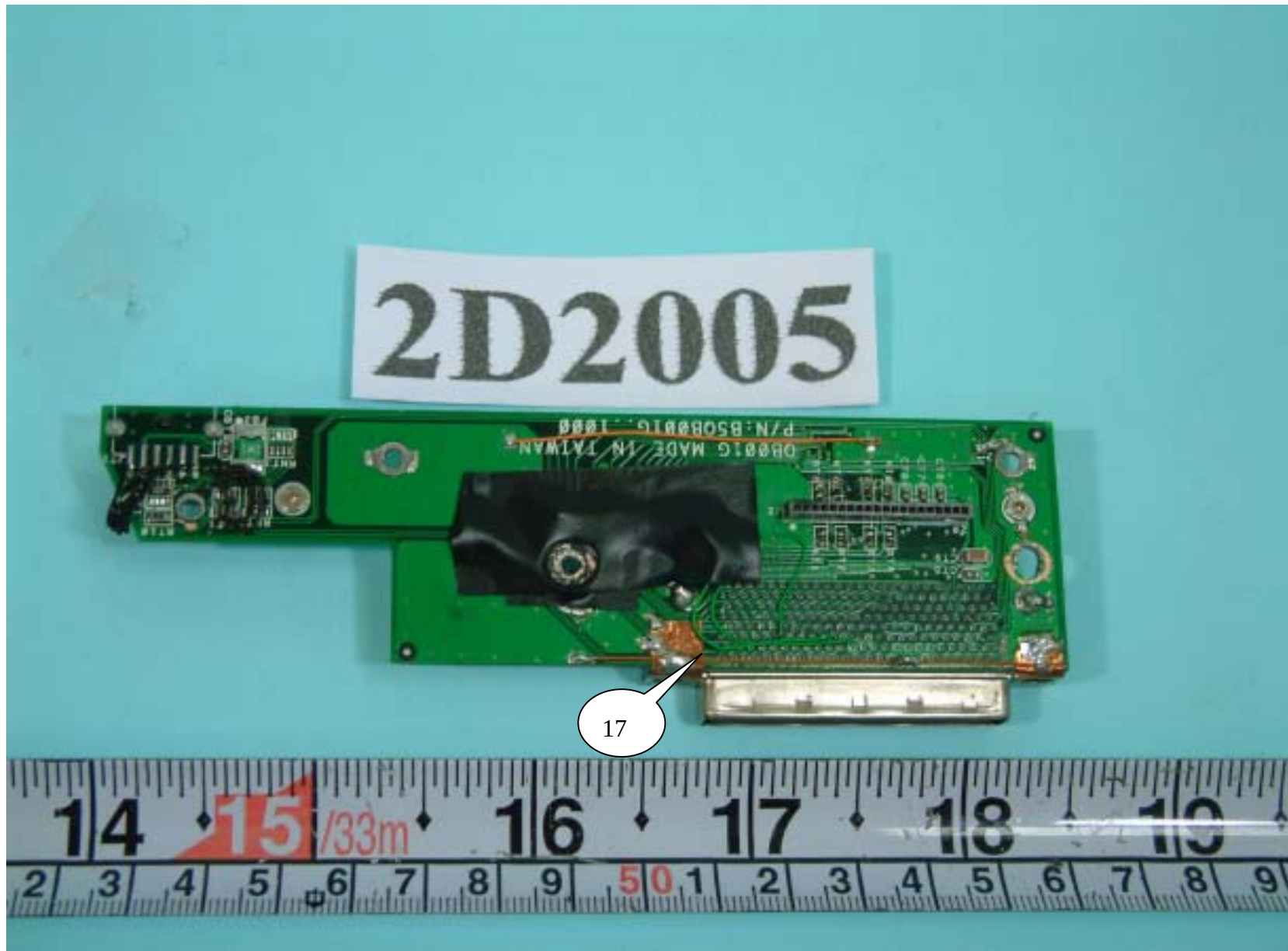
Rear side of I/O stick's PS2 & connect port board
