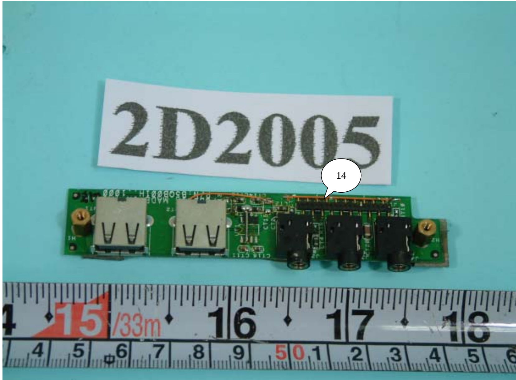
Front side of I/O stick's audio & USB board
