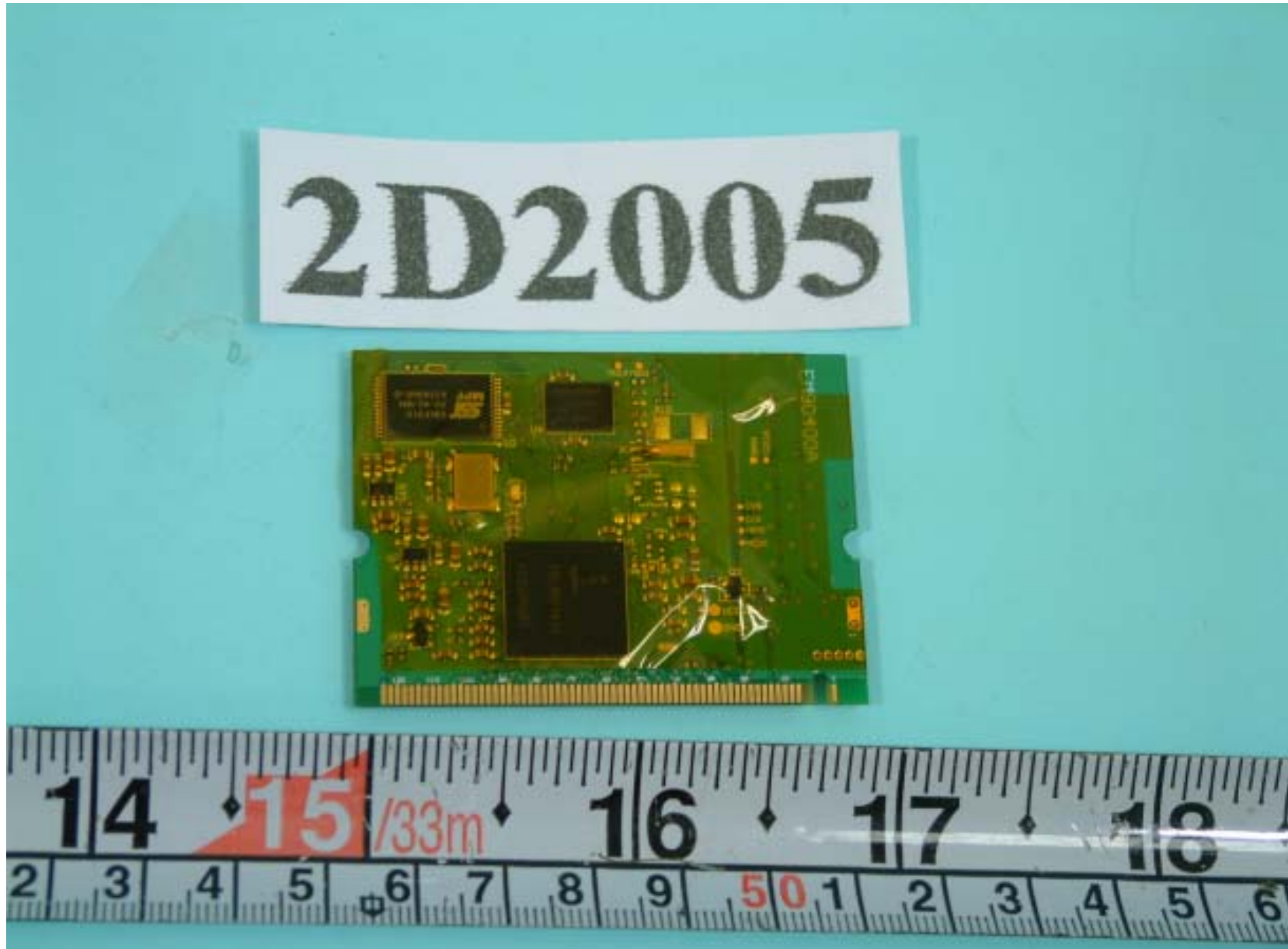
Rear side of IEEE802.11b WLAN module
