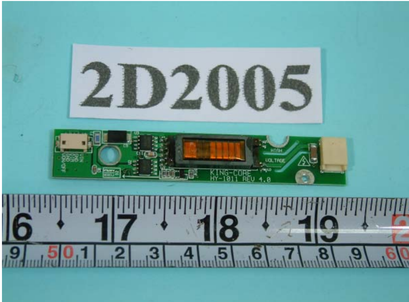
Front side of inverter
