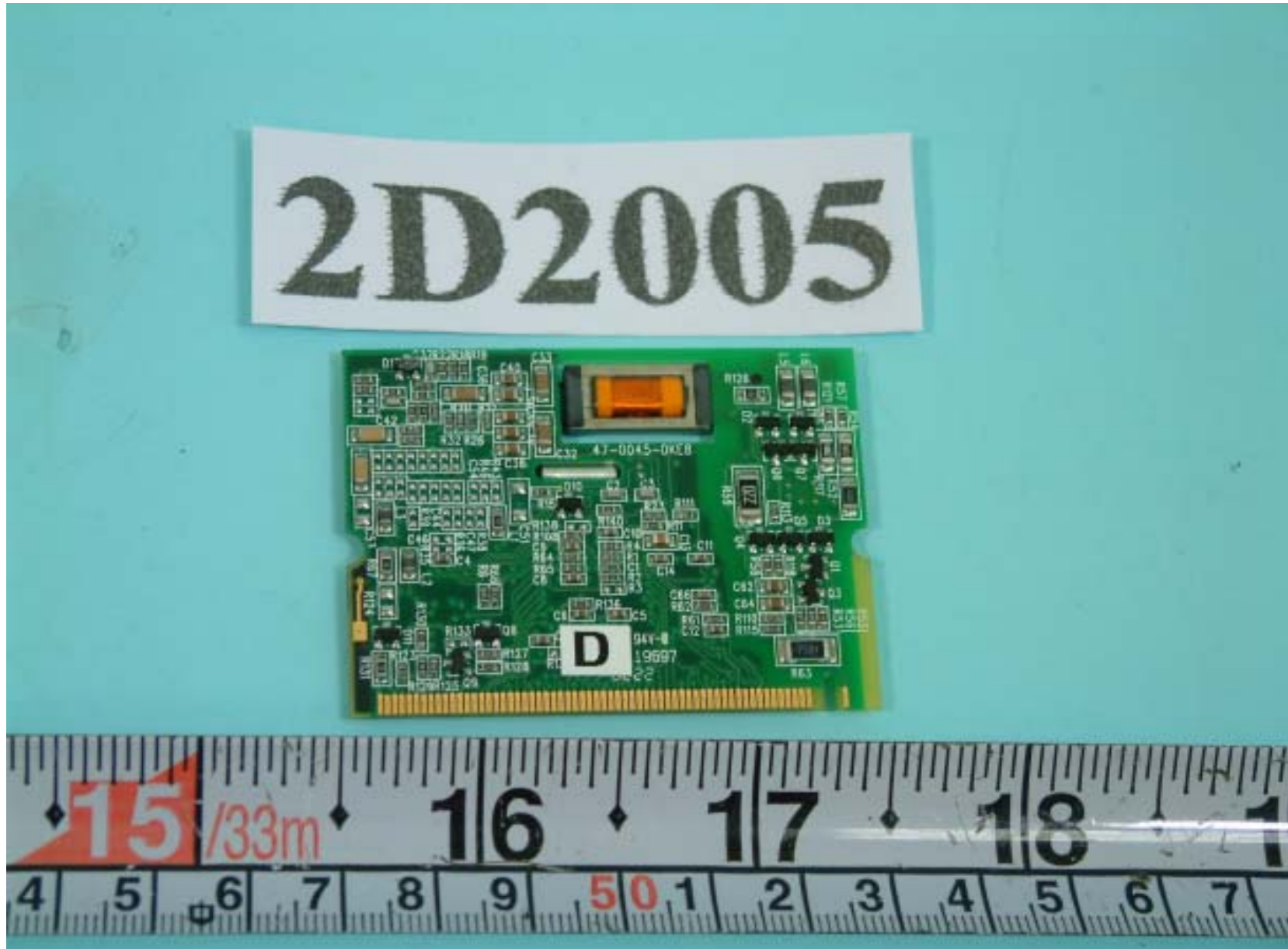
Rear side of BLUETOOTH module
