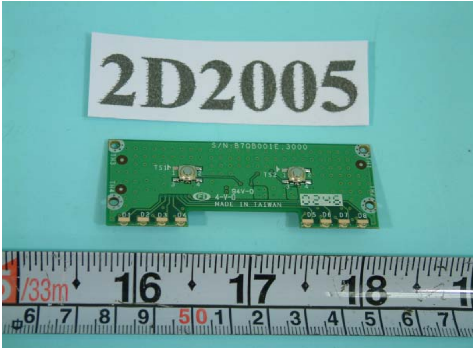
Rear side of touch pad's controlled board
