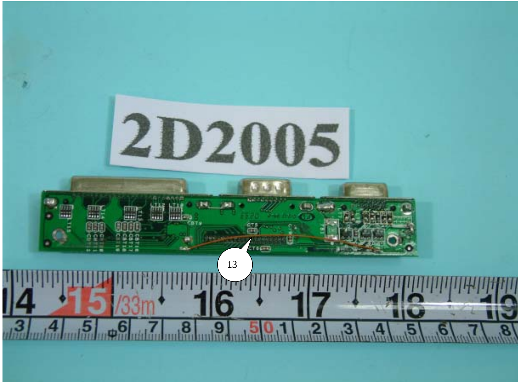
Rear side of I/O stick's VGA, COM, PRINTER board
