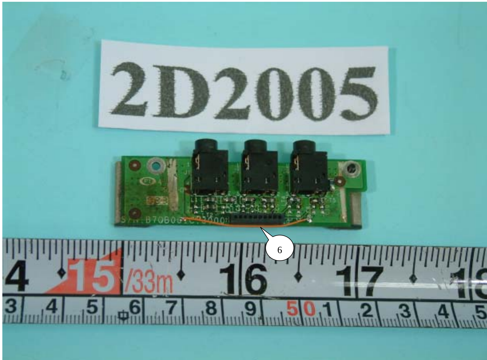
Front side of audio board
