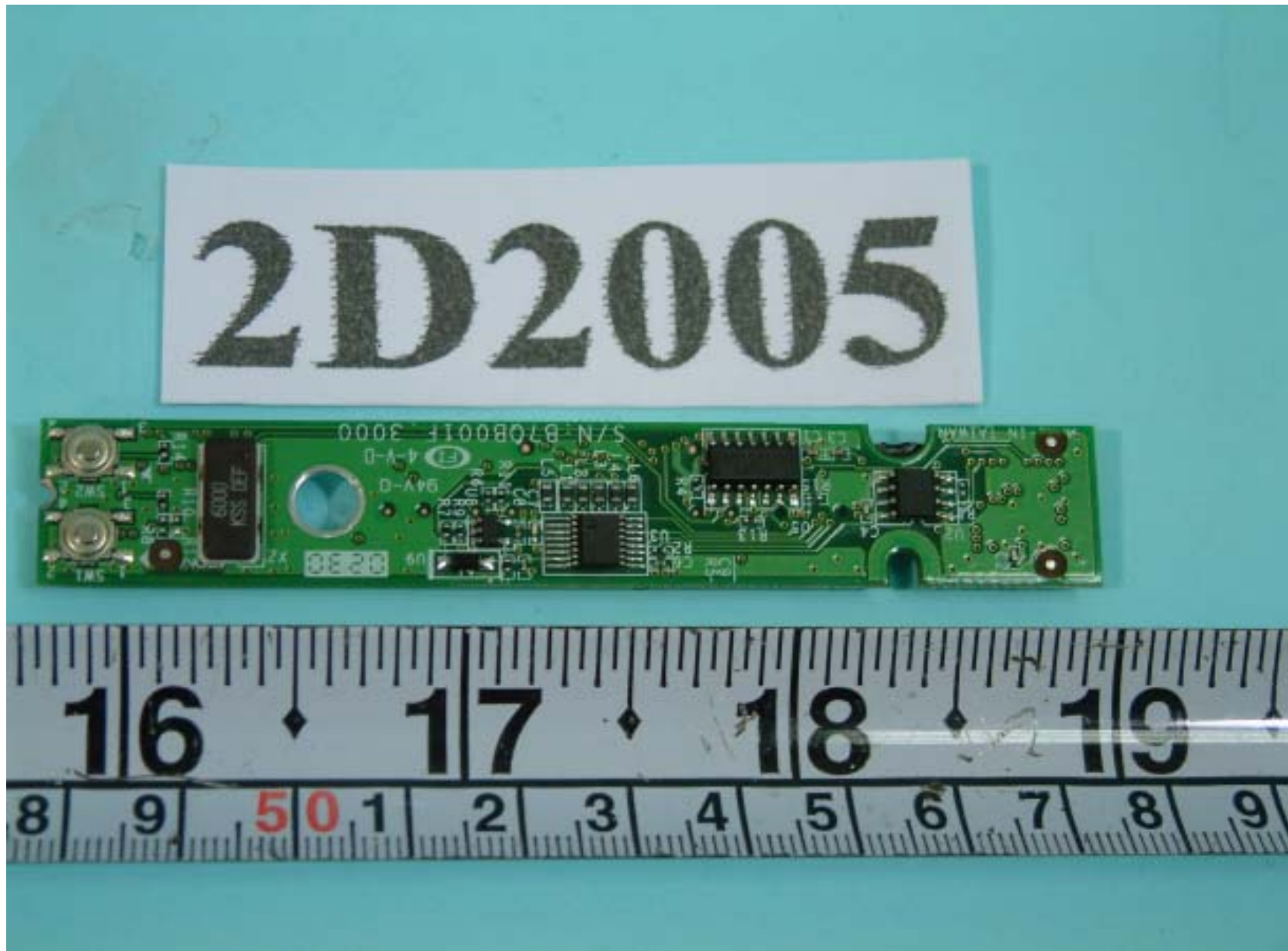
Rear side of panel's control board
