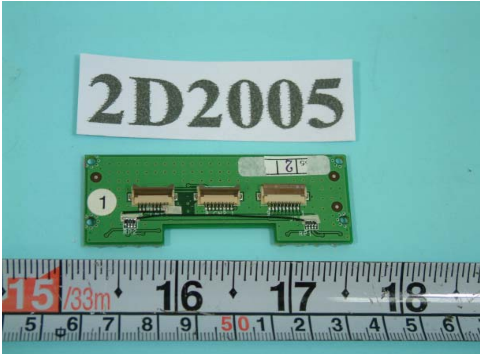
Front side of touch pad's controlled board
