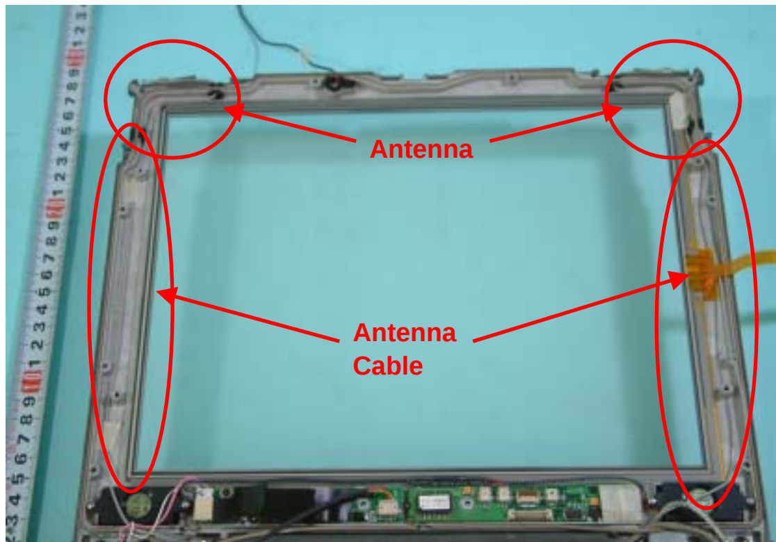
Antenna and antenna cable inside the panel.
