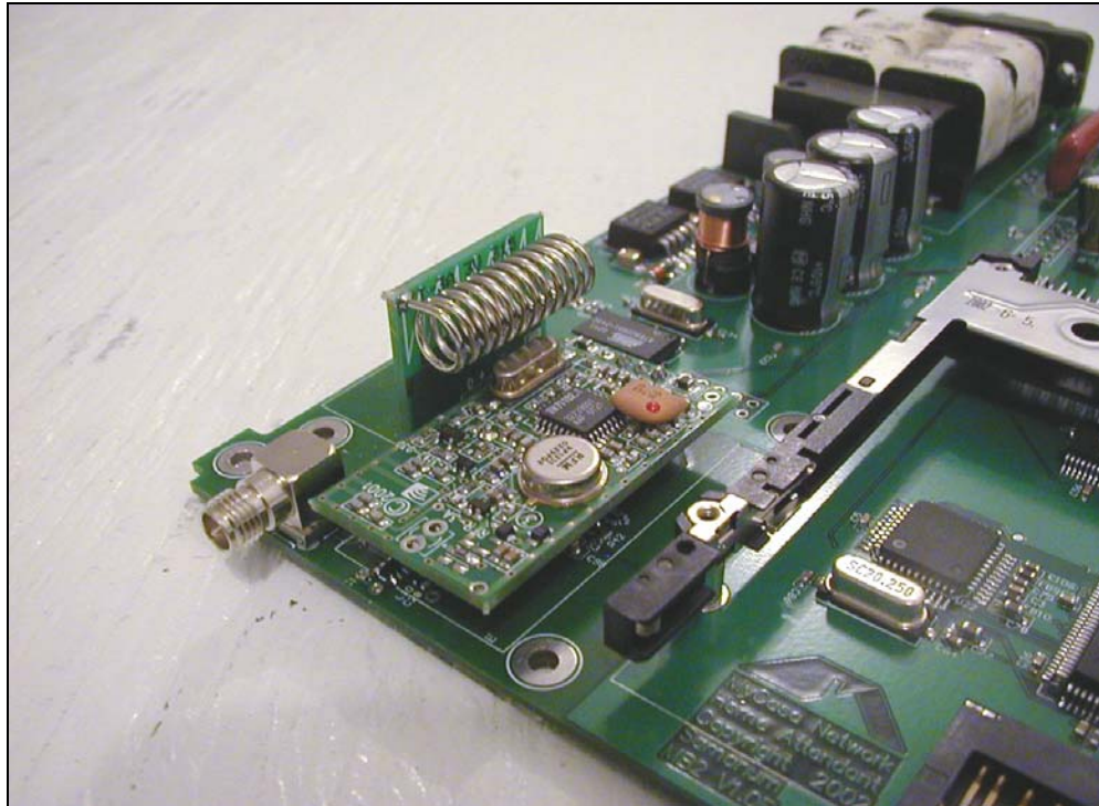
Figure 7: EUT Main Board, showing Transmitter module
