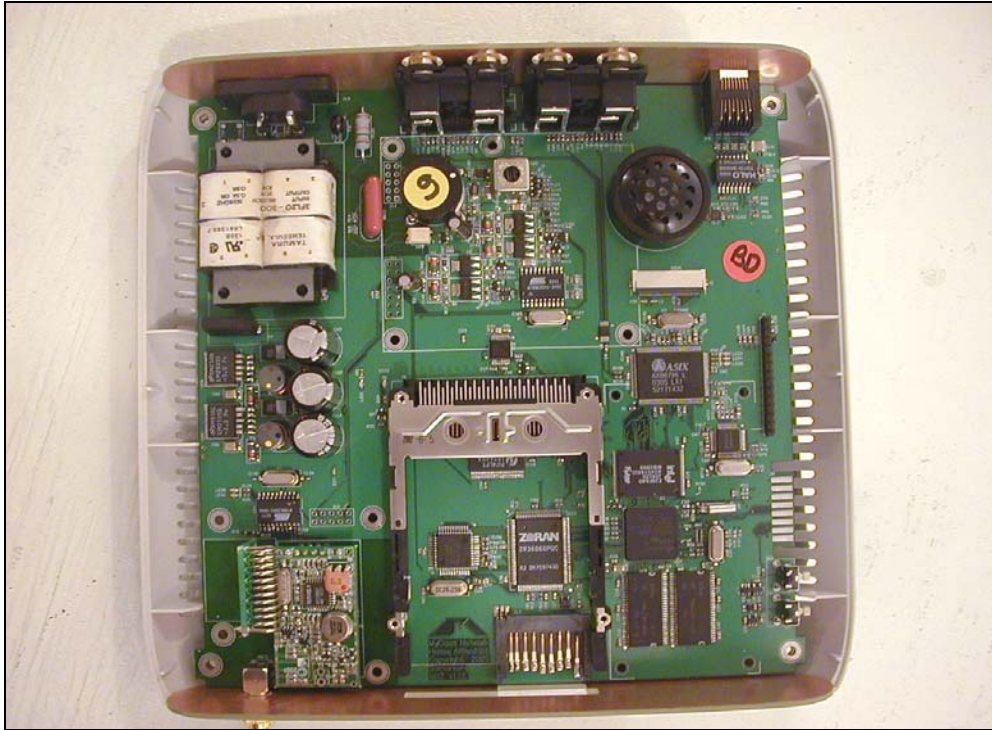
Figure 1: EUT Internal View
