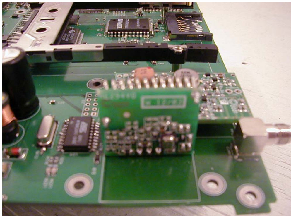
Figure 8: EUT Main Board, showing antenna board
