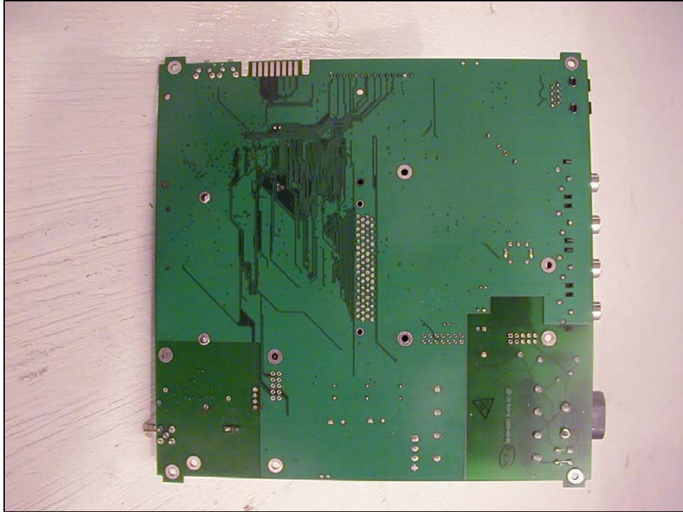
Figure 3: EUT Main Board, solder side view
