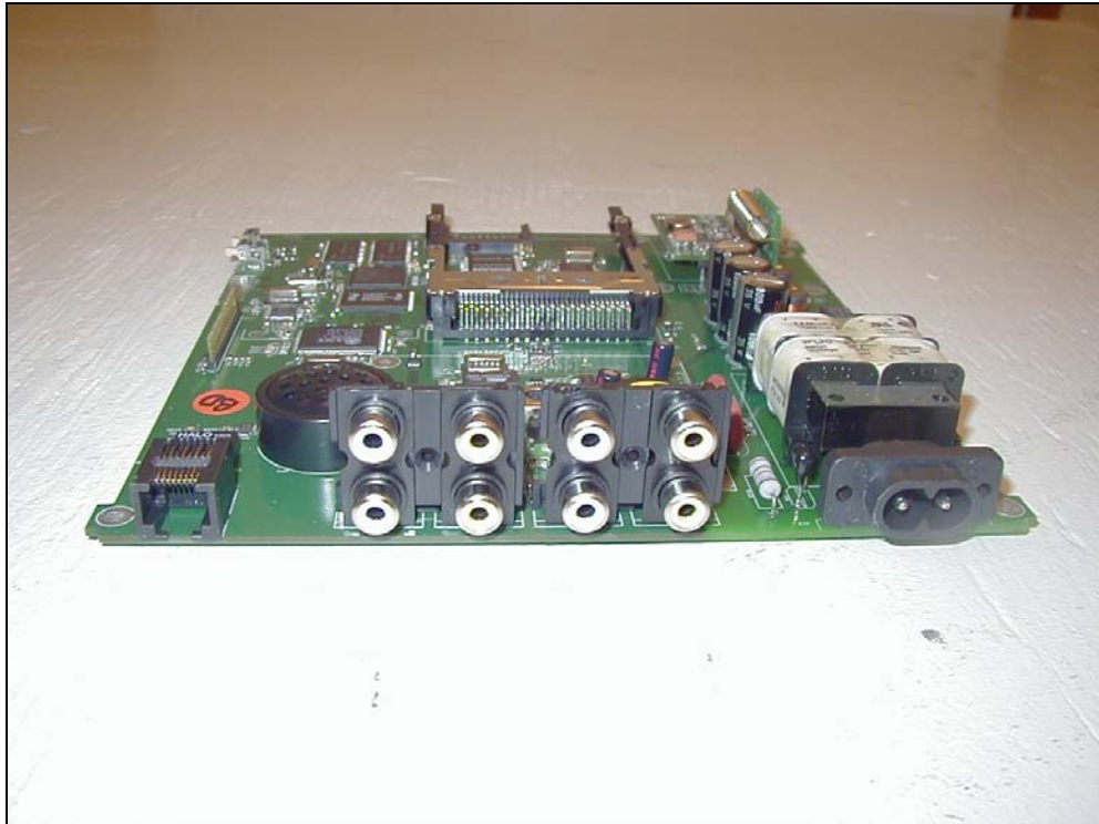
Figure 5: EUT Main Board, connector side view
