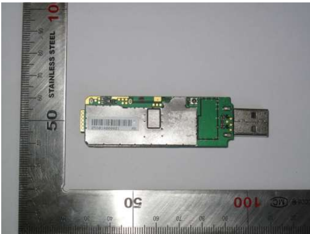
PCB back side with shield
