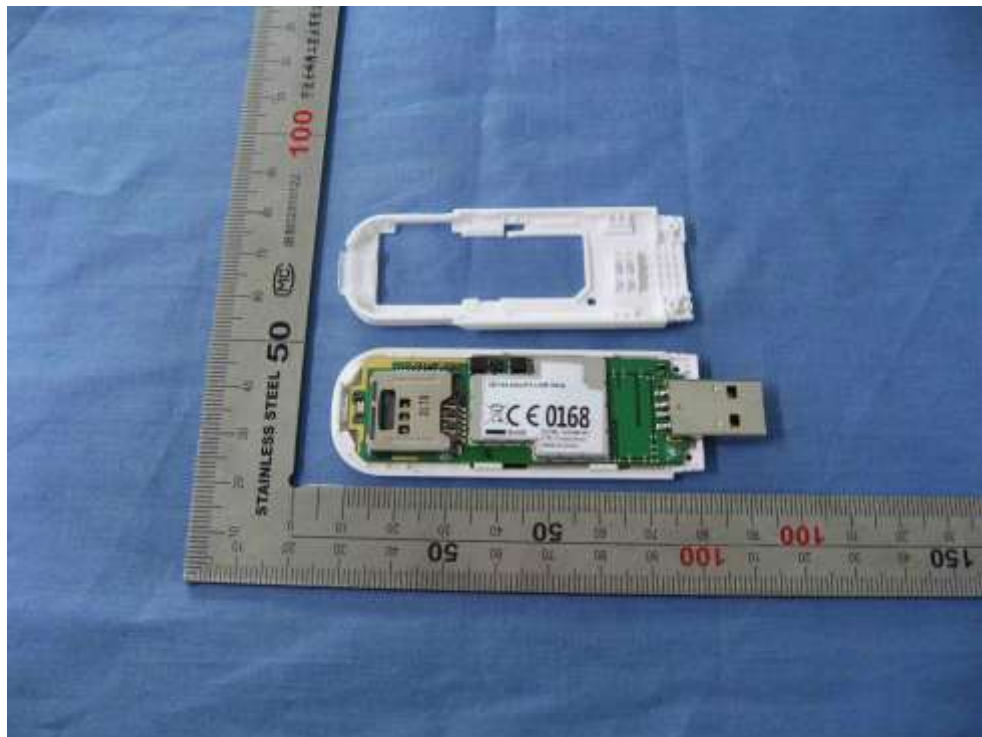
PCB front side with shield
