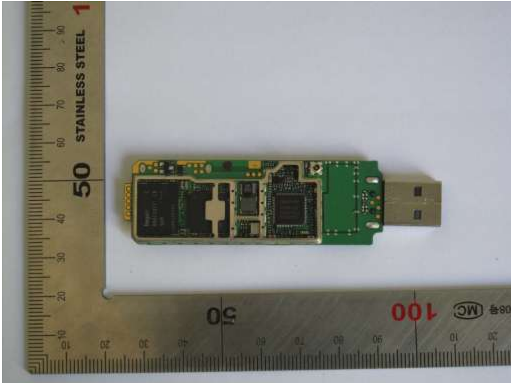
PCB back side without shield
