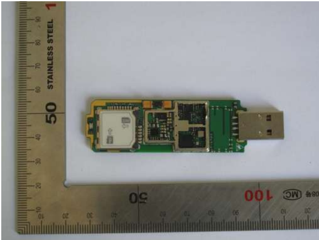
PCB front side without shield
