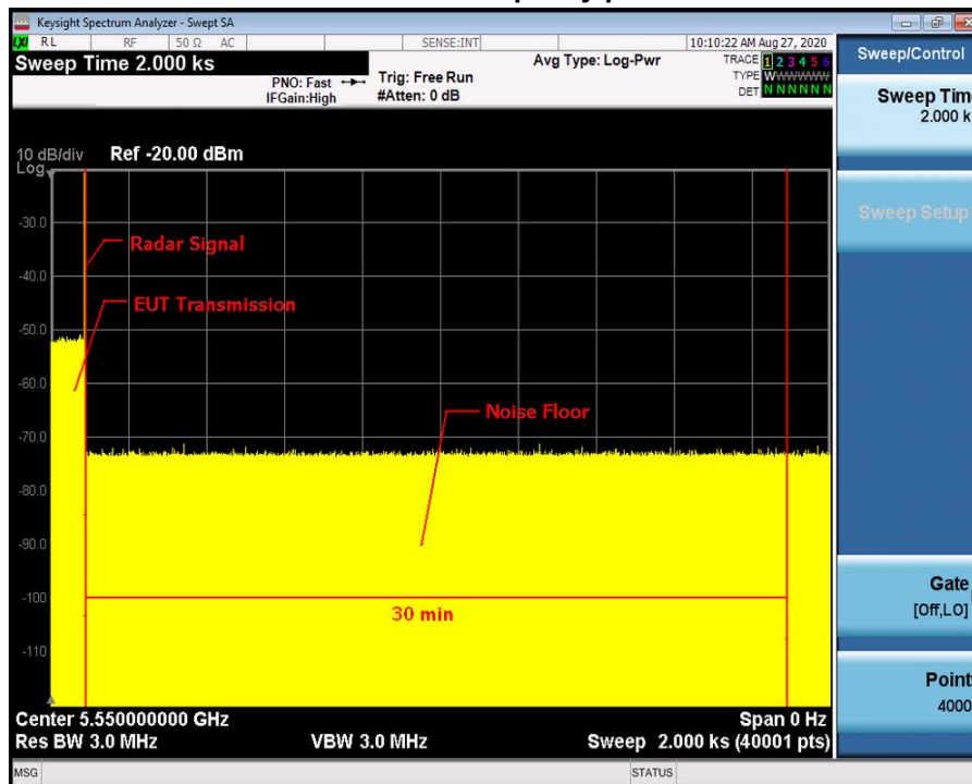
TX (11ac 40MHz Mode) 5550 Non-Occupancy period
