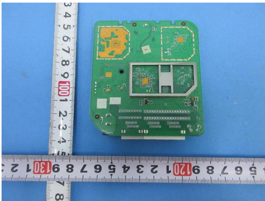
B PCB
