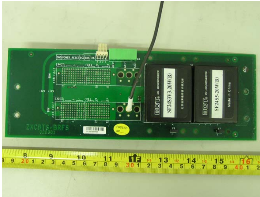
EUT-Power (DC-DC BRFS) PCB Bottom View
