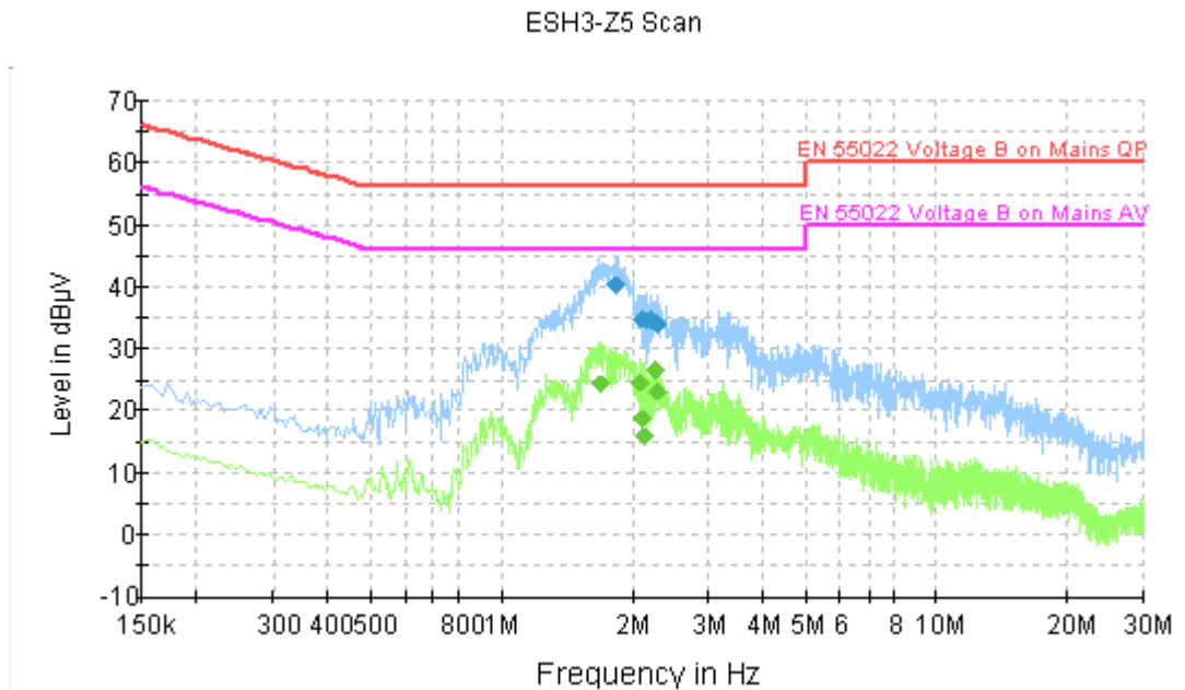
Fig. 77 AC Powerline Conducted Emission-802.11g
