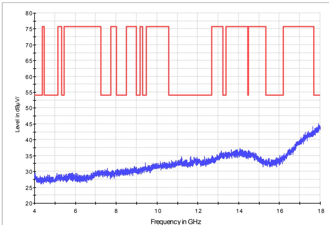
Fig. 46 Radiated Spurious Emission (802.11b, Ch1, 4 GHz-18 GHz)
