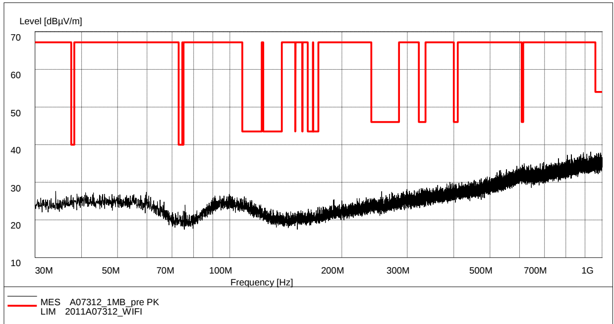
Fig. 101 Radiated Spurious Emission (802.11b, Ch6, 30 MHz-1 GHz)
