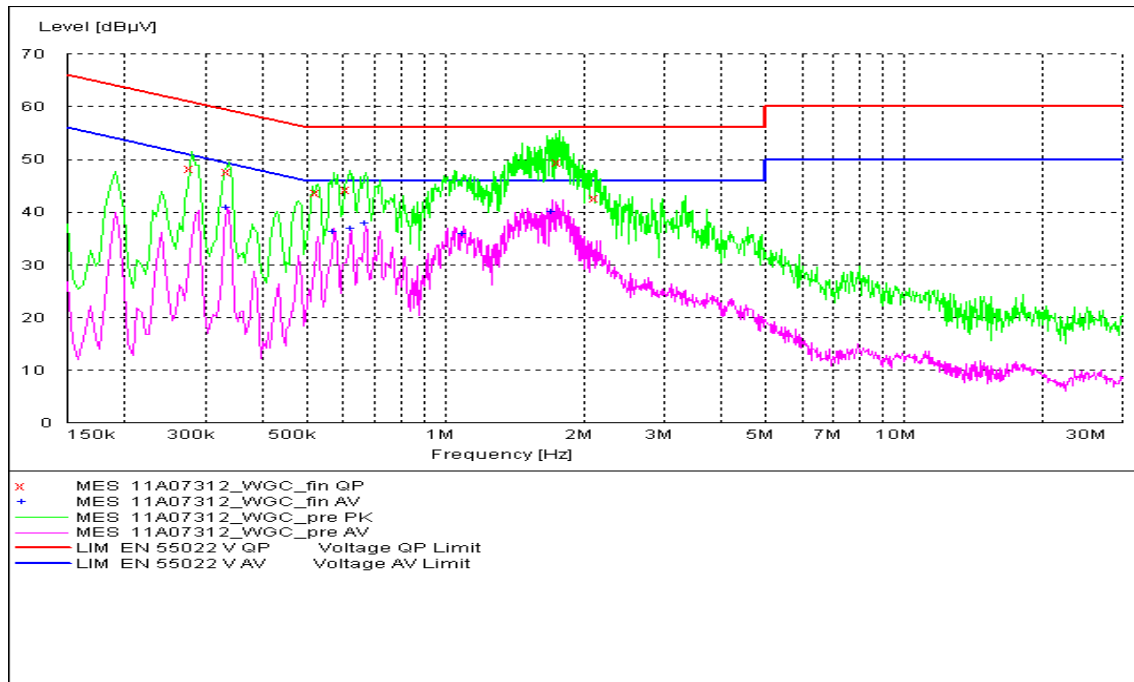
Fig. 133 AC Powerline Conducted Emission-802.11g
