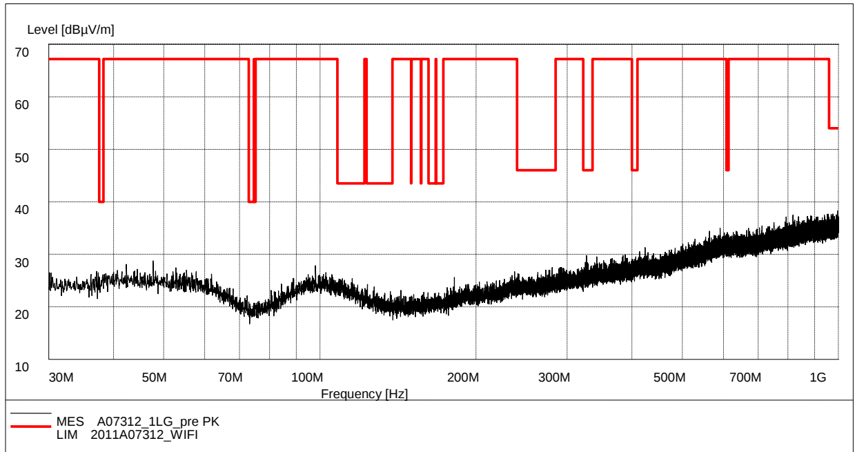
Fig. 109 Radiated Spurious Emission (802.11g, Ch1, 30 MHz-1 GHz)
