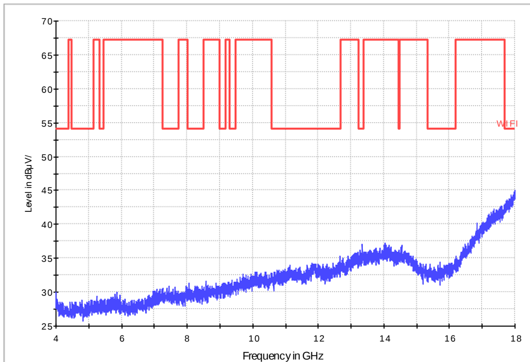
Fig. 114 Radiated Spurious Emission (802.11g, Ch6, 4 GHz-18 GHz)
