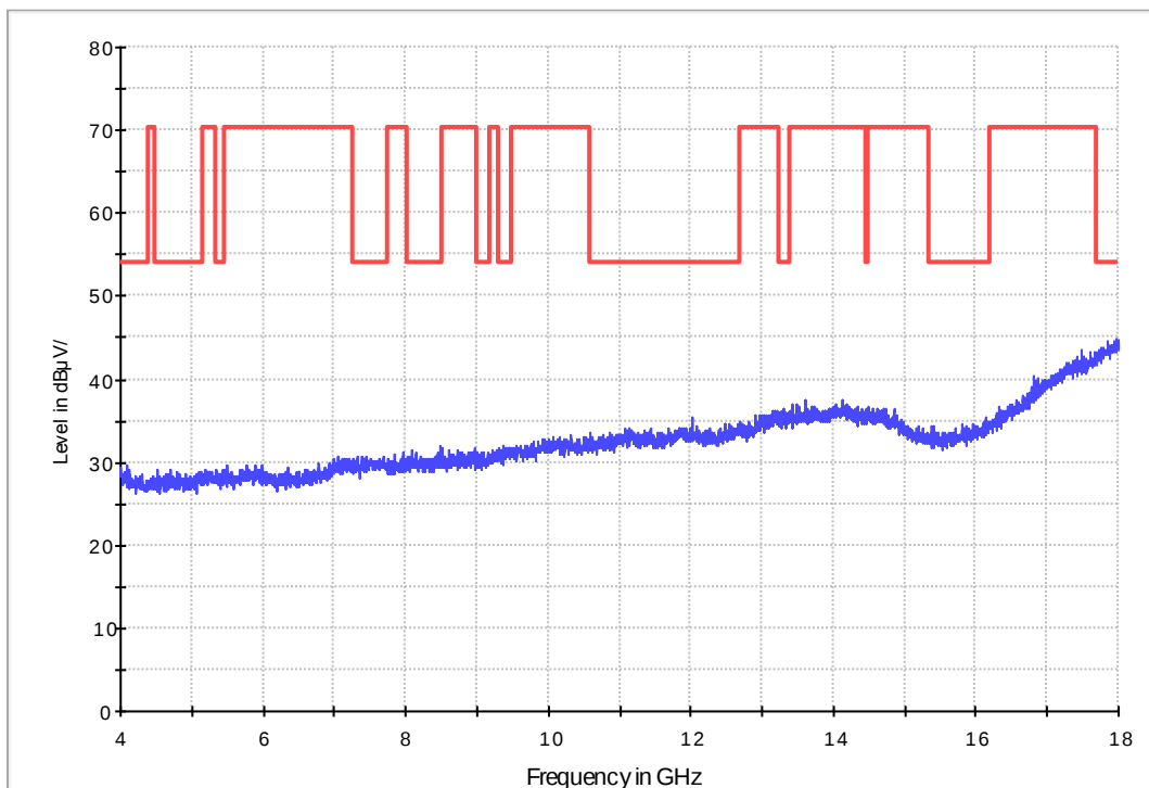
Fig. 130 Radiated Spurious Emission (802.11n-20MHz, Ch11, 4 GHz-18 GHz)
