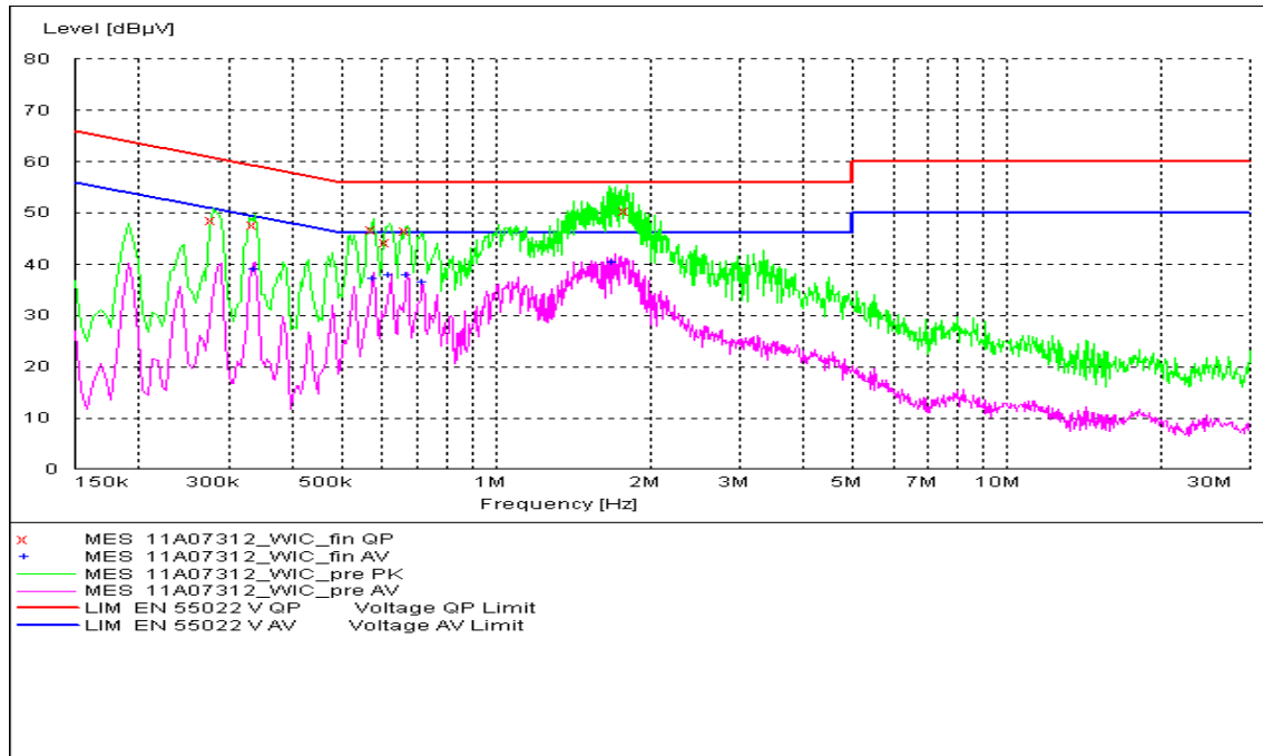
Fig. 134 AC Powerline Conducted Emission-802.11n-20MHz
