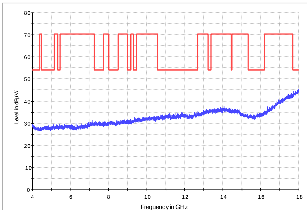
Fig. 126 Radiated Spurious Emission (802.11n-20MHz, Ch6, 4 GHz-18 GHz)
