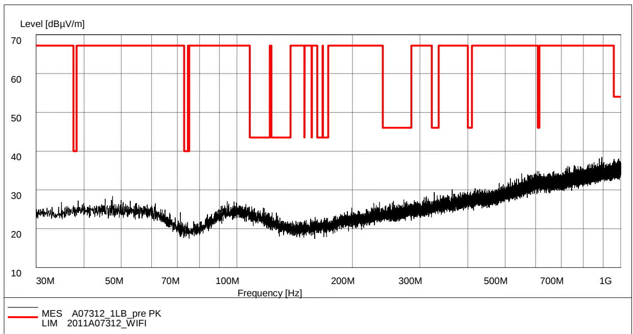
Fig. 98 Radiated Spurious Emission (802.11b, Ch1, 30 MHz-1 GHz)
