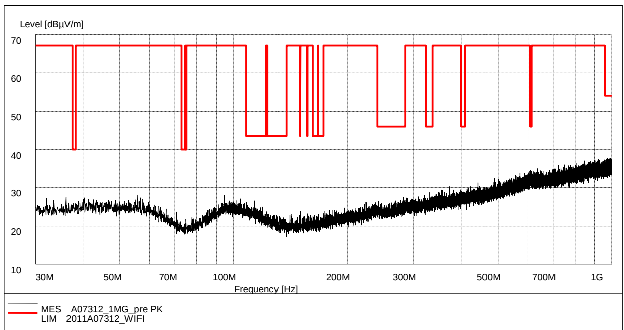
Fig. 112 Radiated Spurious Emission (802.11g, Ch6, 30 MHz-1 GHz)
