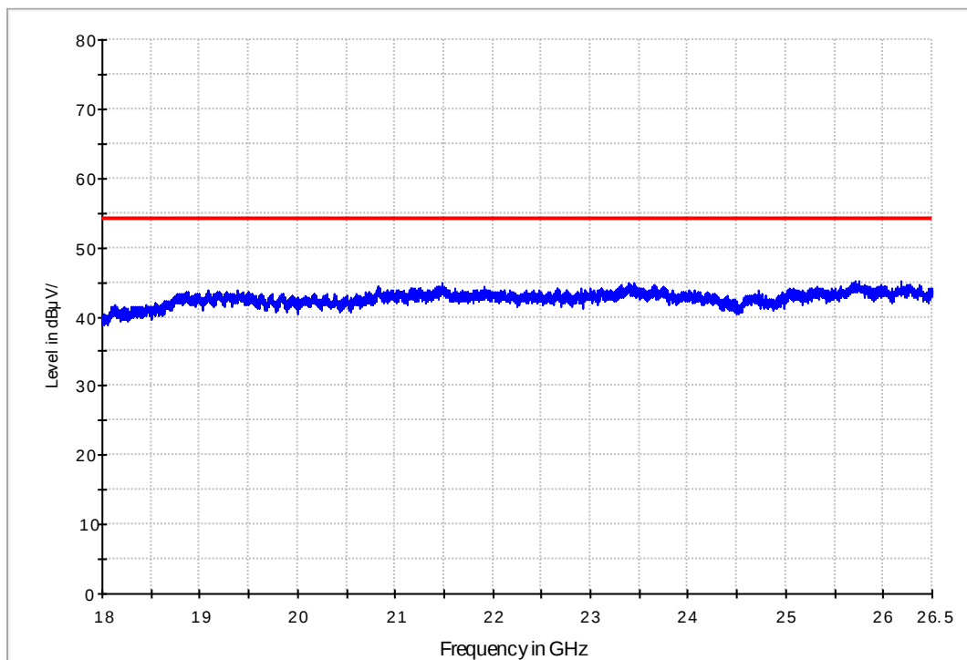
Fig. 131 Radiated emission: 18 GHz - 26.5 GHz
