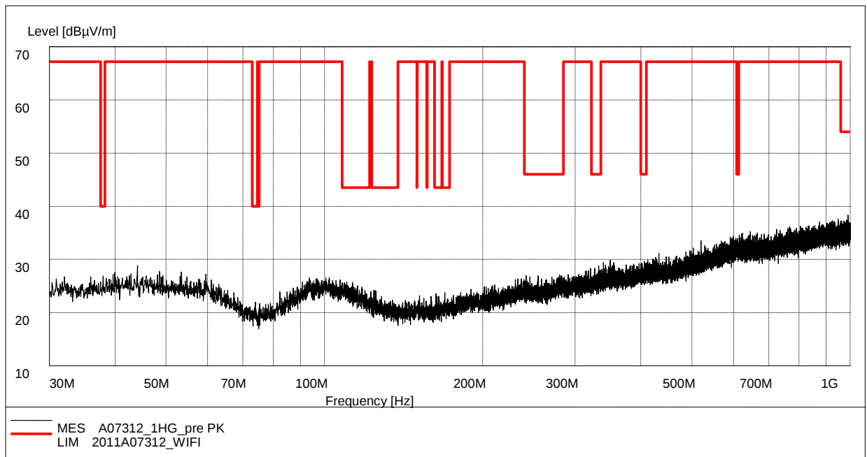
Fig. 116 Radiated Spurious Emission (802.11g, Ch11, 30 MHz-1 GHz)
