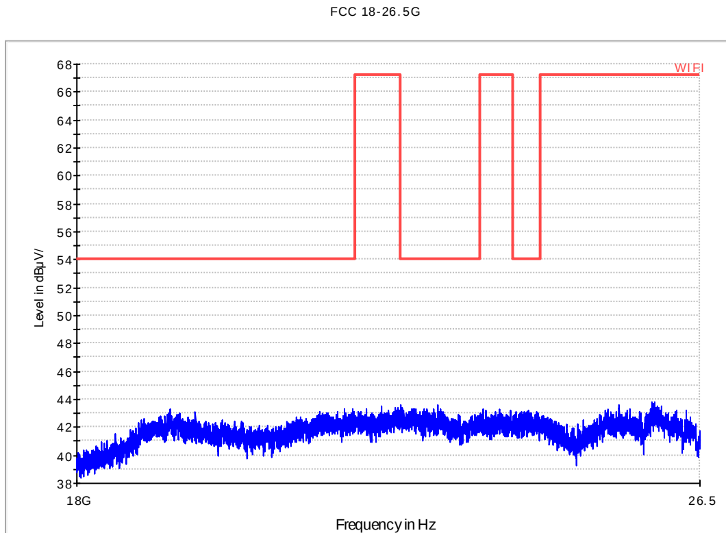
Fig. 119 Radiated emission: 18 GHz - 26.5 GHz
