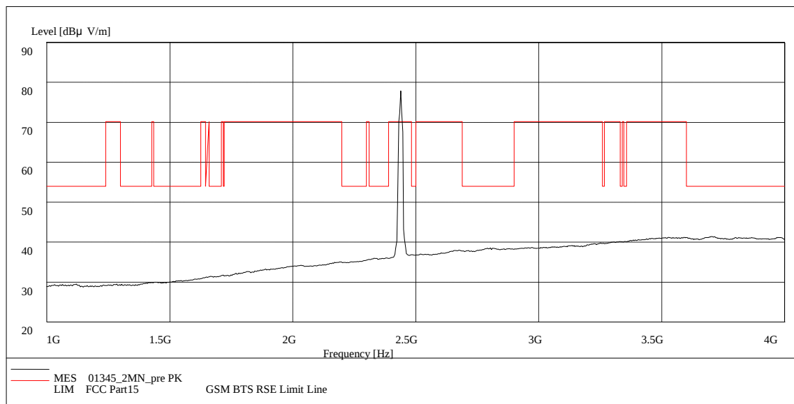
Fig. 125 Radiated Spurious Emission (802.11n-20MHz, Ch6, 1 GHz-4 GHz)
