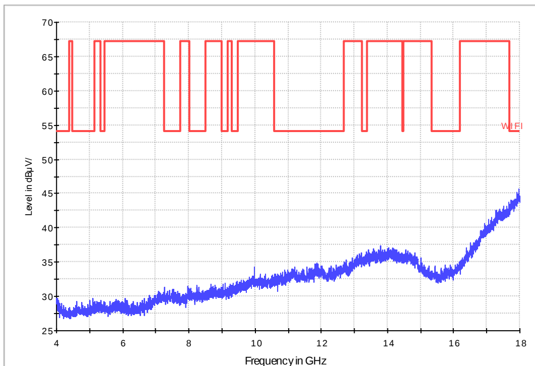
Fig. 100 Radiated Spurious Emission (802.11b, Ch1, 4 GHz-18 GHz)
