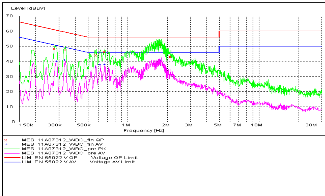
Fig. 132 AC Powerline Conducted Emission-802.11b
