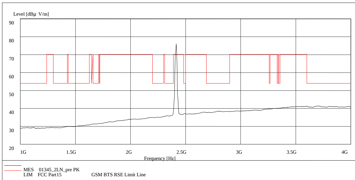
Fig. 122 Radiated Spurious Emission (802.11n-20MHz, Ch1, 1 GHz-4 GHz)
