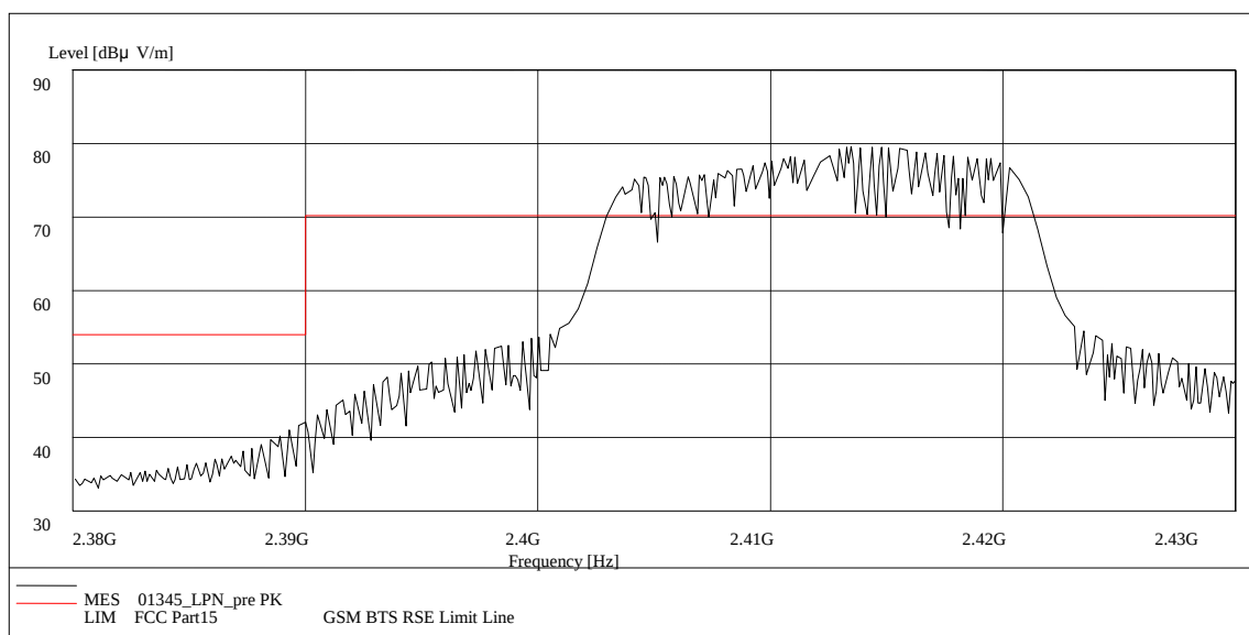
Fig. 120 Radiated Spurious Emission (Power): 802.11n-20MHz, ch1, 2.38 GHz - 2.43GHz
