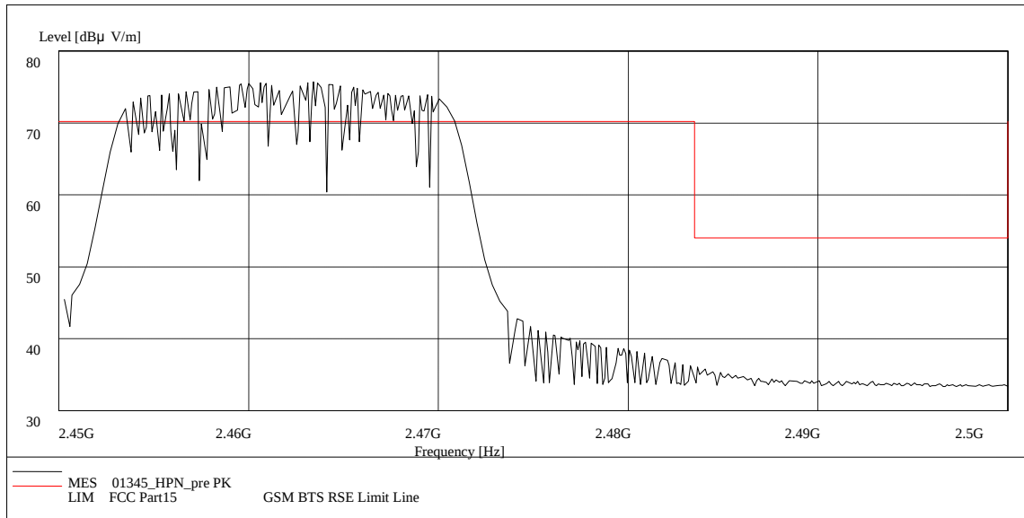
Fig. 127 Radiated Spurious Emission (Power): 802.11n-20MHz, ch11, 2.45 GHz - 2.50GHz
