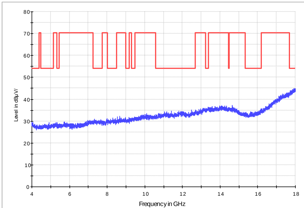
Fig. 123 Radiated Spurious Emission (802.11n-20MHz, Ch1, 4 GHz-18 GHz)
