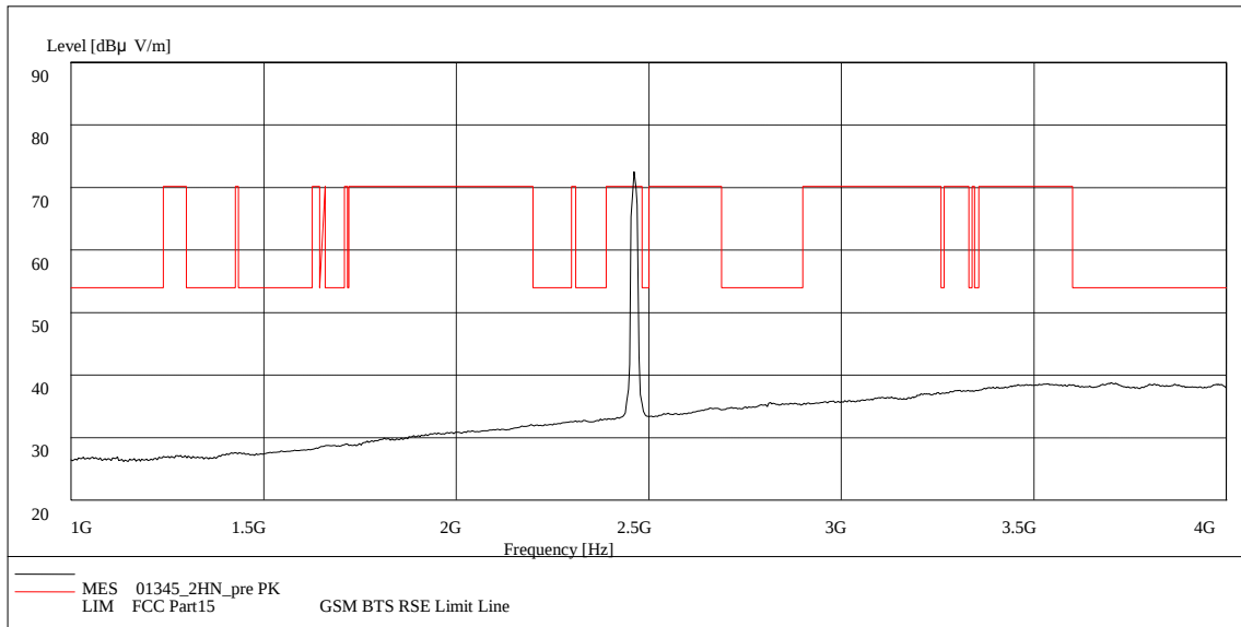
Fig. 129 Radiated Spurious Emission (802.11n-20MHz, Ch11, 1 GHz-4 GHz)
