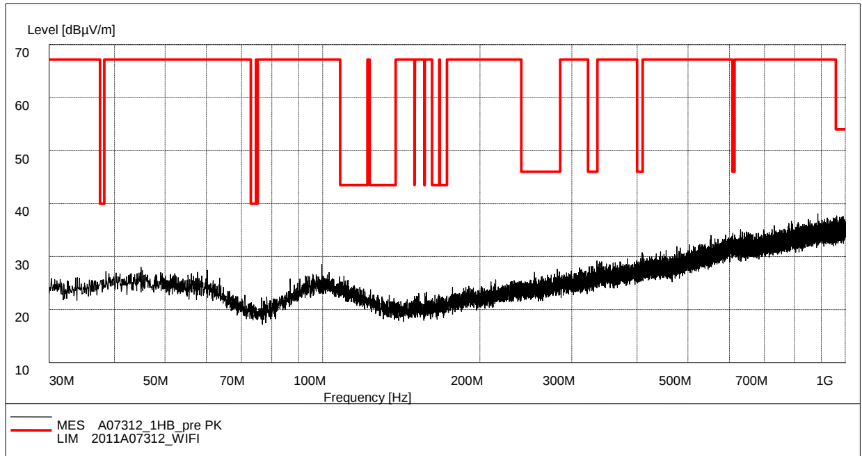
Fig. 105 Radiated Spurious Emission (802.11b, Ch11, 30 MHz-1 GHz)
