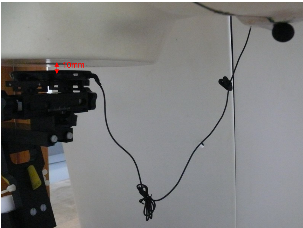
Picture 20: Front Side with earphone, the distance from handset to the bottom of the Phantom is 10mm
