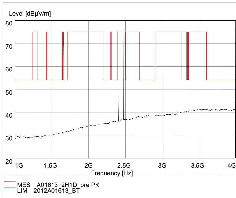
Fig.65. Radiated emission: GFSK, Channel 78, 1 GHz - 4 GHz
