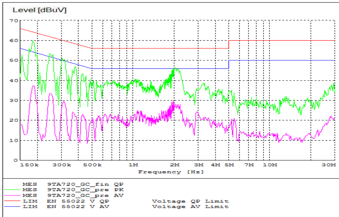
Figure A.5 Conducted Emission
