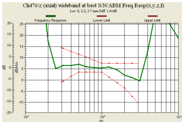
Fig. 8.7 CDMA2000 BC10 Ch476
