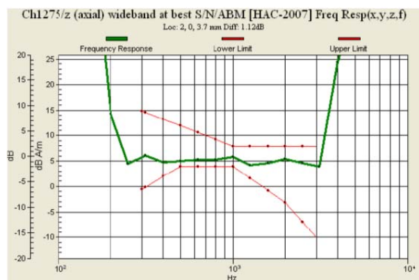
Fig. 9.3 CDMA2000 BC14 Ch1275
