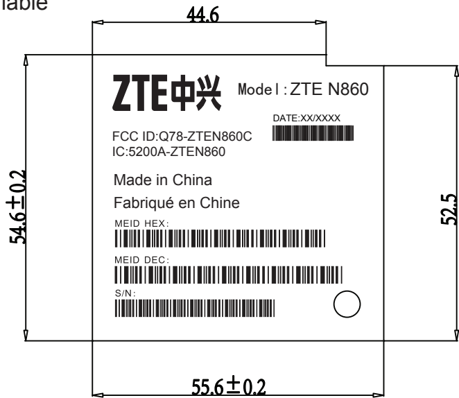
Device lable
