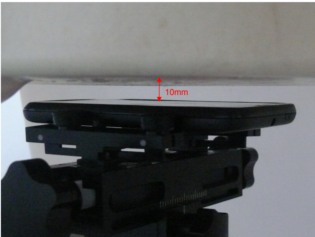
Picture 14: Body, the EUT display towards phantom, the distance from handset to the bottom of the Phantom is 10mm
