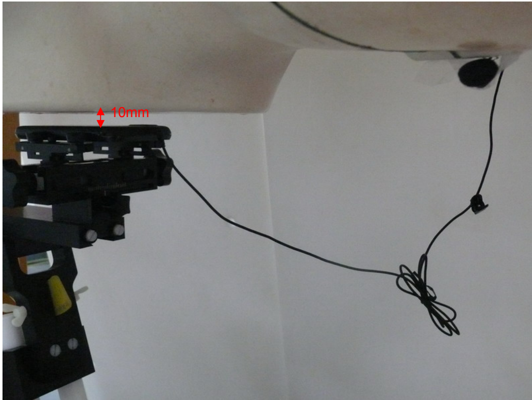
Picture 19: Body with Earphone, The EUT display towards ground, the distance from handset to the bottom of the Phantom is 10mm
