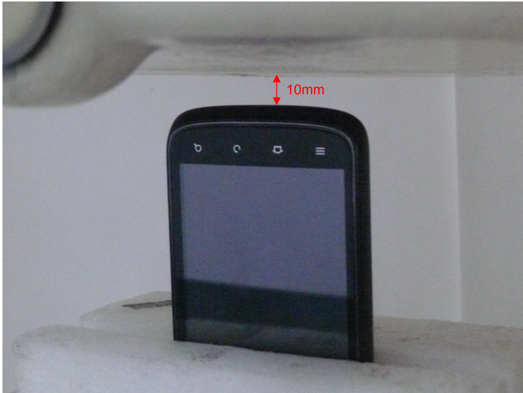
Picture 17: bottom edge, the distance from handset to the bottom of the Phantom is 10mm
