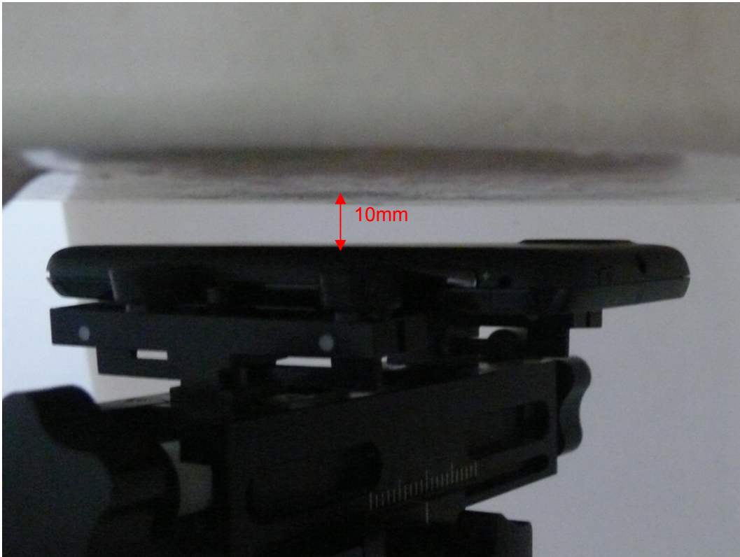
Picture 13: Body, the EUT display towards ground, the distance from handset to the bottom of the Phantom is 10mm
