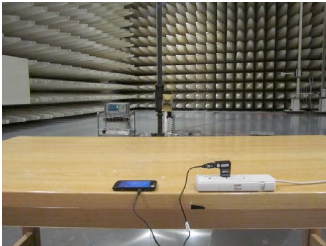
2011A04613_RE_15B_Charging
