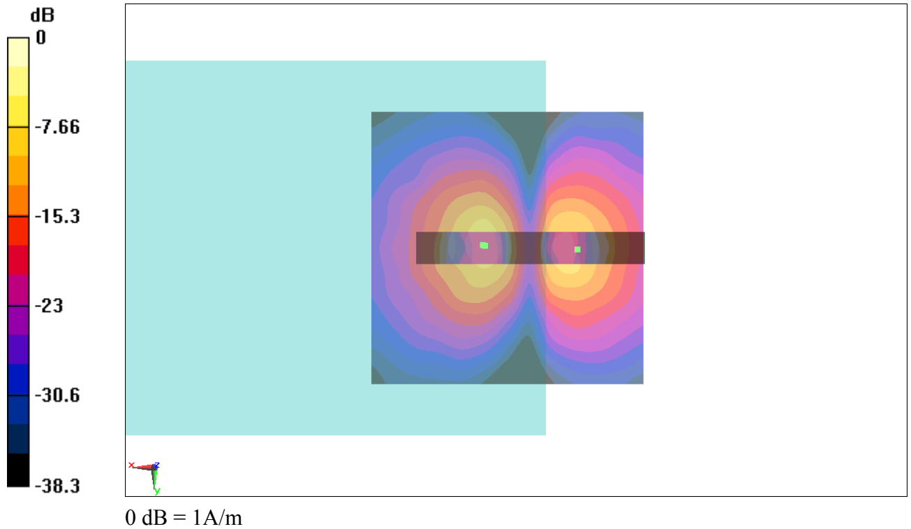
Fig B.1 T-Coil CDMA 835_Channel 777
