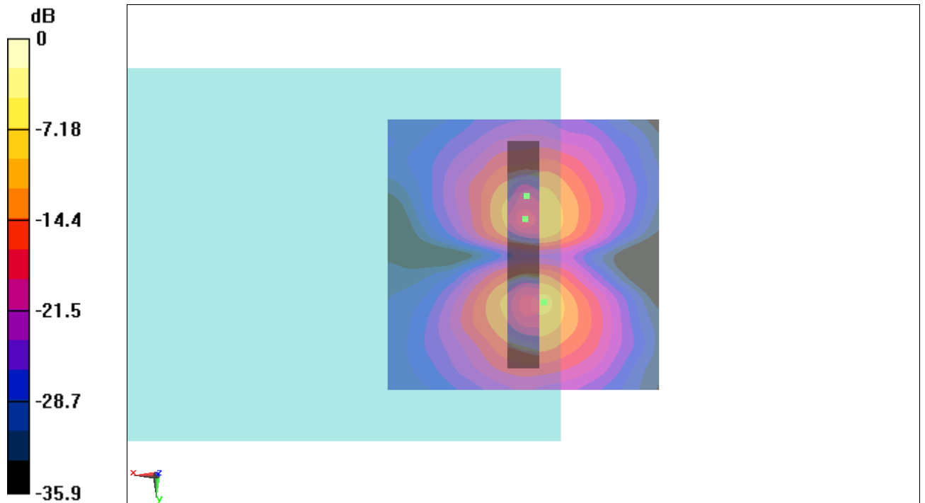
Fig B.11 T-Coil CDMA 1880_Channel 1175
