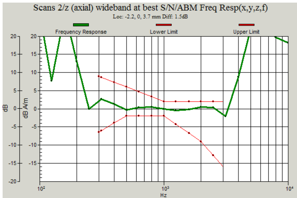
Figure C.2 Frequency Response of CDMA 835_Channel 384
