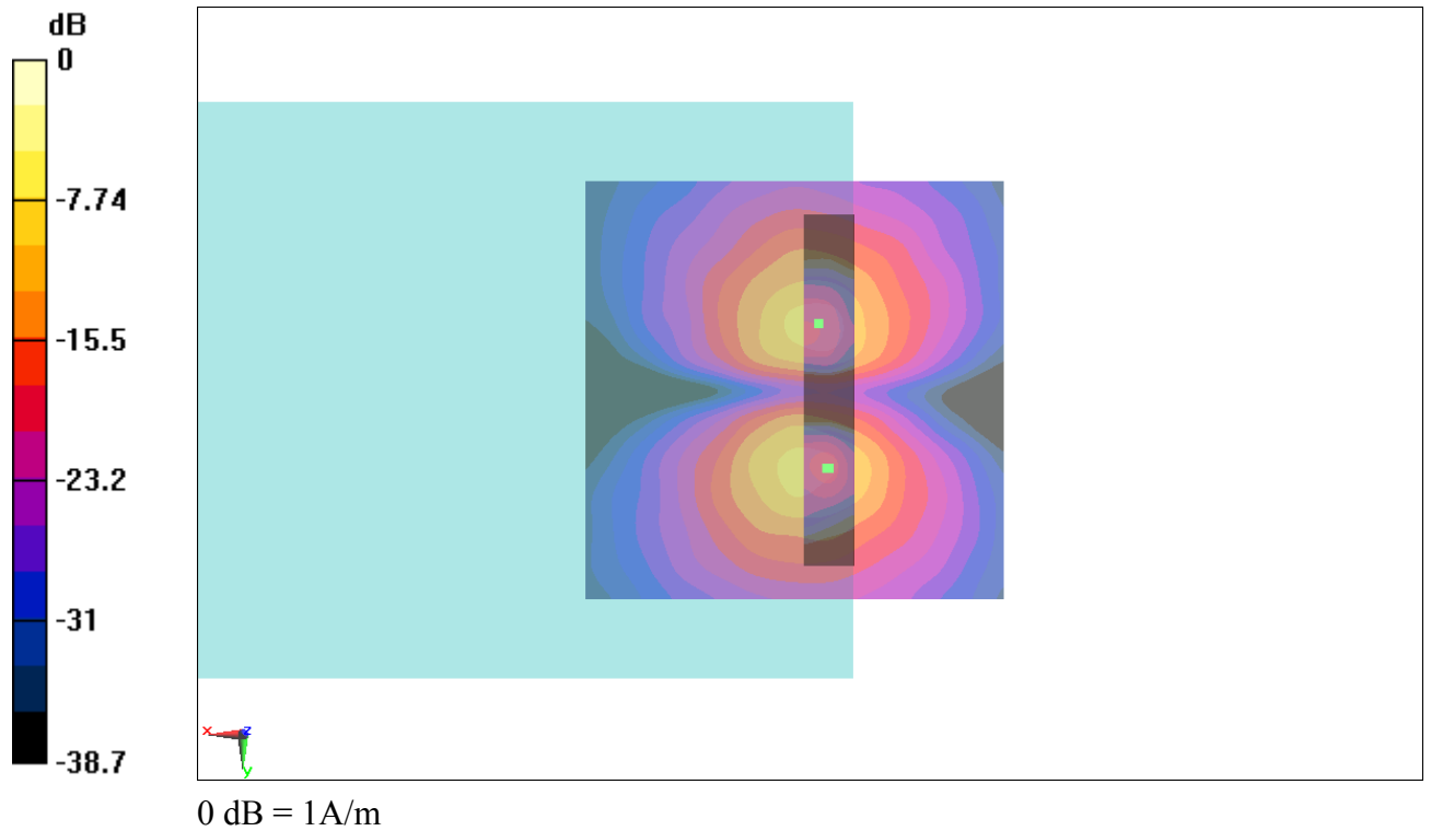
Fig B.2 T-Coil CDMA 835_Channel 777
