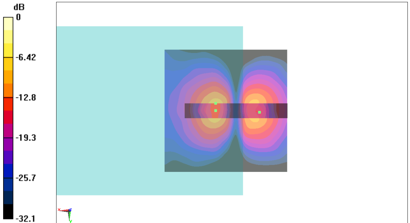
Fig B.16 T-Coil CDMA 1880_Channel 25
