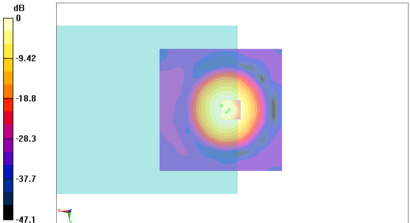
Fig B.18 T-Coil CDMA 1880_Channel 25
