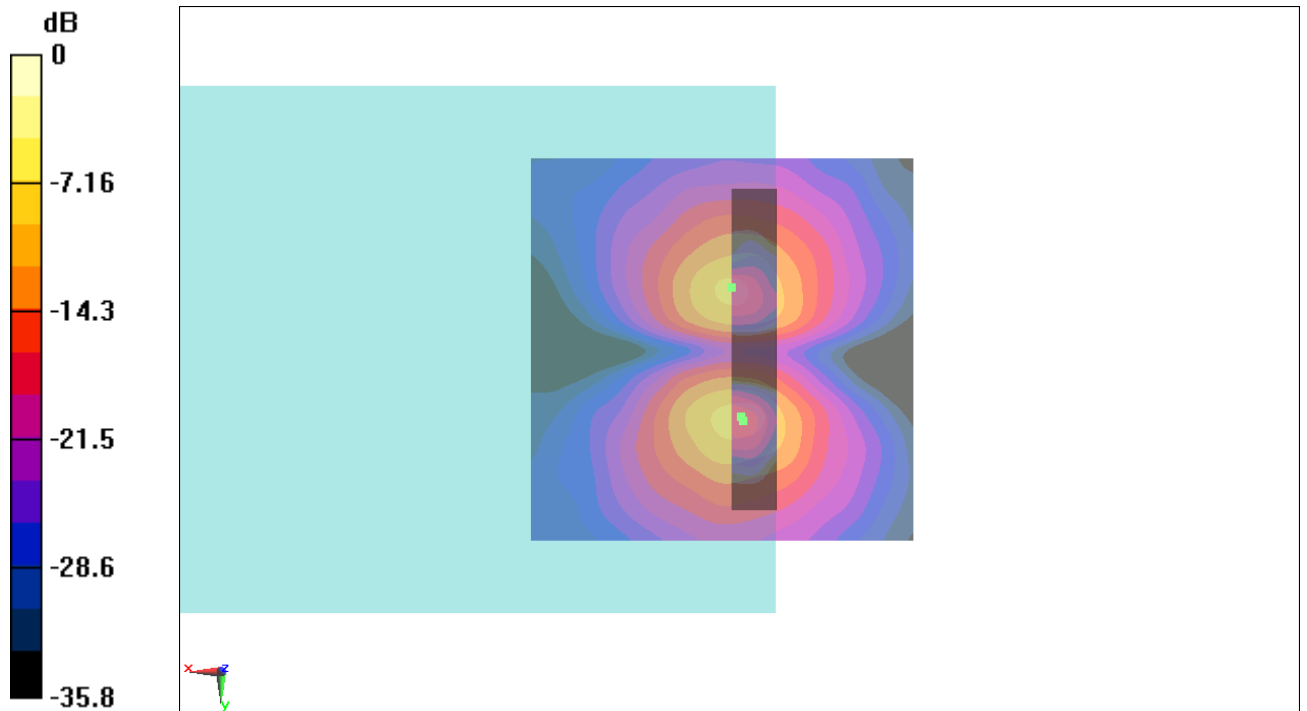
Fig B.8 T-Coil CDMA 835_Channel 1013
