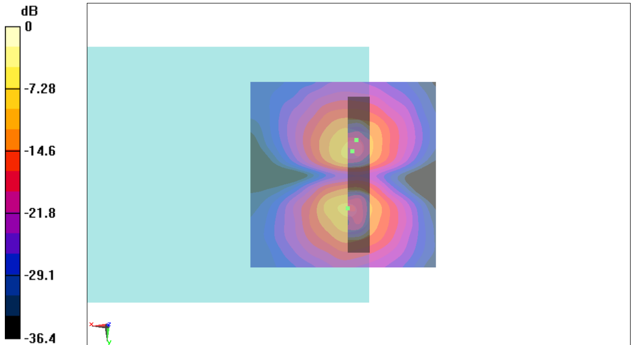
Fig B.14 T-Coil CDMA 1880_Channel 600
