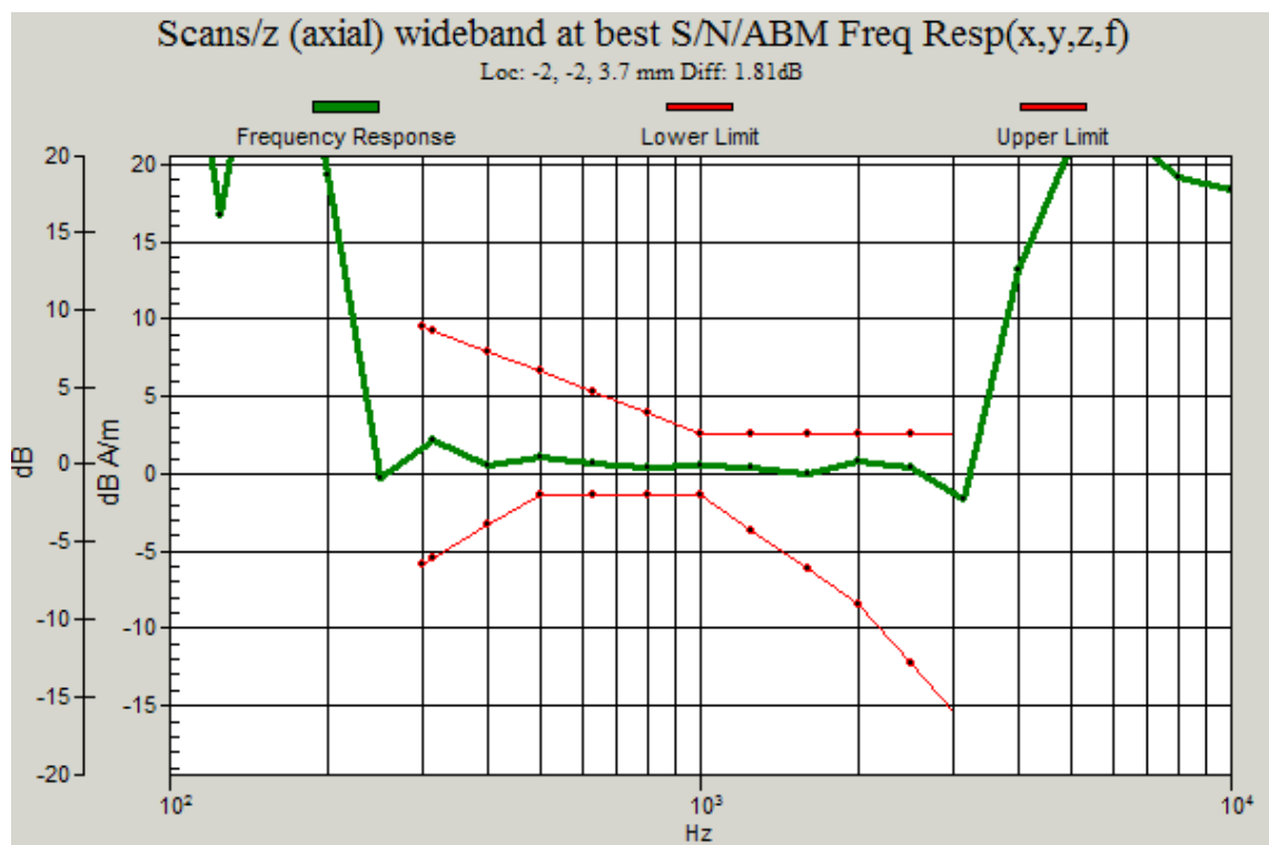
Figure C.4 Frequency Response of CDMA 1880_Channel 1175
