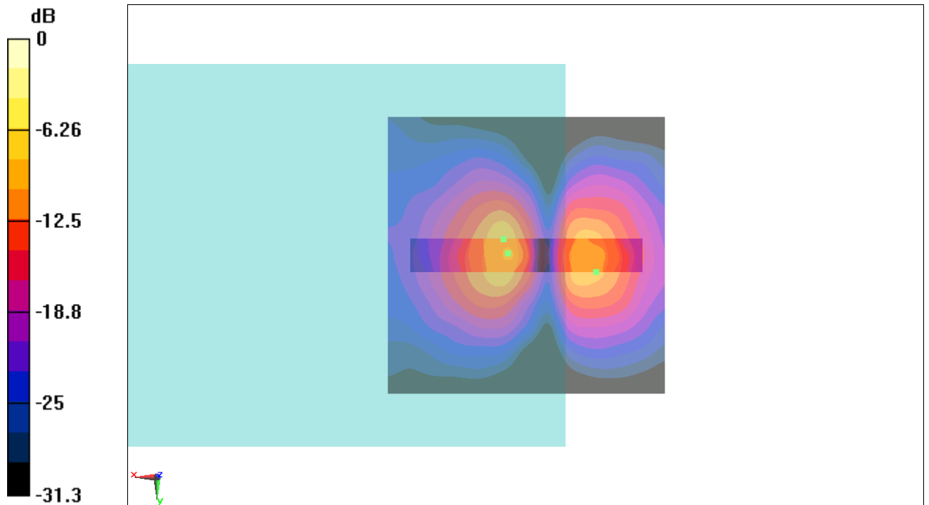
Fig B.10 T-Coil CDMA 1880_Channel 1175
