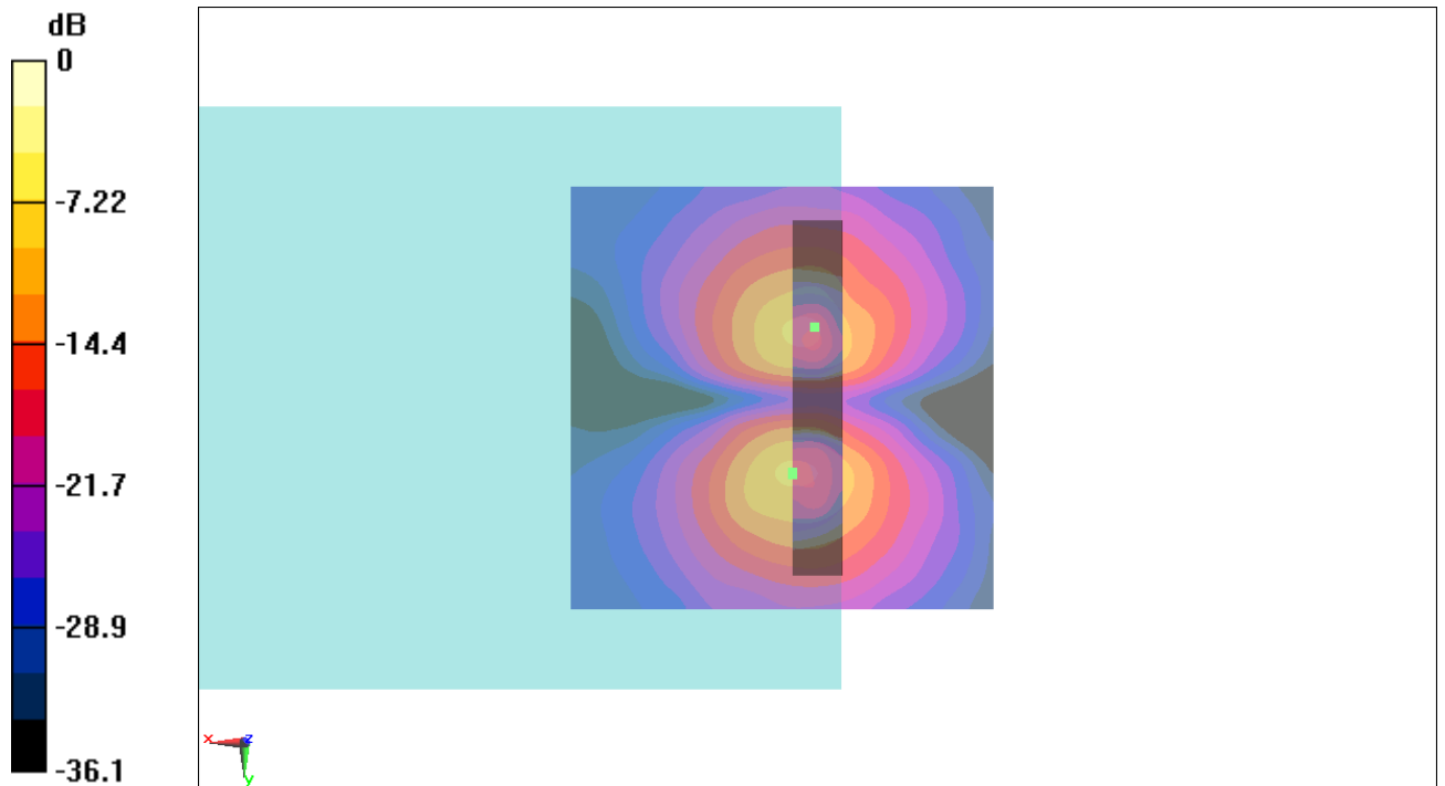
Fig B.17 T-Coil CDMA 1880_Channel 25
