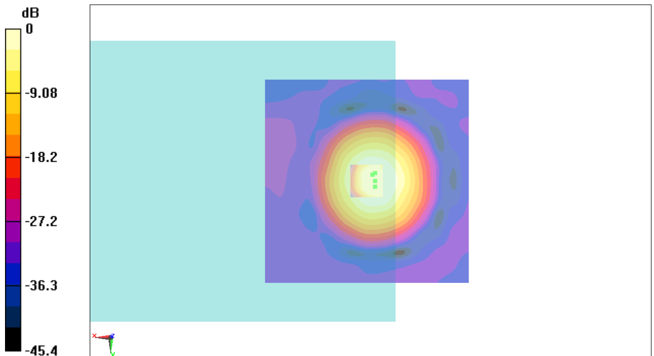
Fig B.12 T-Coil CDMA 1880_Channel 1175
