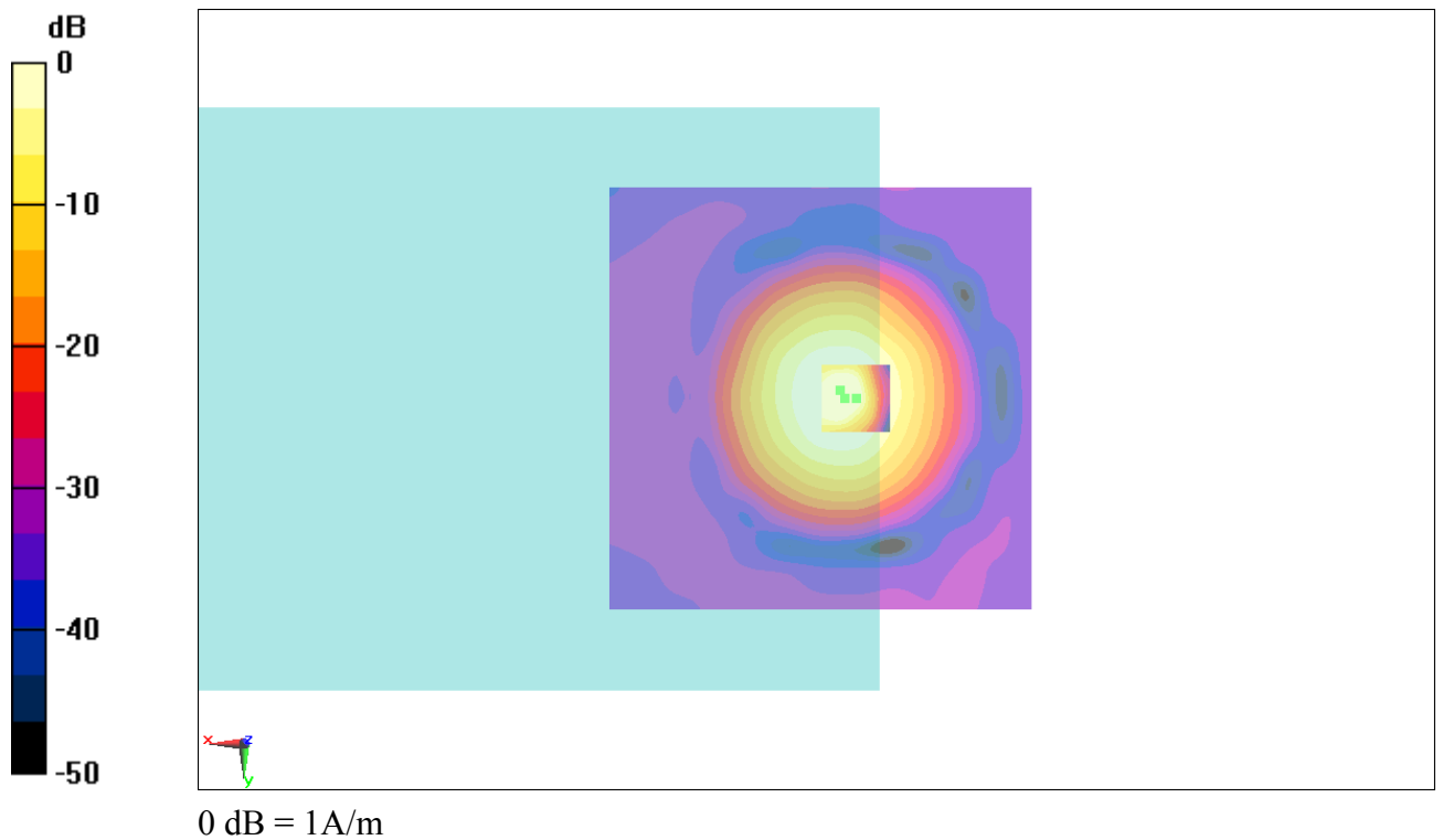
Fig B.3 T-Coil CDMA 835_Channel 777
