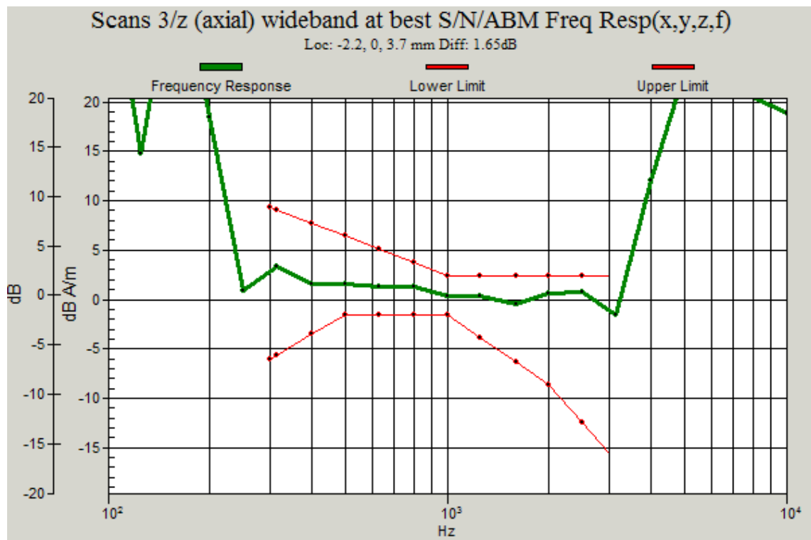
Figure C.3 Frequency Response of CDMA 835_Channel 1013
