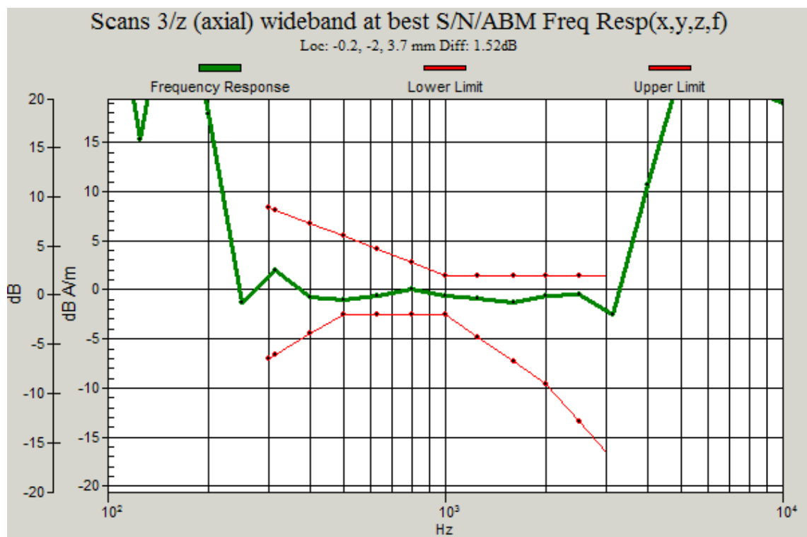
Figure C.6 Frequency Response of CDMA 1880_Channel 25
