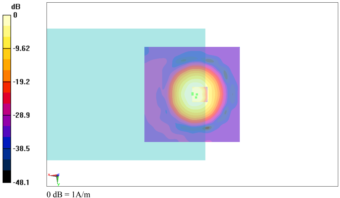
Fig B.15 T-Coil CDMA 1880_Channel 600
