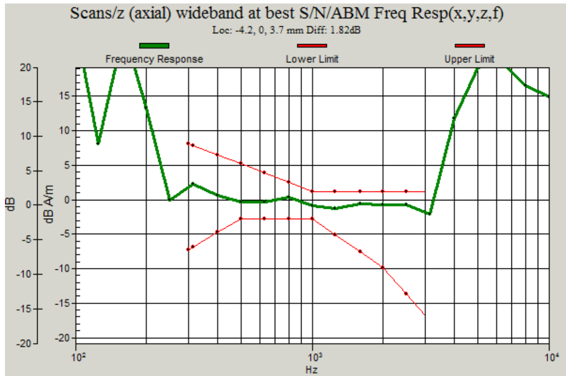
Figure C.1 Frequency Response of CDMA 835_Channel 777
