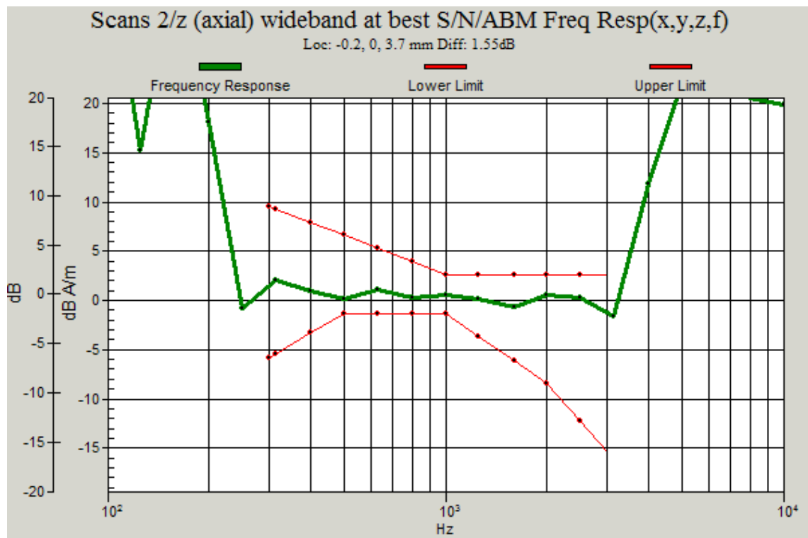
Figure C.5 Frequency Response of CDMA 1880_Channel 600
