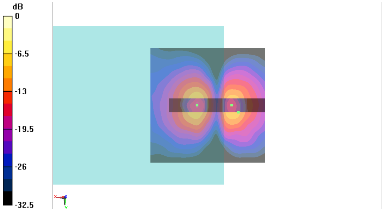
Fig B.13 T-Coil CDMA 1880_Channel 600
