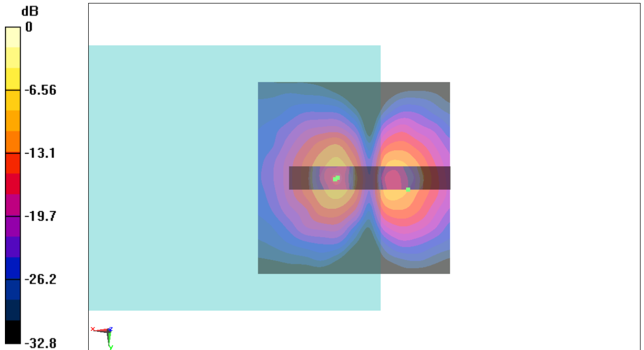
Fig B.7 T-Coil CDMA 835_Channel 1013
