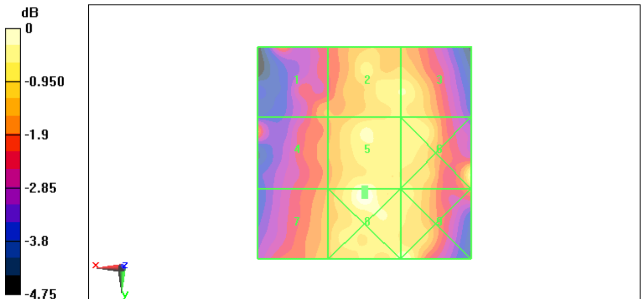
Fig B.7 HAC RF E-Field CDMA 835 High
