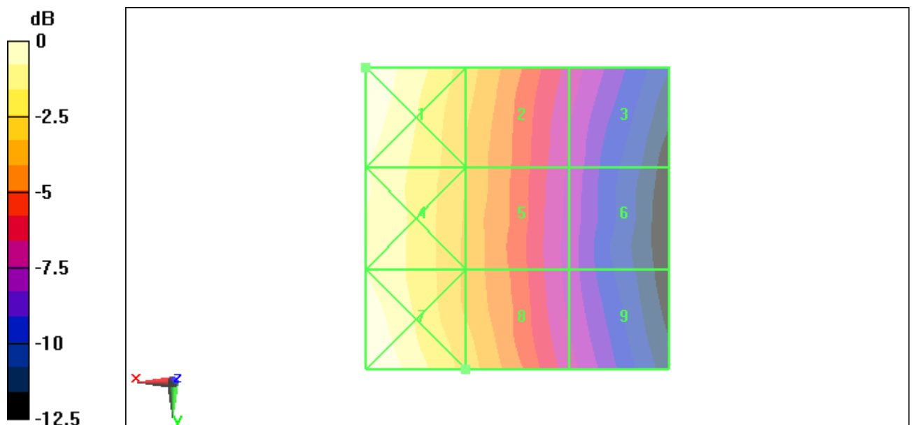
Fig B.13 HAC RF H-Field CDMA 835 High
