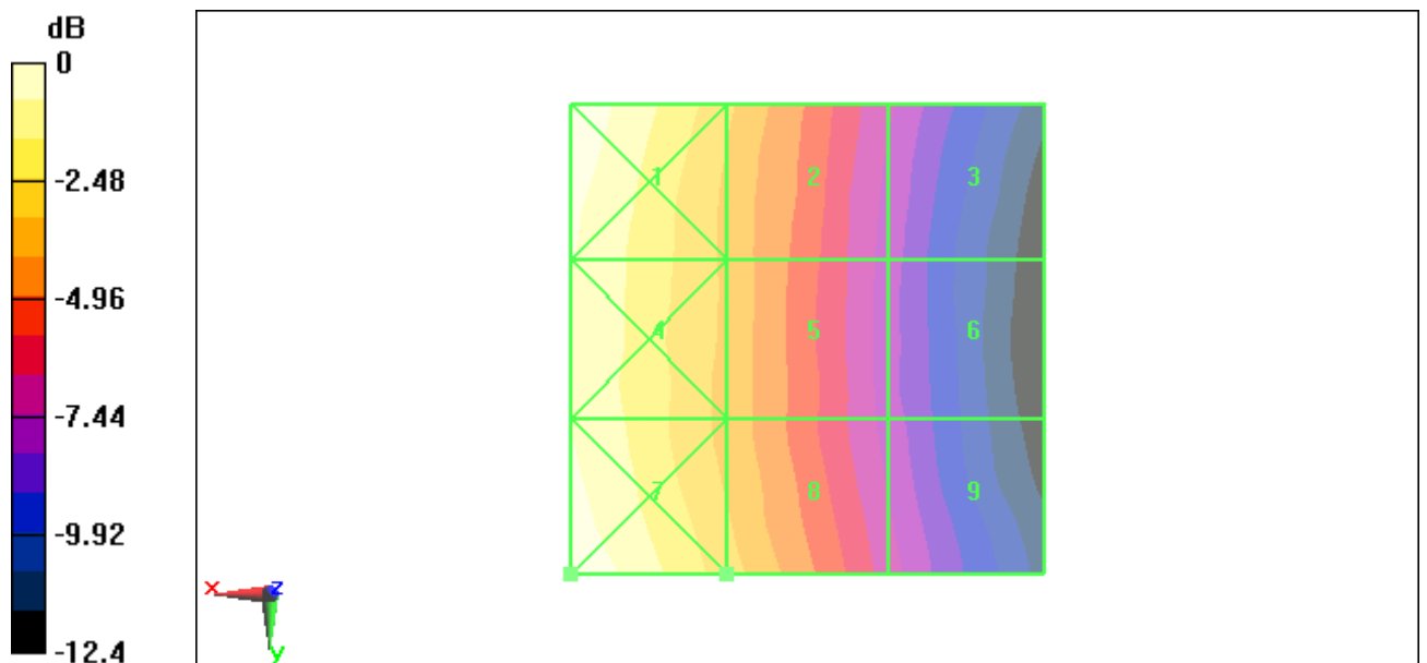
Fig B.14 HAC RF H-Field CDMA 835 Middle
