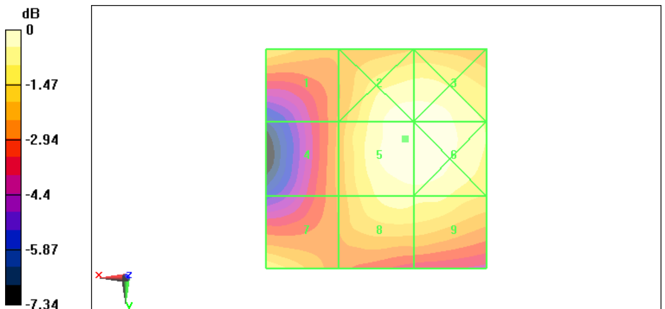
Fig B.16 HAC RF H-Field CDMA 1900 High
