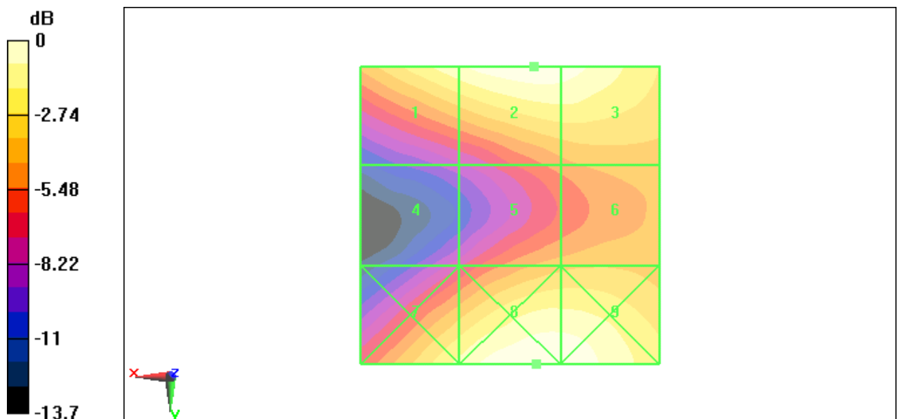
Fig B.4 HAC RF E-Field CDMA 1900 High
