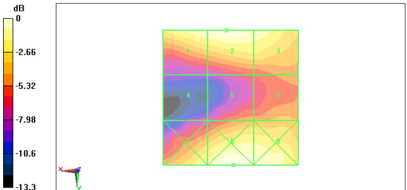
Fig B.12 HAC RF E-Field CDMA 1900 Low
