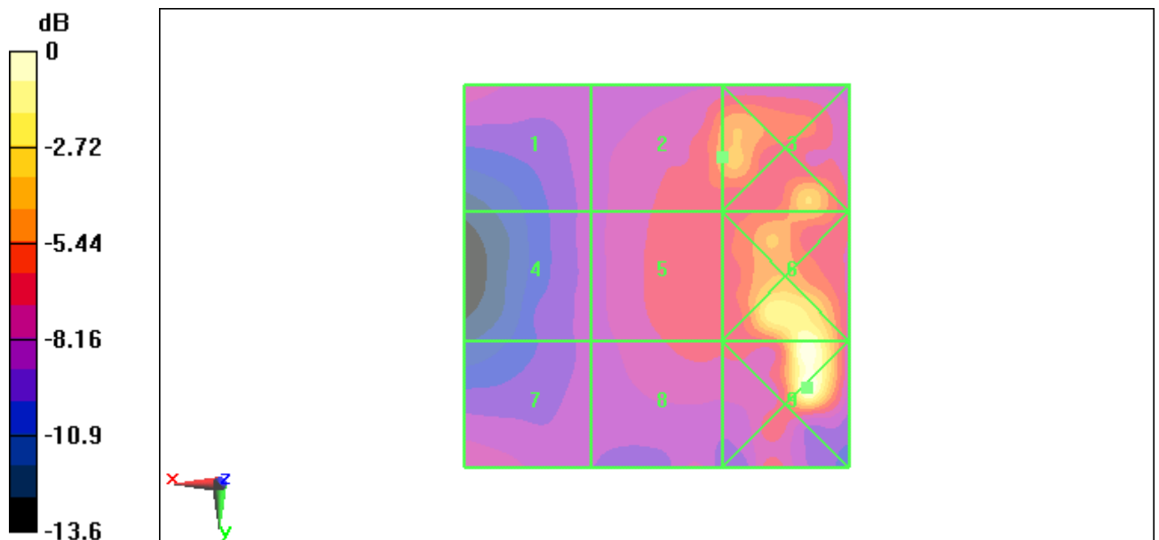
Fig B.22 HAC RF H-Field CDMA 1900 High
