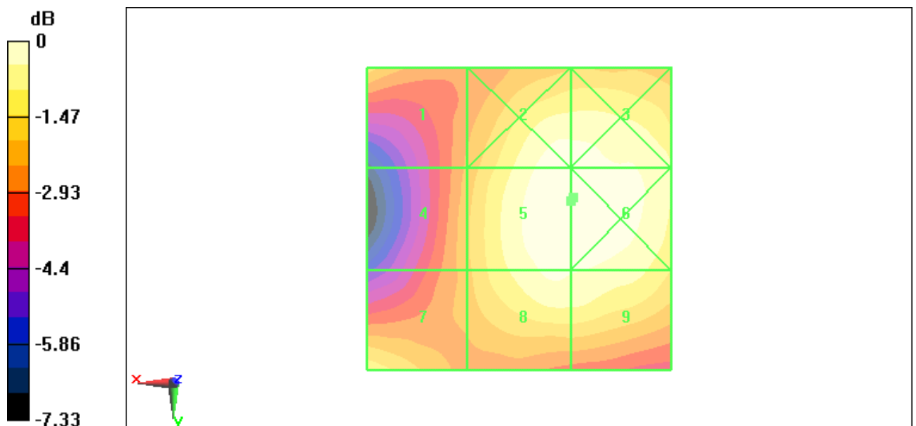
Fig B.17 HAC RF H-Field CDMA 1900 Middle
