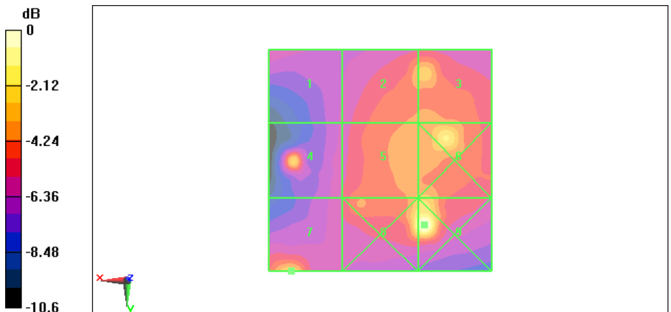
Fig B.24 HAC RF H-Field CDMA 1900 Low
