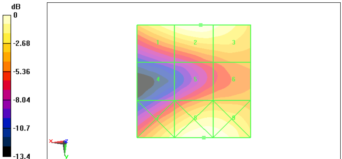
Fig B.5 HAC RF E-Field CDMA 1900 Middle
