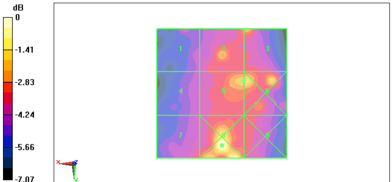
Fig B.9 HAC RF E-Field CDMA 835 Low
