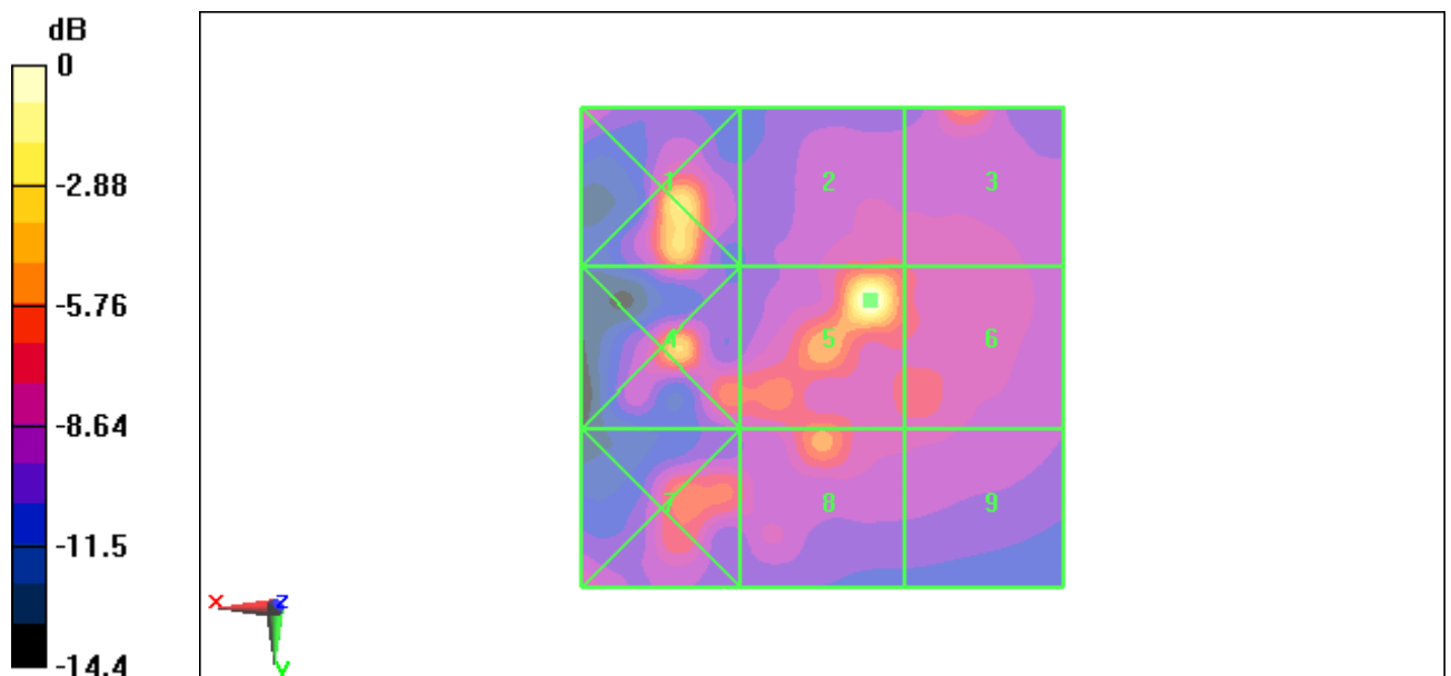
Fig B.23 HAC RF H-Field CDMA 1900 Middle
