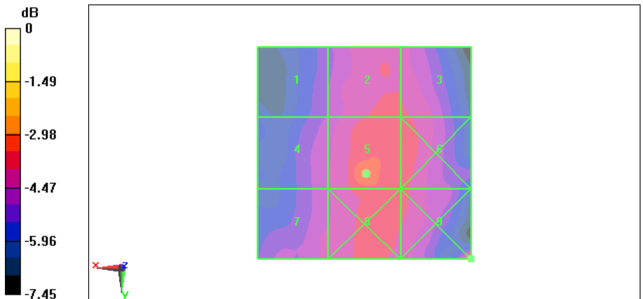
Fig B.8 HAC RF E-Field CDMA 835 Middle
