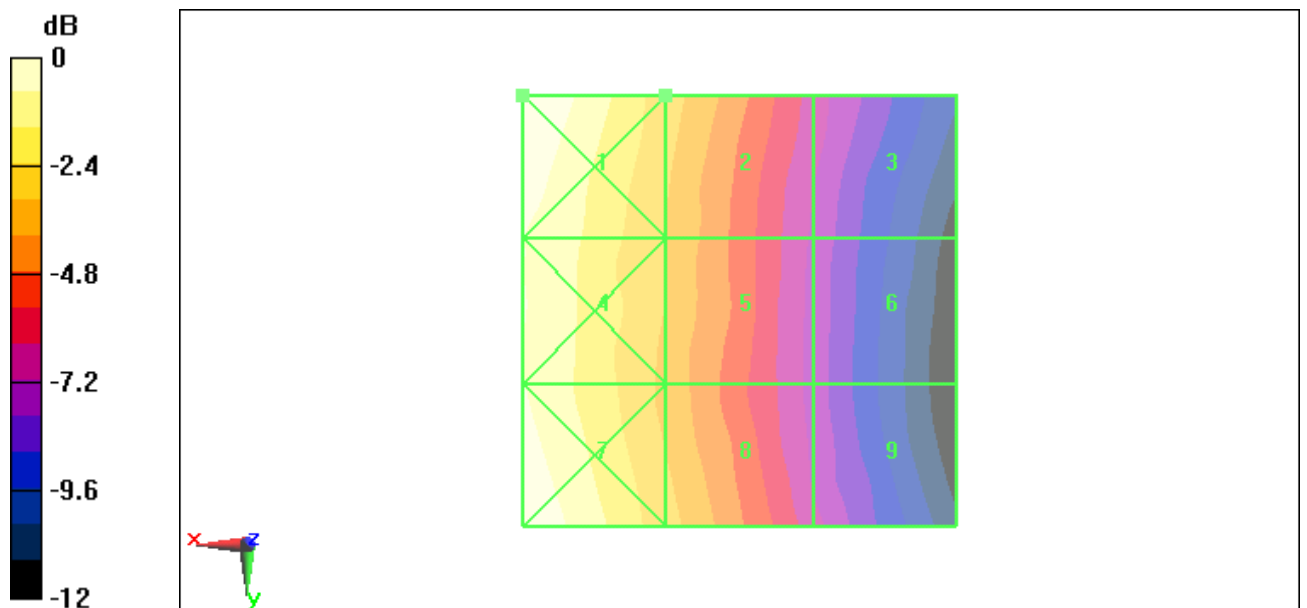
Fig B.15 HAC RF H-Field CDMA 835 Low
