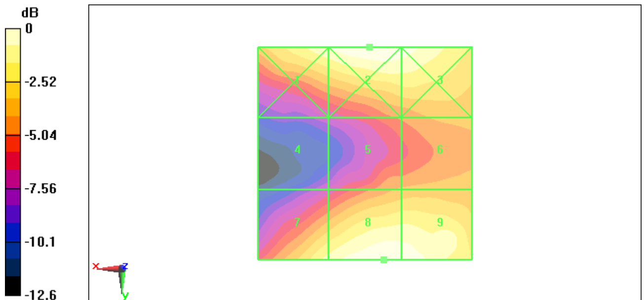
Fig B.10 HAC RF E-Field CDMA 1900 High
