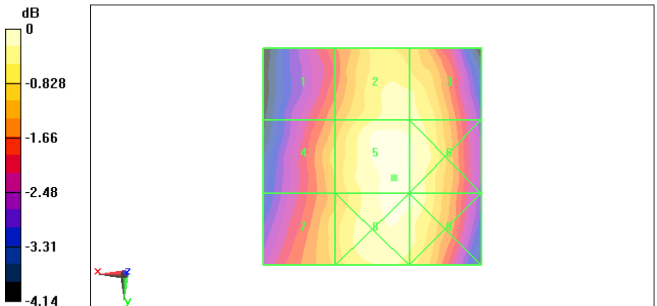
Fig B.3 HAC RF E-Field CDMA 835 Low
