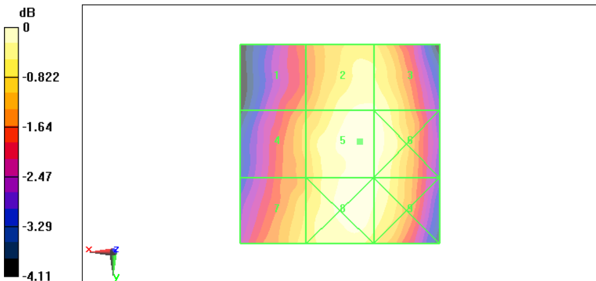
Fig B.1 HAC RF E-Field CDMA 835 High
