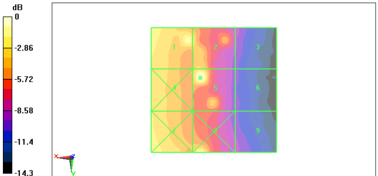
Fig B.20 HAC RF H-Field CDMA 835 Middle
