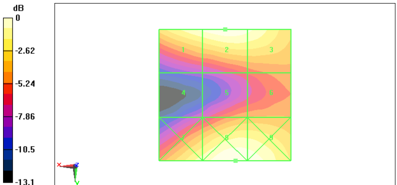
Fig B.6 HAC RF E-Field CDMA 1900 Low
