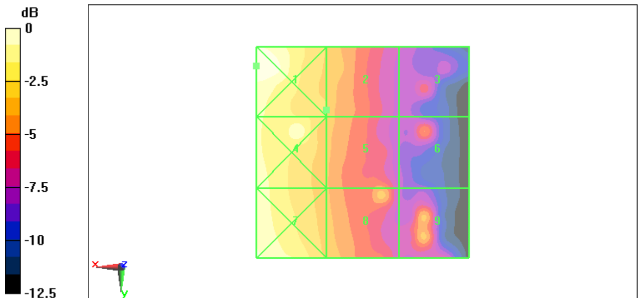
Fig B.21 HAC RF H-Field CDMA 835 Low
