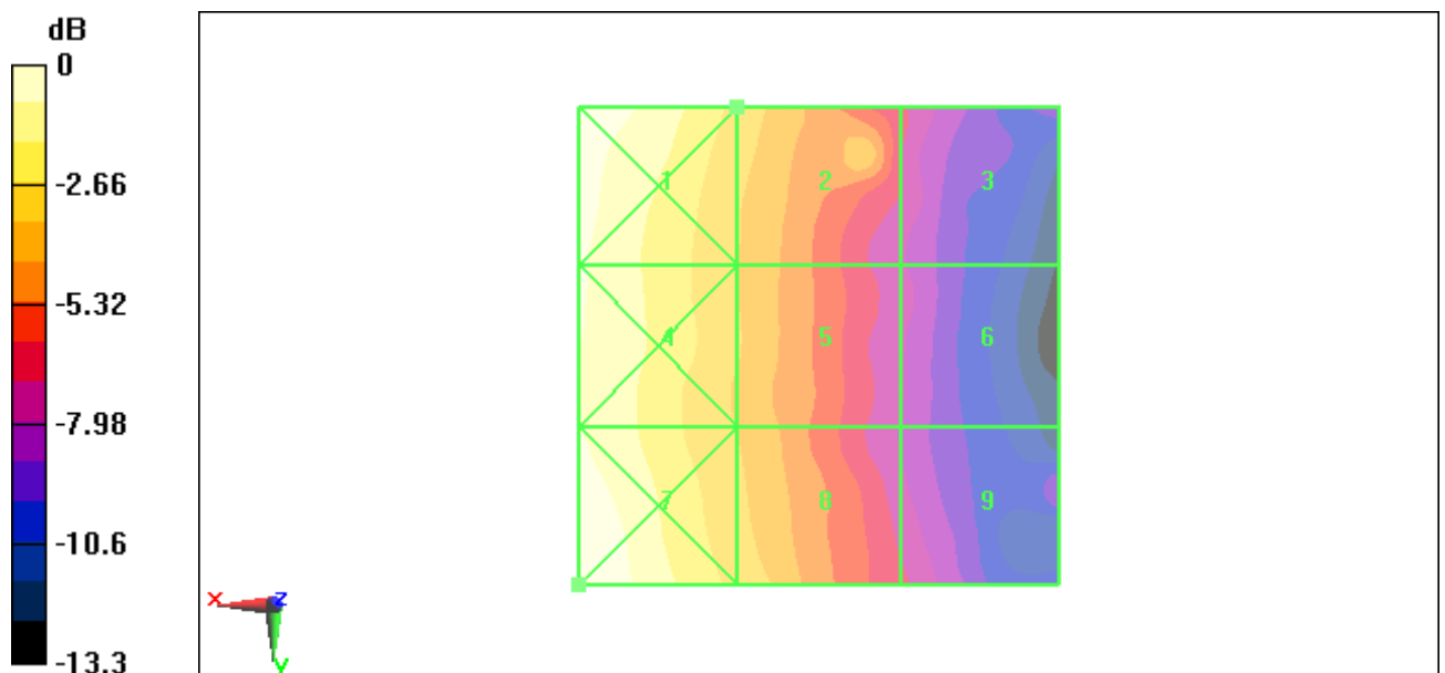
Fig B.19 HAC RF H-Field CDMA 835 High
