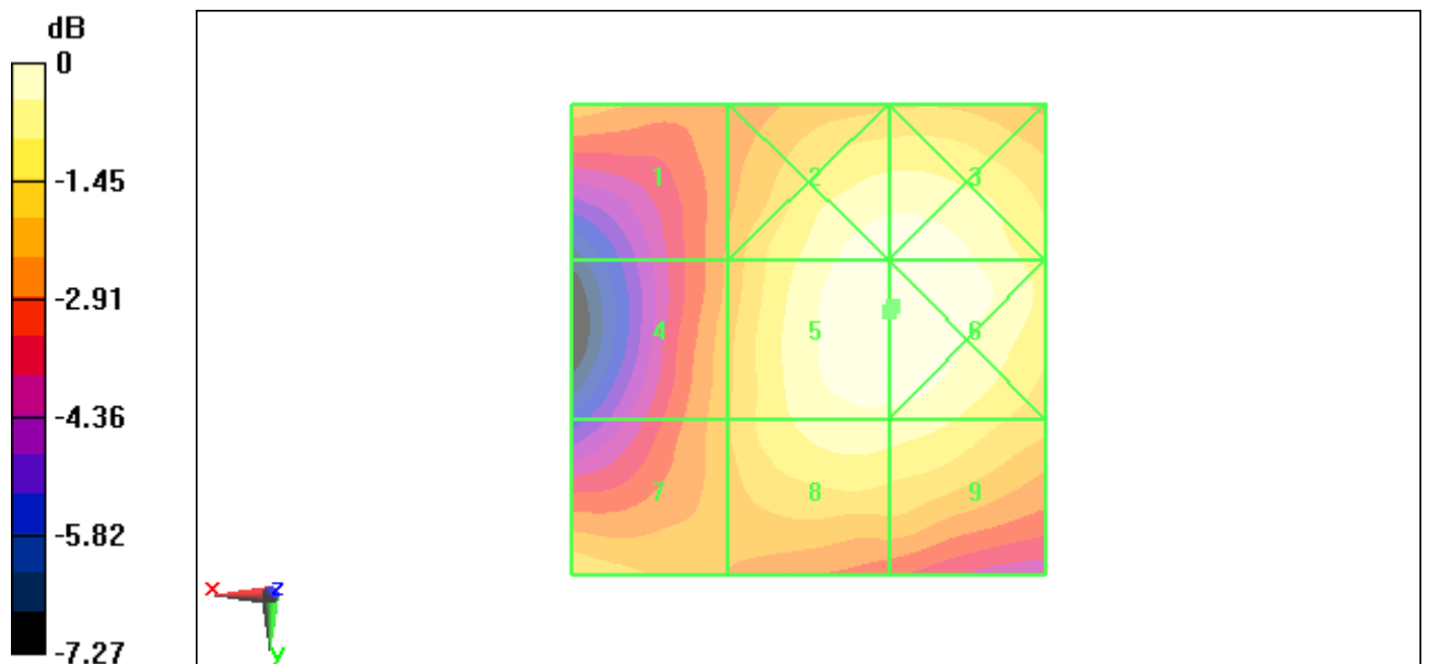
Fig B.18 HAC RF H-Field CDMA 1900 Low
