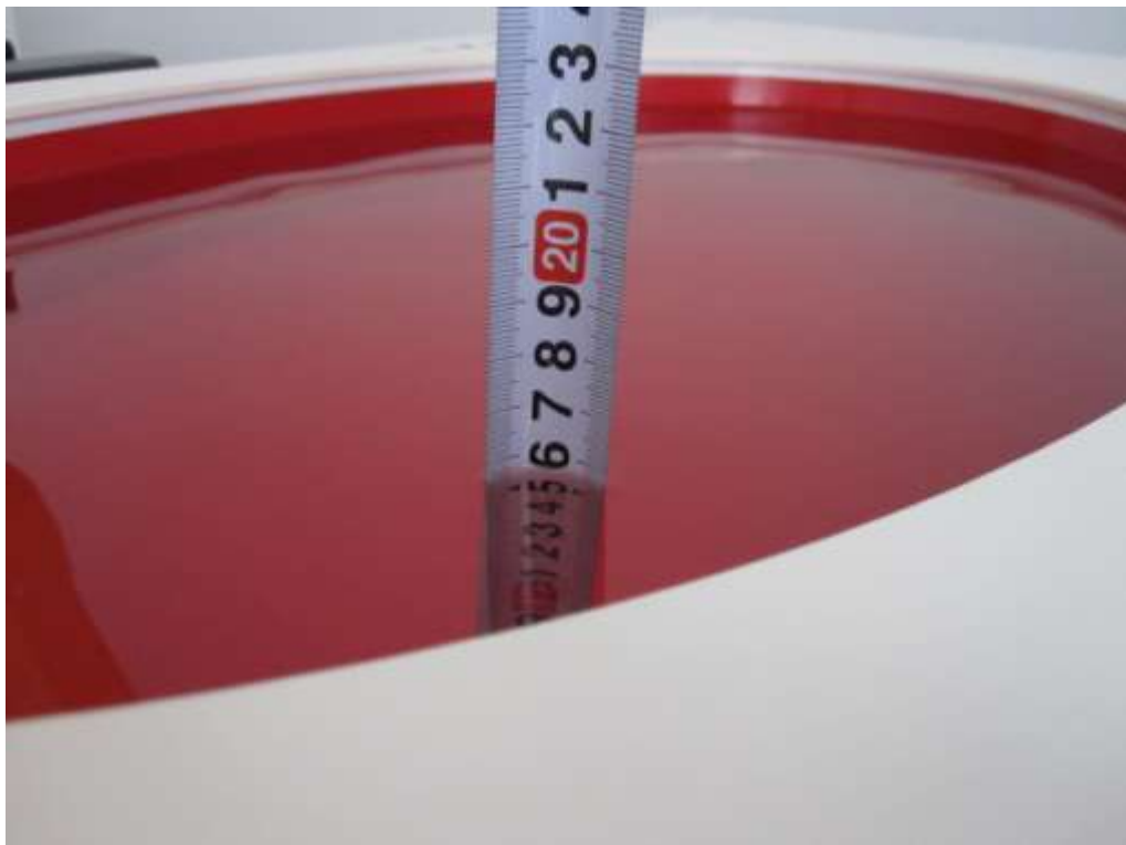
Picture 5: Liquid depth in the EL14 Phantom (2450 MHz) (15.4cm deep)
