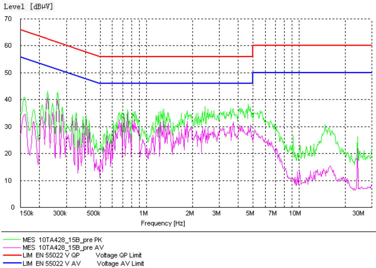
Figure A.3 Conducted Emission
