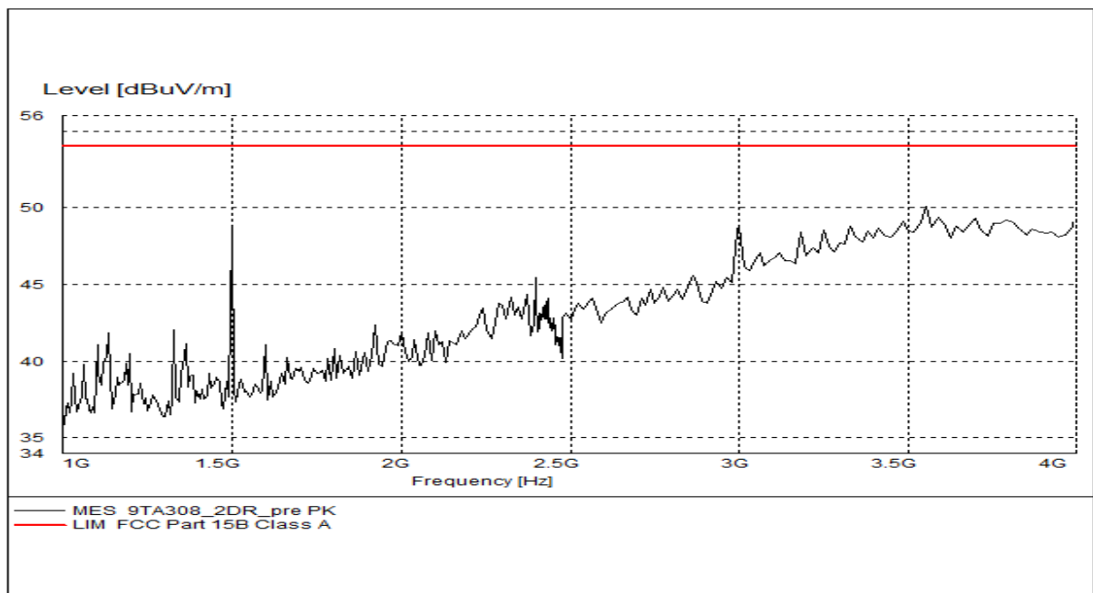
Figure A.2 Radiated Emission from 1GHz to 4GHz
