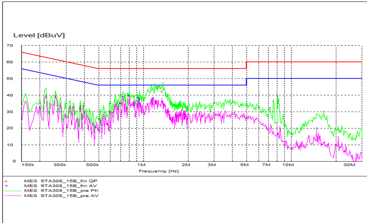
Figure A.3 Conducted Emission
