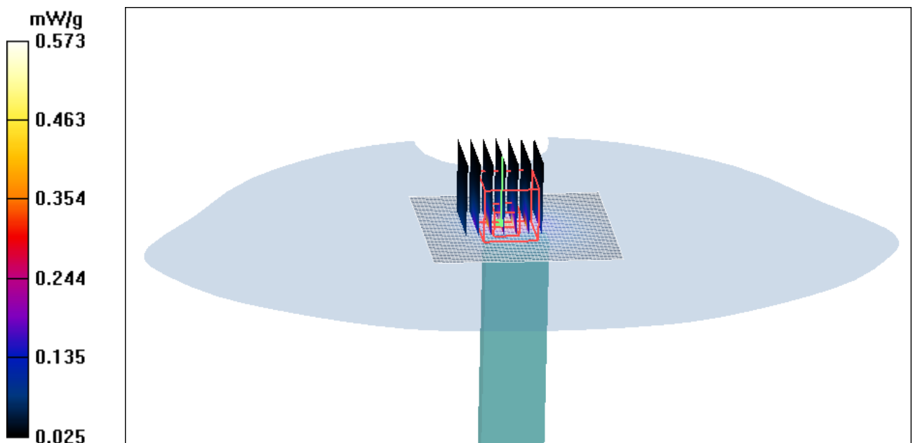
Figure 109 WCDMA Band V with BenQ Joybook R55V 180 degree Test Position 3 Channel 4182
