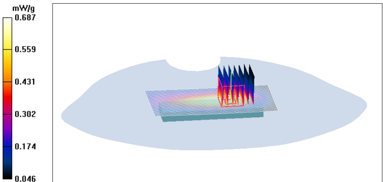
Figure 99 WCDMA Band V with BenQ Joybook R55V 180 degree Test Position 1 Channel 4182
