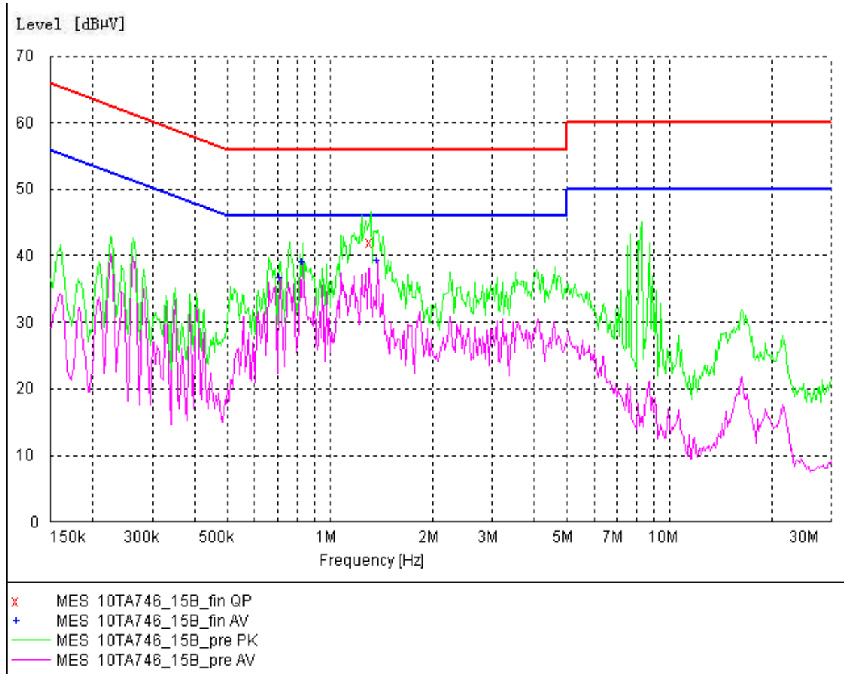
Figure A.3 Conducted Emission
