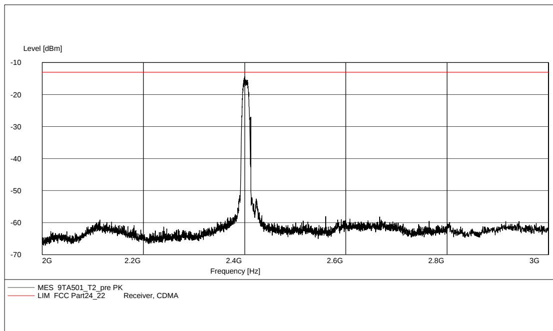
Fig 2 Radiated Spurious Emission (simultaneous transmission 1900 MHz and WiFi 802.11b, 2GHz-3GHz)
