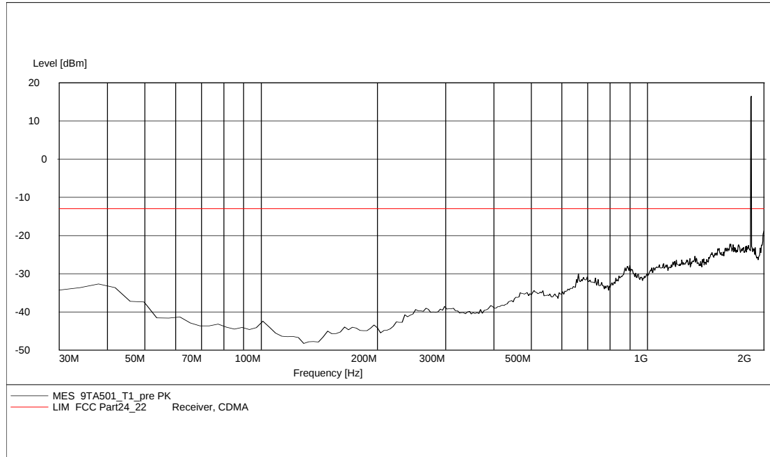
Fig 1 Radiated Spurious Emission (simultaneous transmission 1900 MHz and WiFi 802.11b, 30MHz-2GHz)
