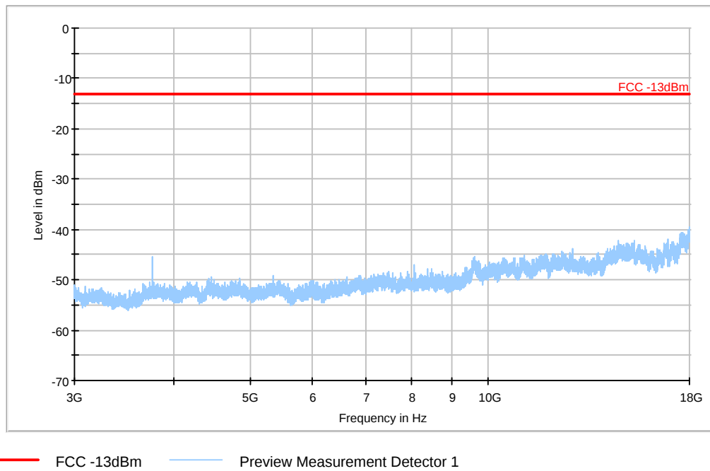
Fig 3 Radiated Spurious Emission (simultaneous transmission 1900 MHz and WiFi 802.11b, 3GHz-18GHz)
