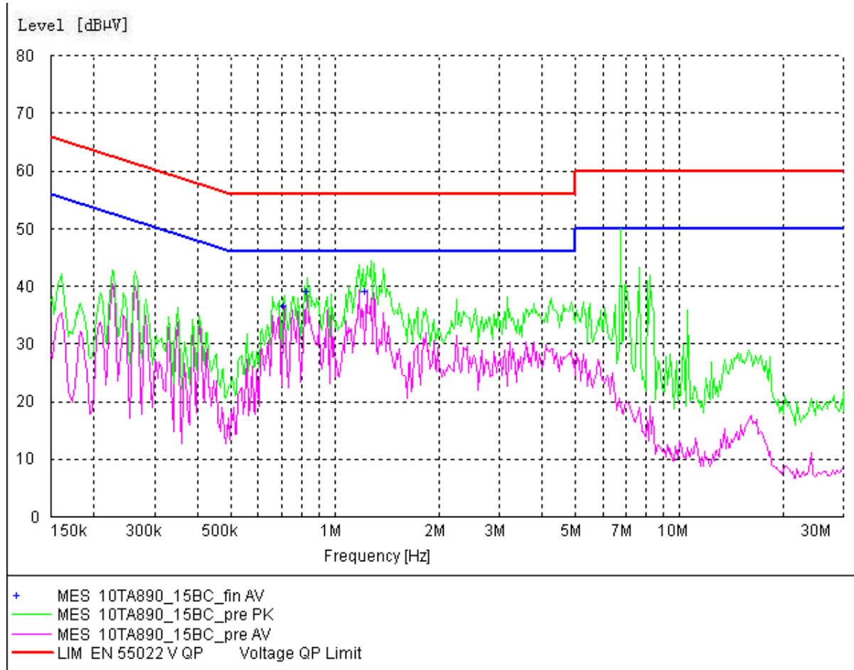
Figure A.6 Conducted Emission
