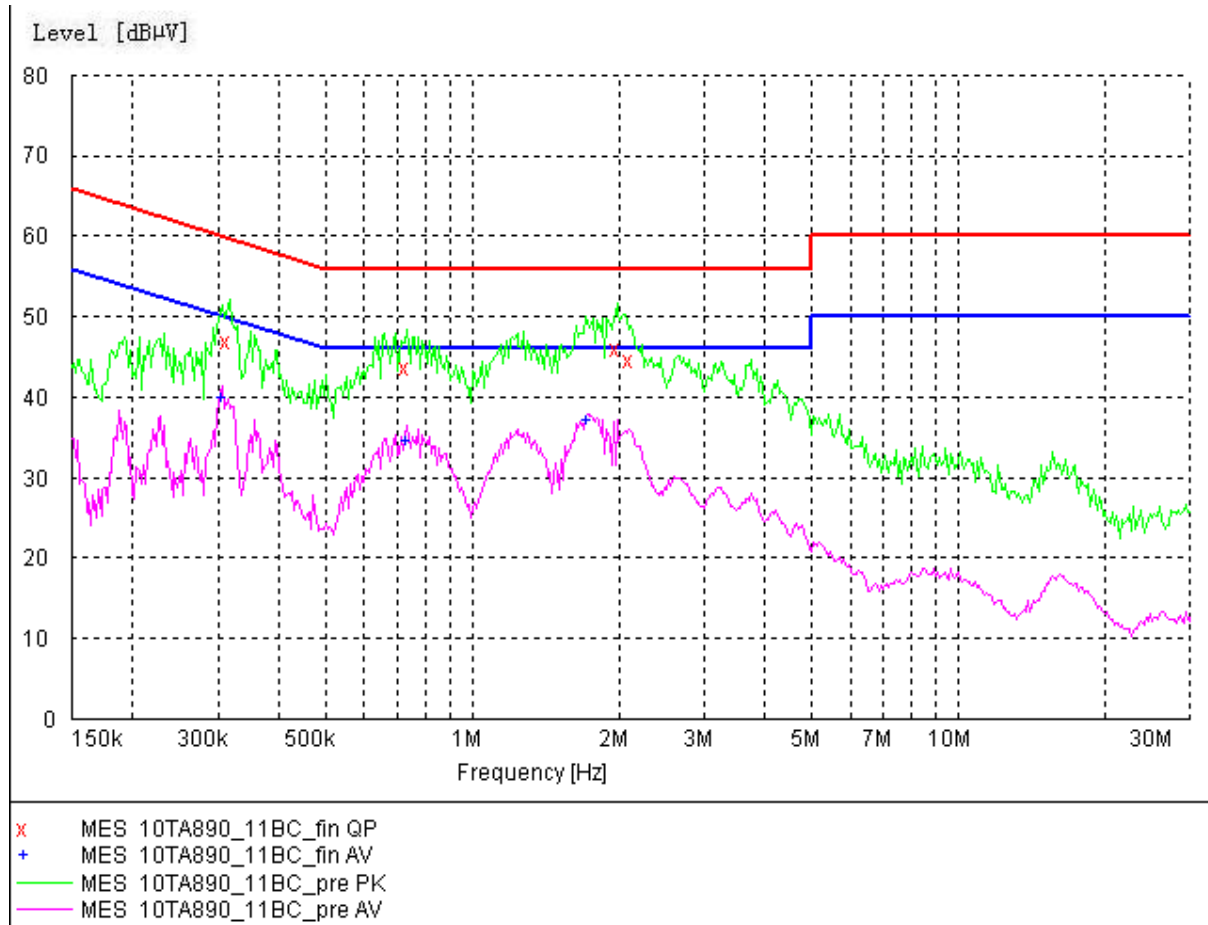
Figure A.5 Conducted Emission
