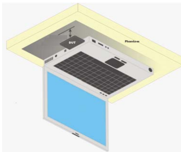
Fig. 3 Lap-held position, bottom of the computer is touching the phantom
