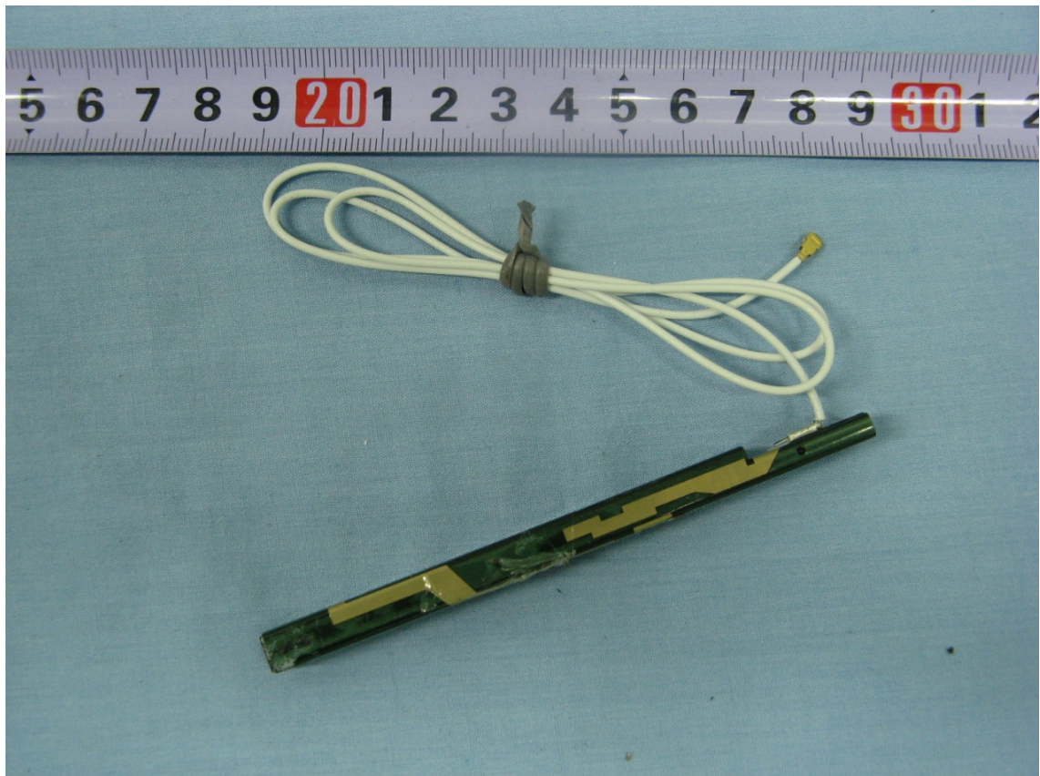
Q78-ZTEMF200 External Photo
