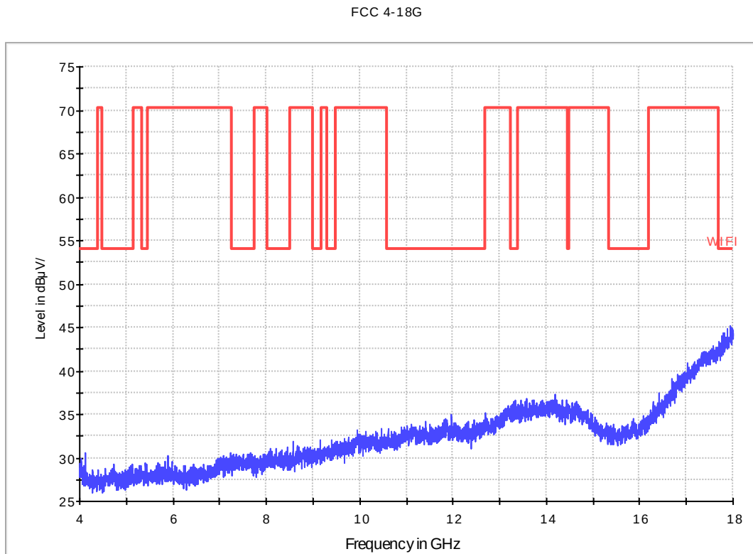
Fig. 39 Radiated Spurious Emission (802.11b, Ch11, 4 GHz-18 GHz)
