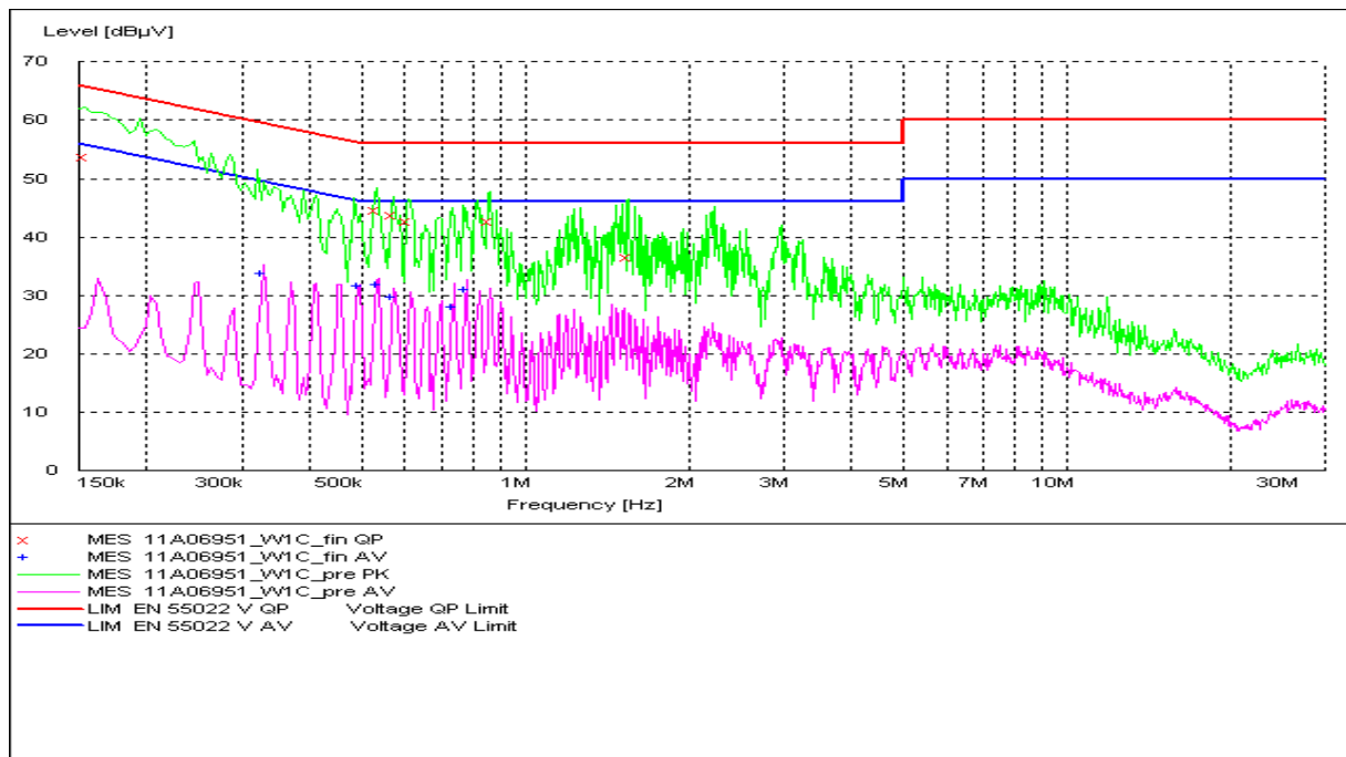
Fig. 52 AC Powerline Conducted Emission-802.11b
