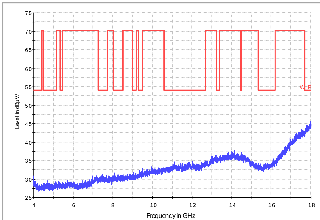
Fig. 46 Radiated Spurious Emission (802.11g, Ch6, 4 GHz-18 GHz)
