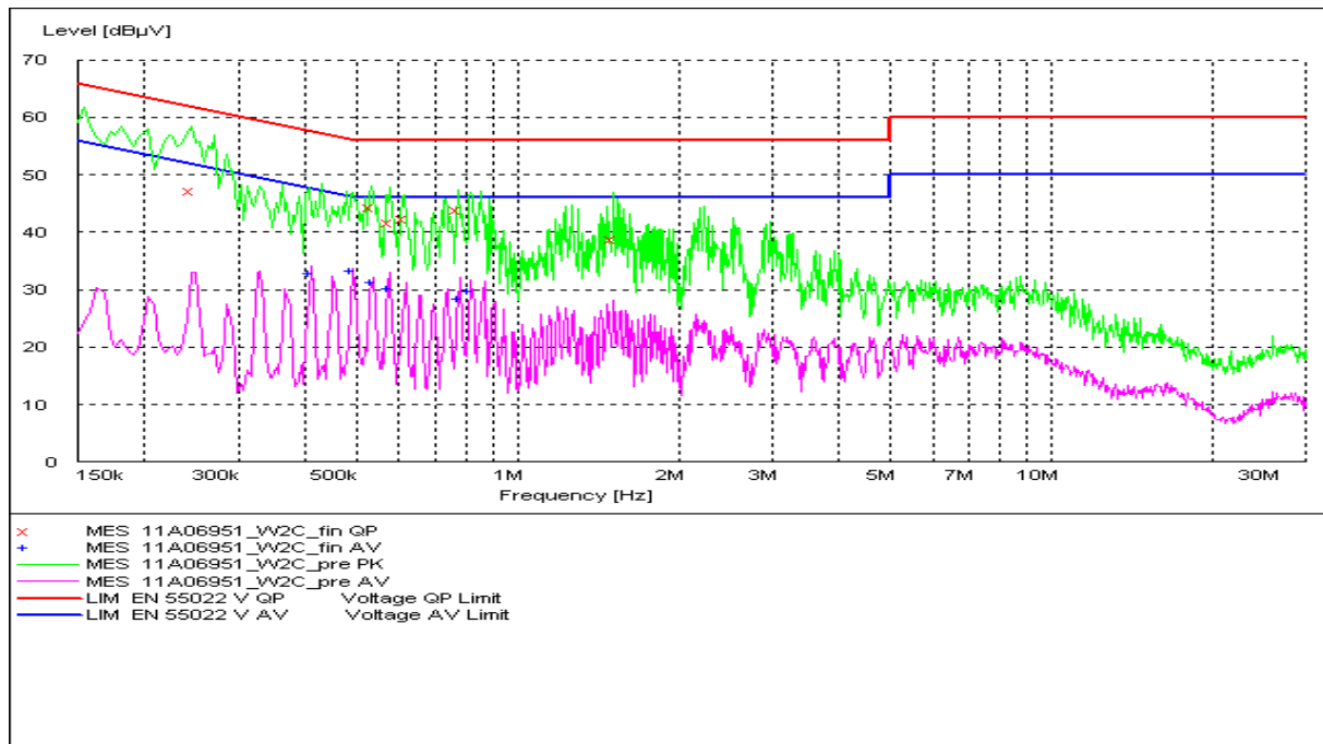
Fig. 53 AC Powerline Conducted Emission-802.11g
