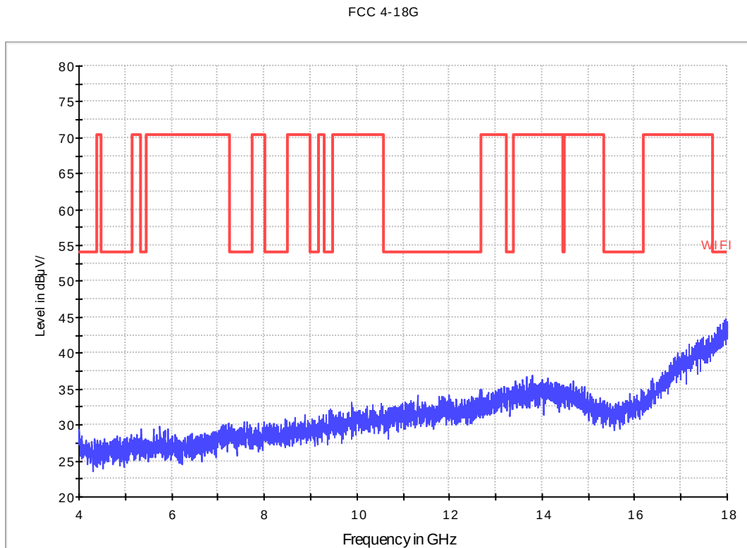
Fig. 35 Radiated Spurious Emission (802.11b, Ch6, 4 GHz-18 GHz)
