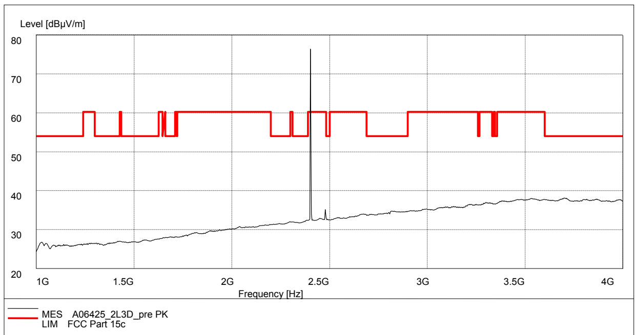
Fig.83. Radiated emission: 8DPSK, Channel 0, 1 GHz - 4 GHz
