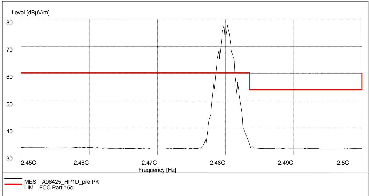
Fig.68. Radiated emission (Power) GFSK, high channel
