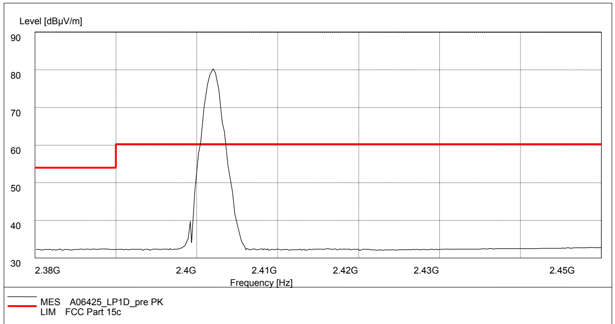
Fig.67. Radiated emission (Power): GFSK, low channel
