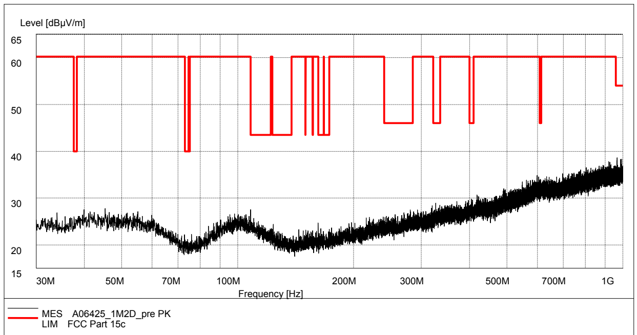
Fig.73. Radiated emission: \pi/4 DQPSK, Channel 39, 30 MHz - 1 GHz
