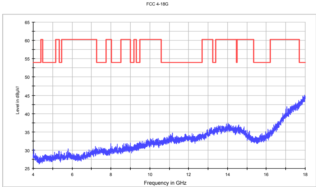
Fig.66. Radiated emission: GFSK, Channel 78, 4 GHz - 18 GHz
