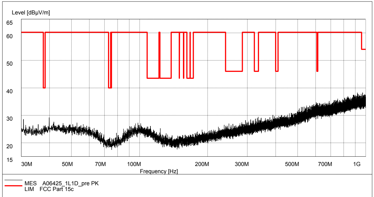
Fig.58. Radiated emission: GFSK, Channel 0, 30 MHz - 1 GHz
