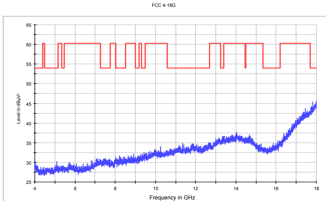
Fig.84. Radiated emission: 8DPSK, Channel 0, 4 GHz - 18 GHz
