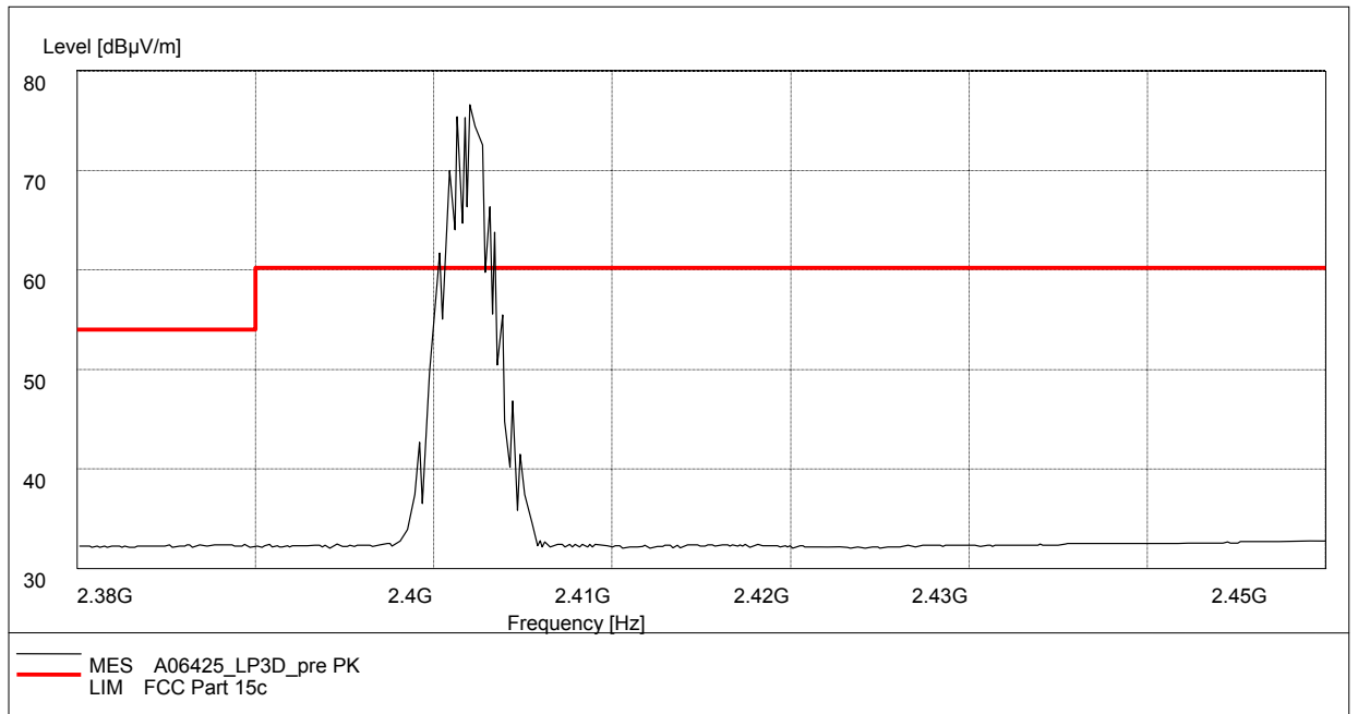
Fig.91. Radiated emission (Power): 8DPSK, low channel
