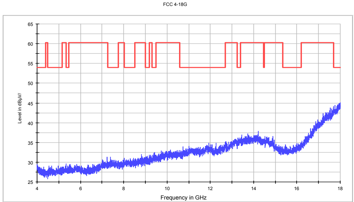
Fig.90. Radiated emission: 8DPSK, Channel 78, 4 GHz - 18 GHz
