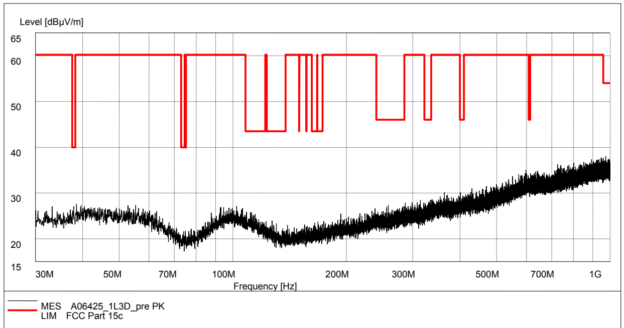
Fig.82. Radiated emission: 8DPSK, Channel 0, 30 MHz - 1 GHz
