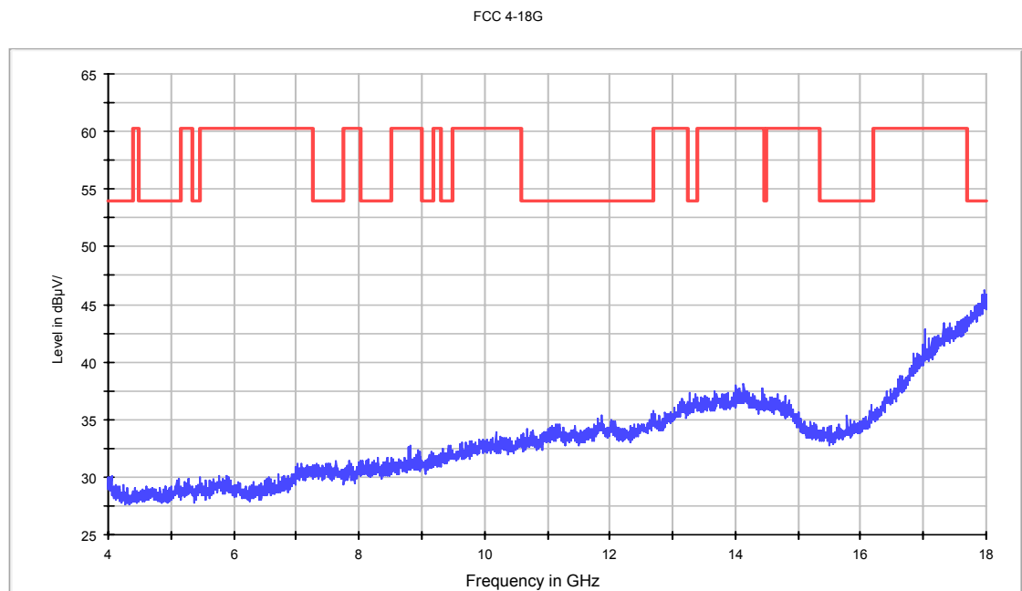
Fig.75. Radiated emission: \pi/4 DQPSK, Channel 39, 4 GHz - 18 GHz
