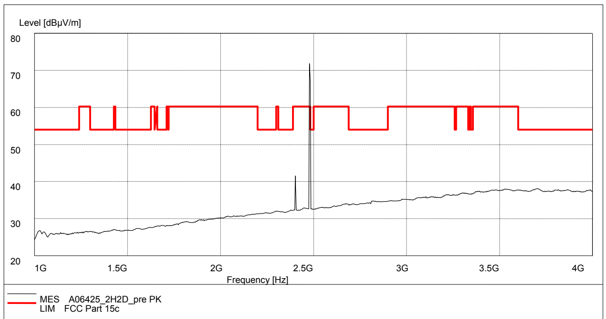
Fig.77. Radiated emission: \pi/4 DQPSK, Channel 78, 1 GHz - 4 GHz
