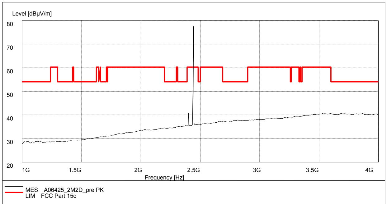
Fig.74. Radiated emission: \pi/4 DQPSK, Channel 39, 1 GHz - 4 GHz
