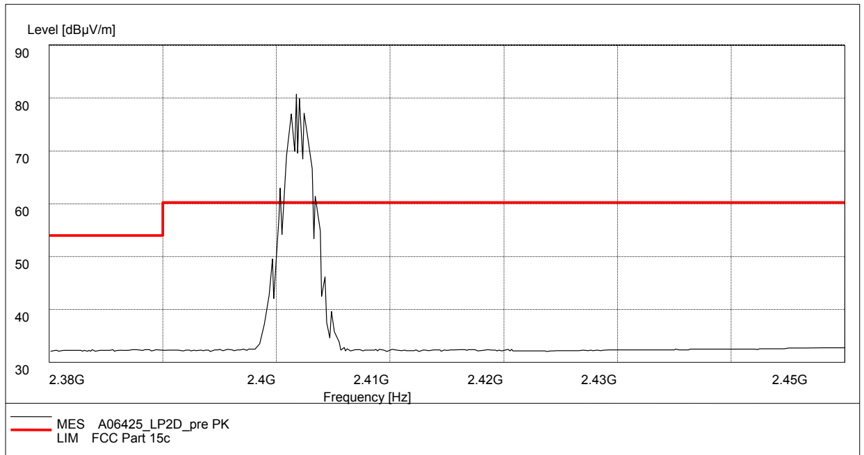
Fig.79. Radiated emission (Power): \pi/4 DQPSK, low channel
