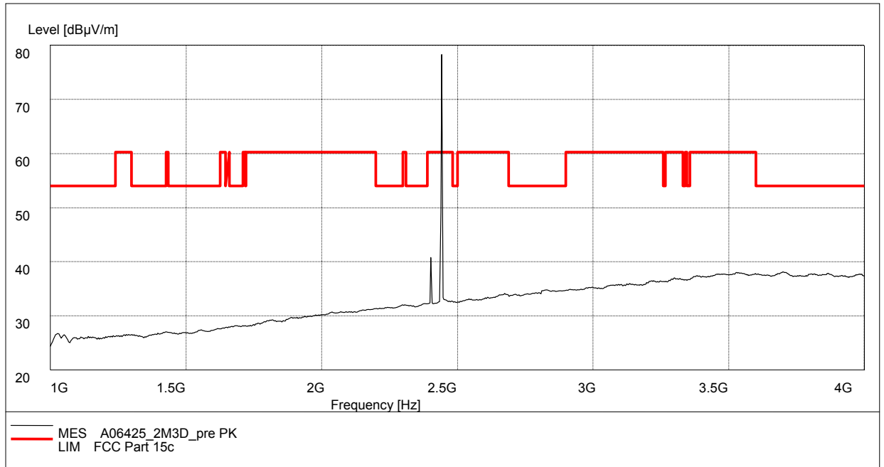
Fig.86. Radiated emission: 8DPSK, Channel 39, 1 GHz - 4 GHz
