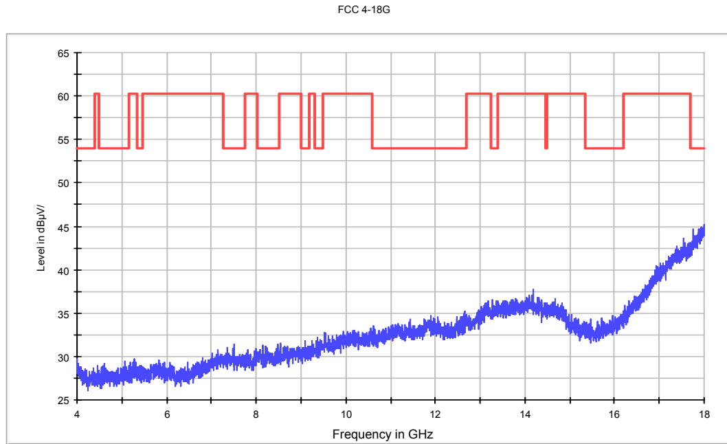
Fig.60. Radiated emission: GFSK, Channel 0, 4 GHz - 18 GHz
