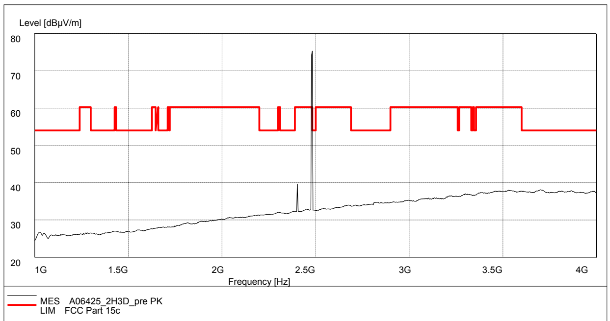
Fig.89. Radiated emission: 8DPSK, Channel 78, 1 GHz - 4 GHz
