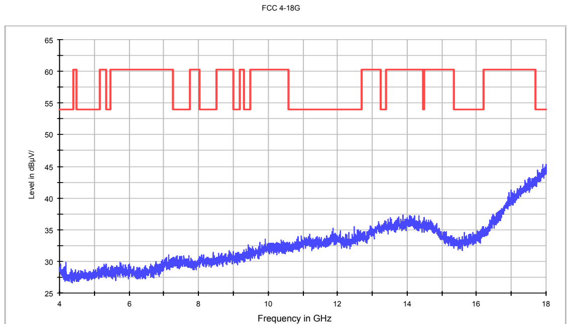
Fig.87. Radiated emission: 8DPSK, Channel 39, 4 GHz - 18 GHz
