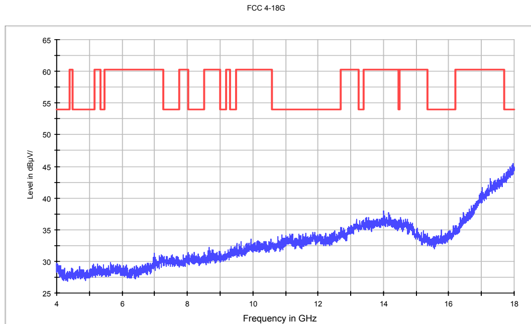
Fig.63. Radiated emission: GFSK, Channel 39, 4 GHz - 18 GHz
