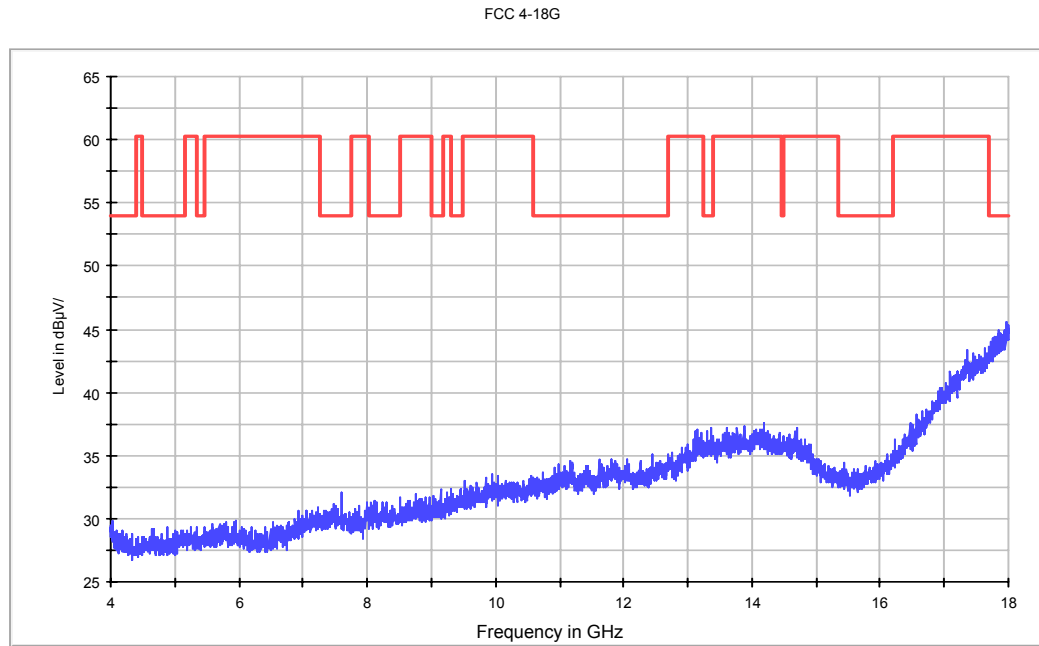
Fig.78. Radiated emission: \pi/4 DQPSK, Channel 78, 4 GHz - 18 GHz
