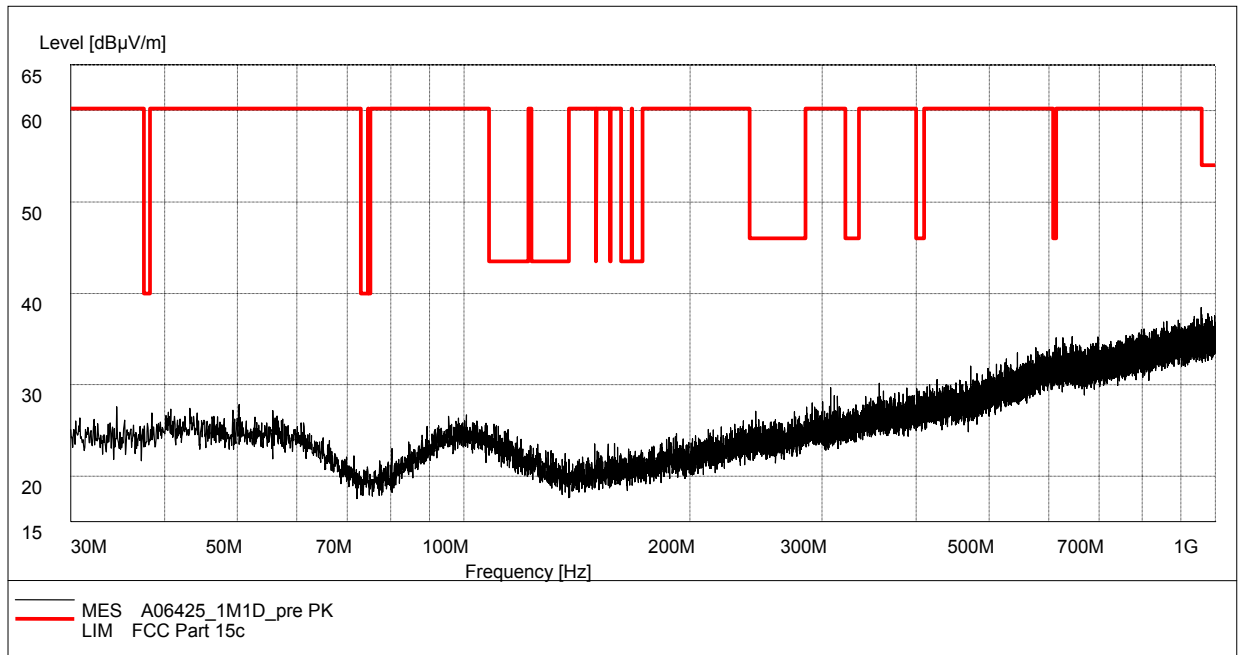
Fig.61. Radiated emission: GFSK, Channel 39, 30 MHz - 1 GHz
