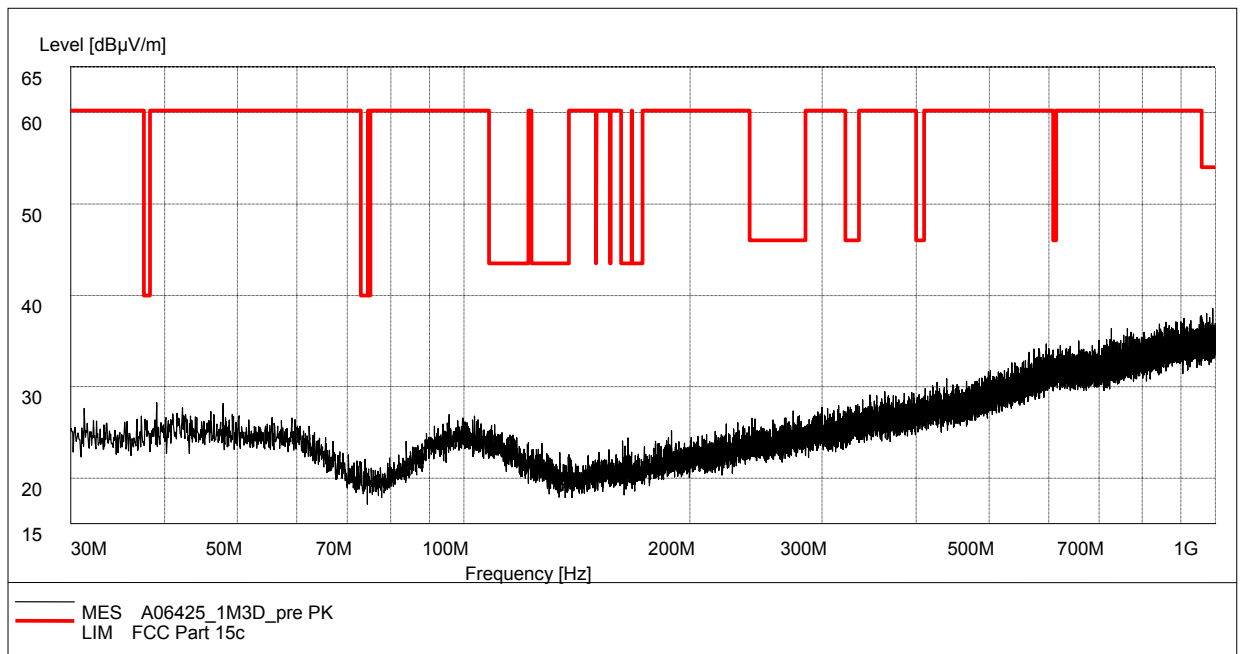
Fig.85. Radiated emission: 8DPSK, Channel 39, 30 MHz - 1 GHz
