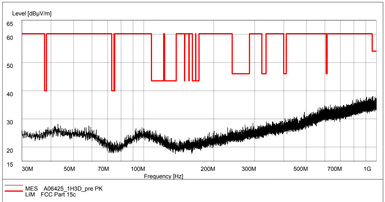
Fig.88. Radiated emission: 8DPSK, Channel 78, 30 MHz - 1 GHz
