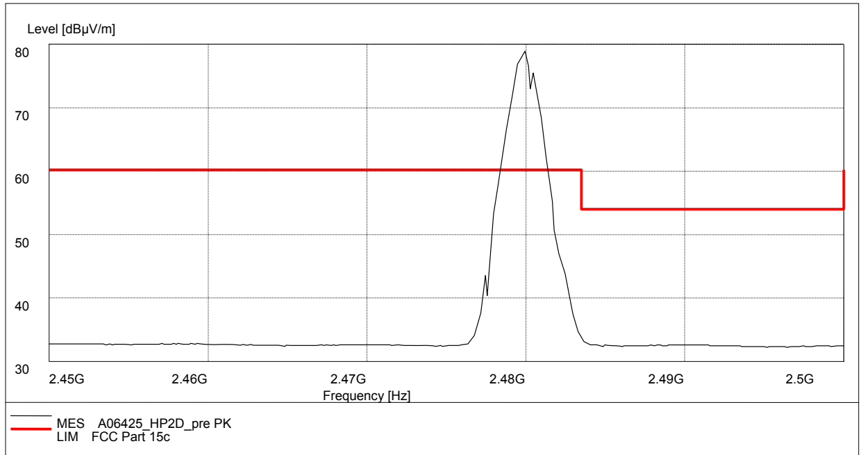
Fig.80. Radiated emission (Power): \pi/4 DQPSK, high channel
