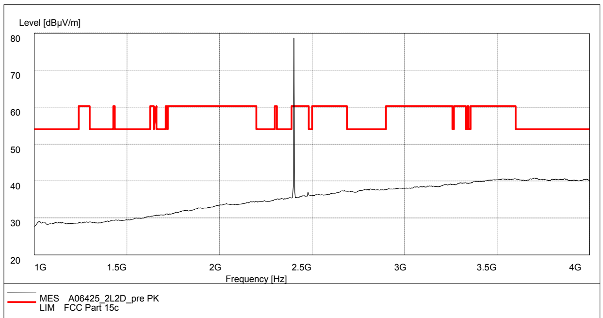
Fig.71. Radiated emission: \pi/4 DQPSK, Channel 0, 1 GHz - 4 GHz
