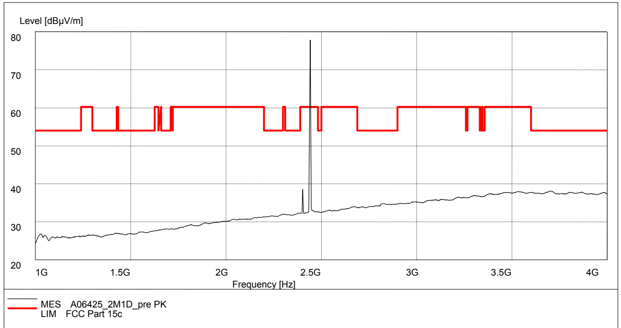
Fig.62. Radiated emission: GFSK, Channel 39, 1 GHz - 4 GHz
