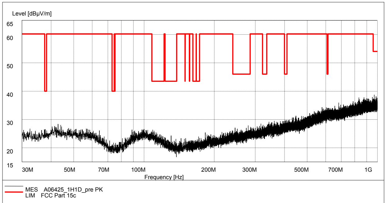
Fig.64. Radiated emission: GFSK, Channel 78, 30 MHz - 1 GHz
