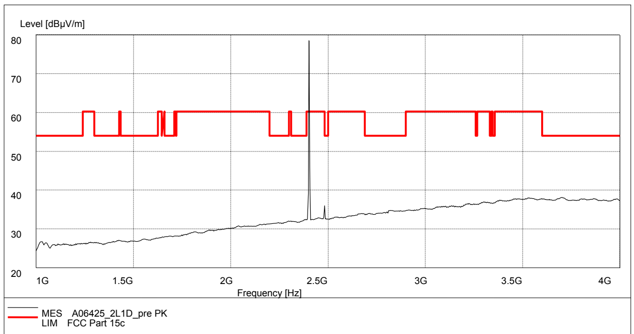
Fig.59. Radiated emission: GFSK, Channel 0, 1 GHz - 4 GHz
