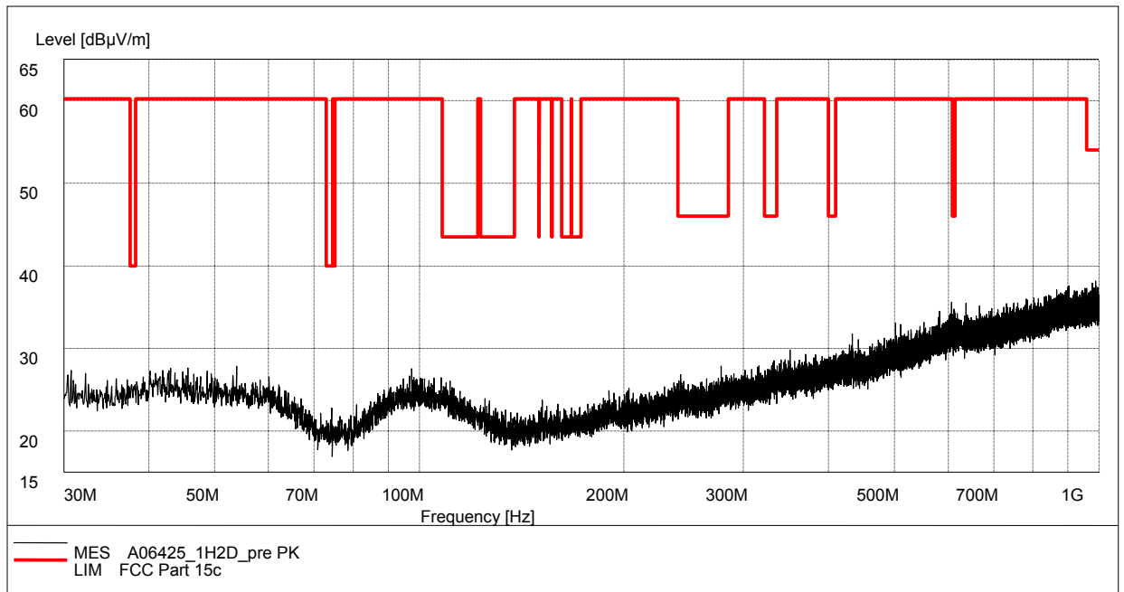
Fig.76. Radiated emission: \pi/4 DQPSK, Channel 78, 30 MHz - 1 GHz
