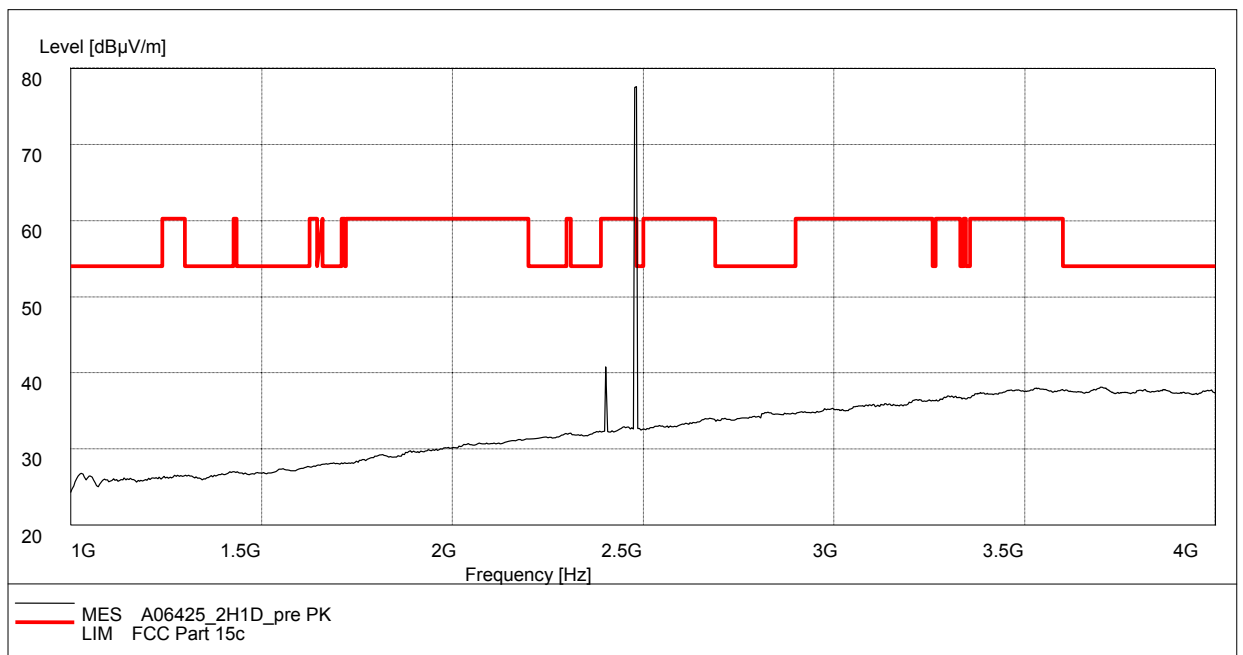
Fig.65. Fig.47 Radiated emission: GFSK, Channel 78, 1 GHz - 4 GHz
