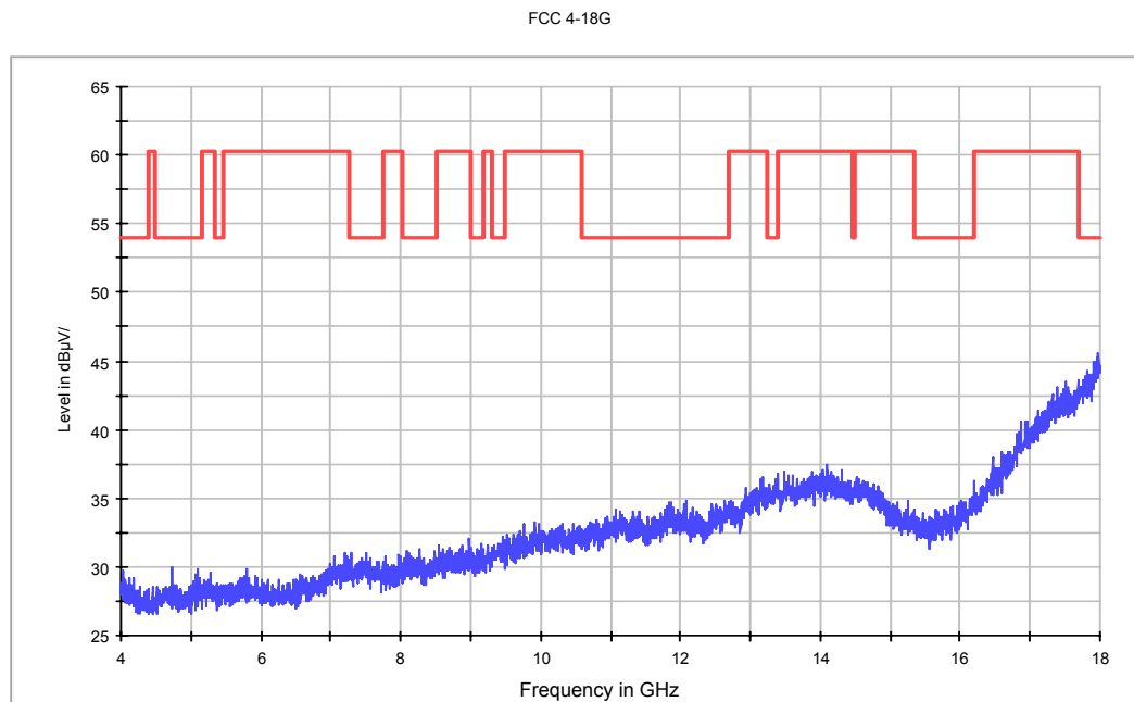
Fig.72. Radiated emission: \pi/4 DQPSK, Channel 0, 4 GHz - 18 GHz
