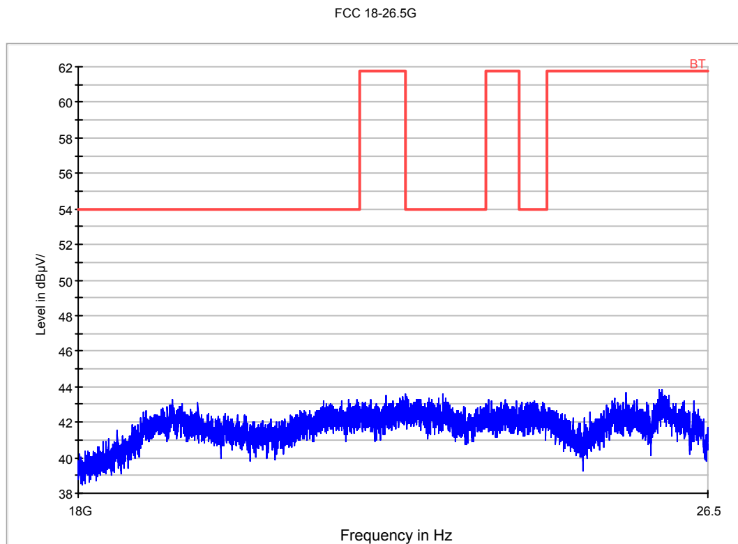
Fig.93. Radiated emission: 8DPSK, 18 GHz - 26 GHz
