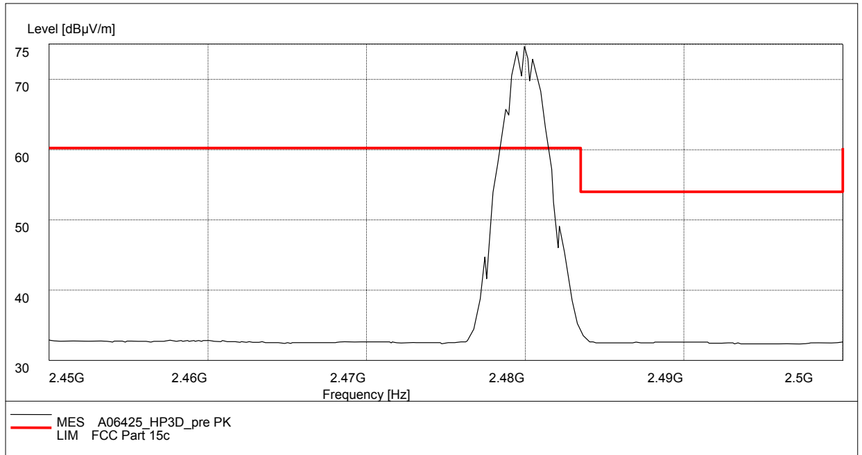
Fig.92. Radiated emission (Power): 8DPSK, high channel
