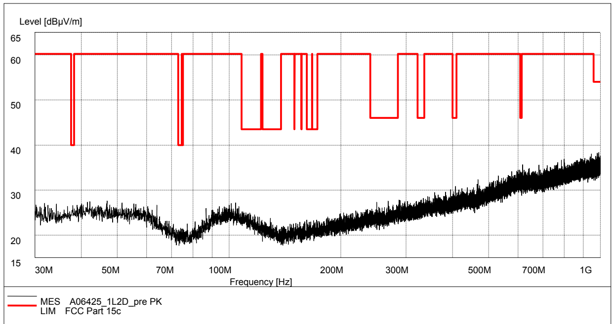
Fig.70. Radiated emission: \pi/4 DQPSK, Channel 0, 30 MHz - 1 GHz
