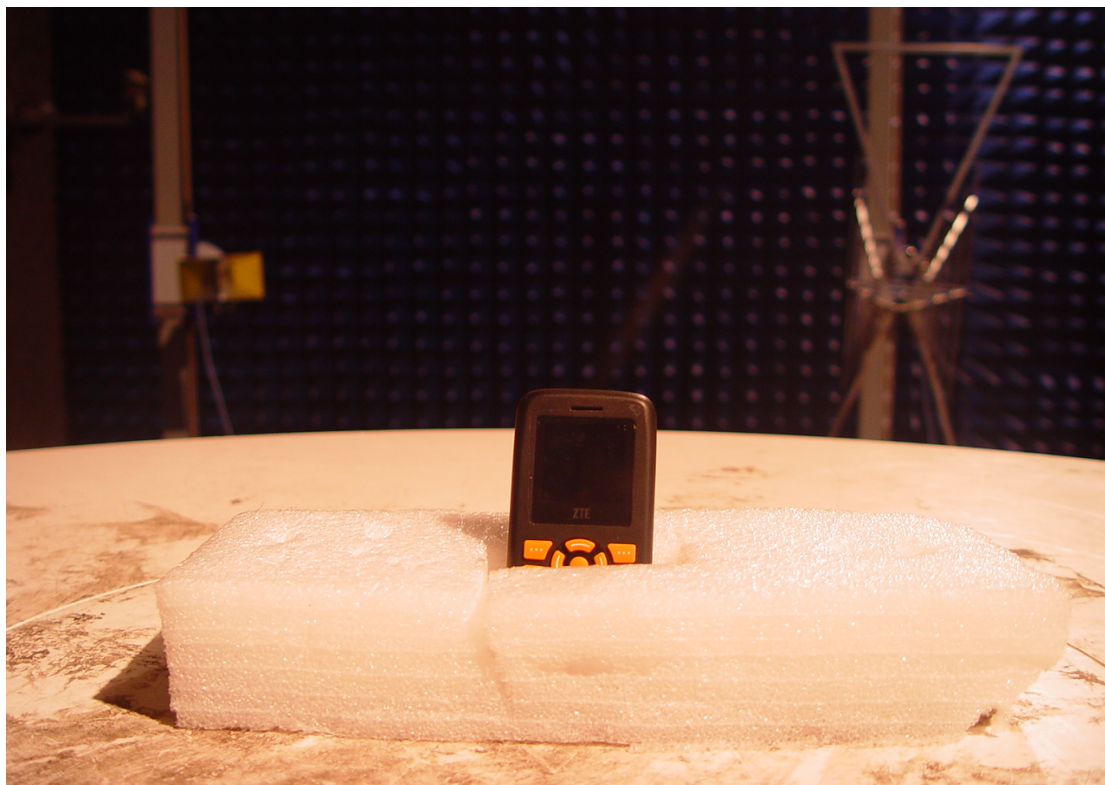
Radiated Spurious Emissions Test setup
