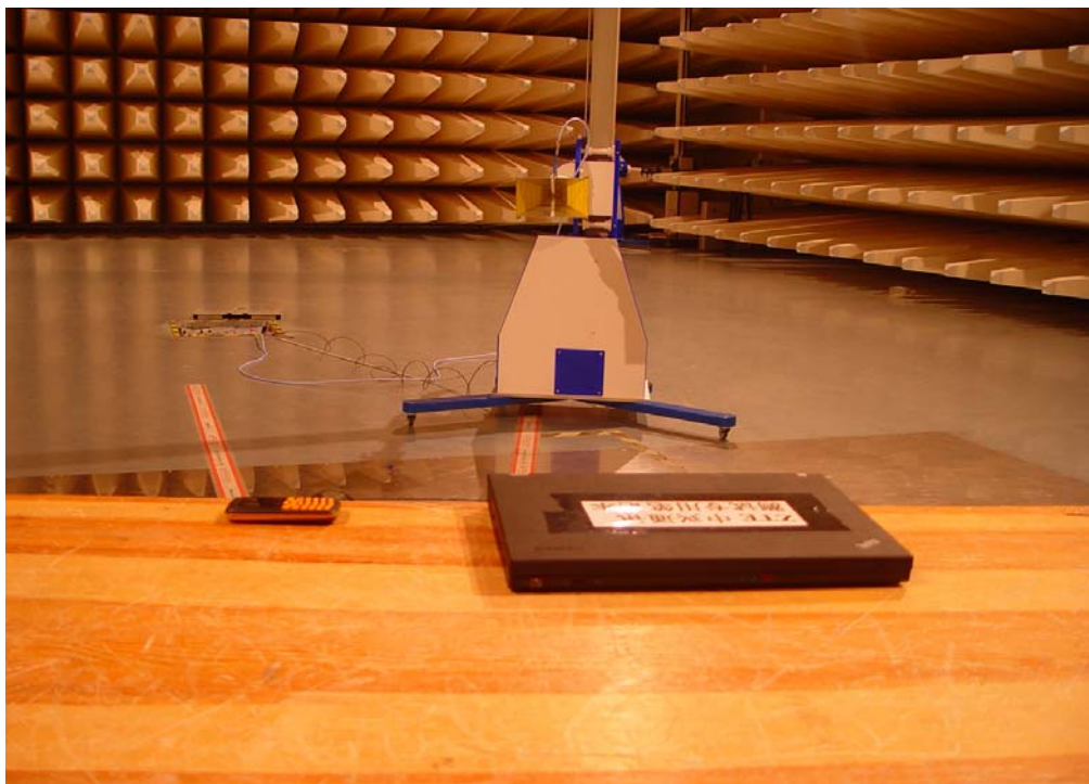
Radiated Emissions Test Setup
