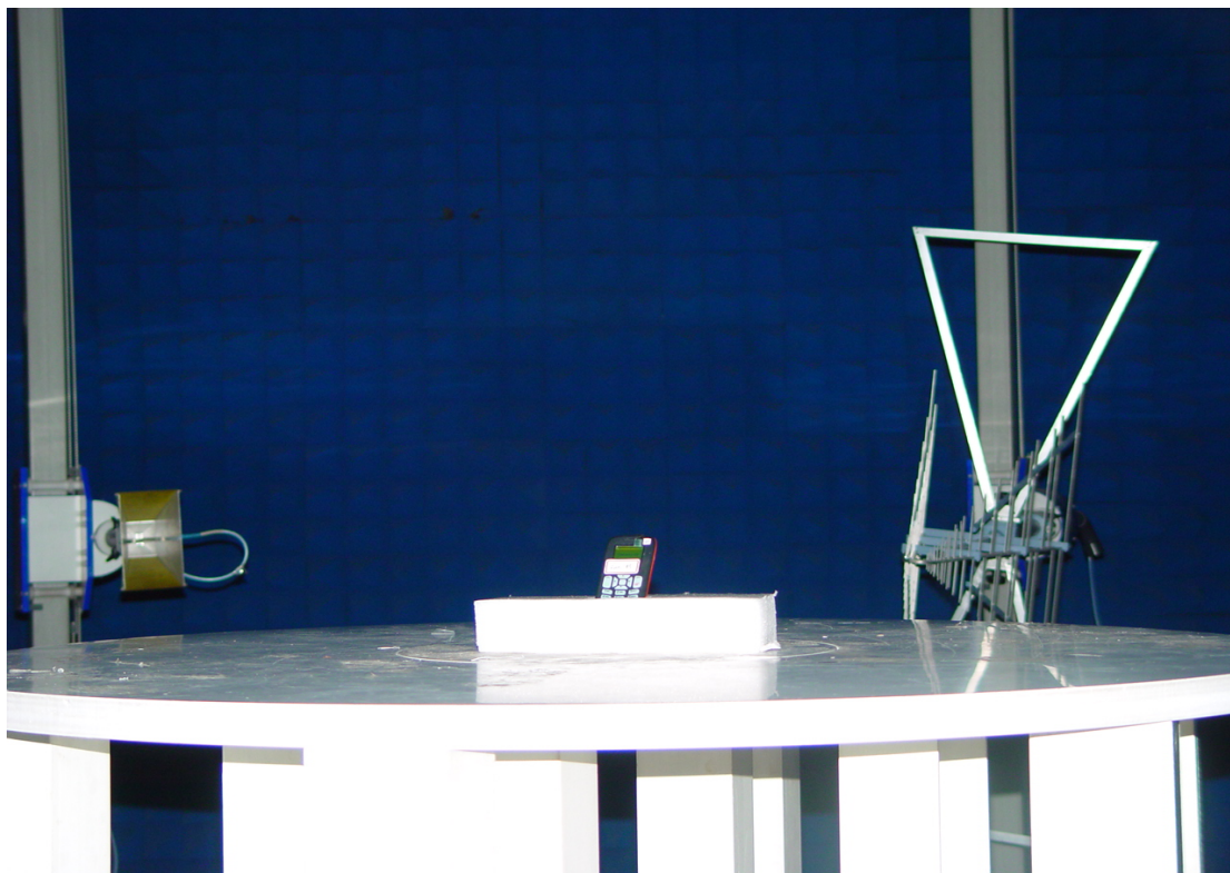
Radiated Spurious Emissions Test setup_1
