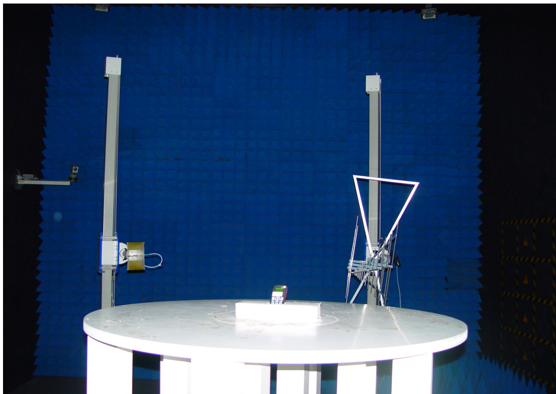
Radiated Spurious Emissions Test setup_2
