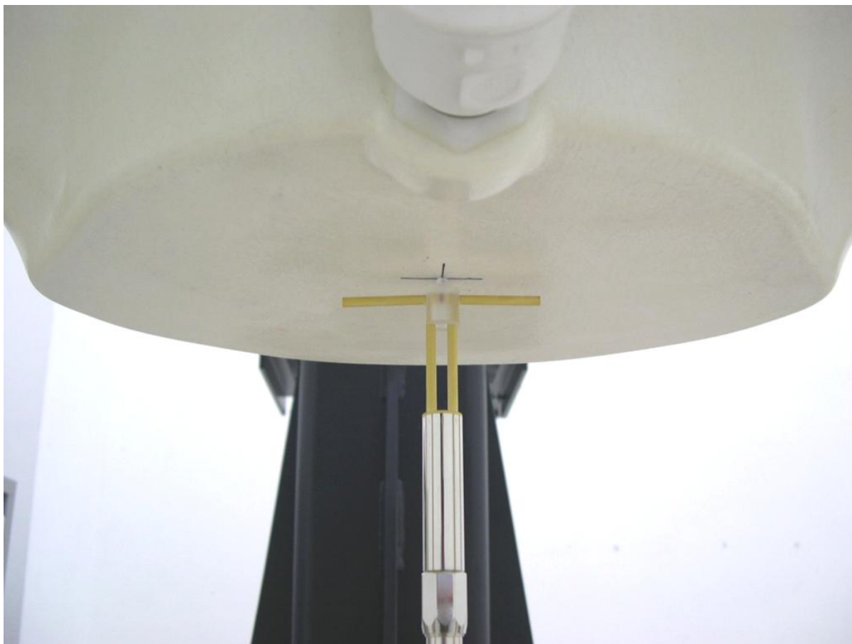
Fig 8.2 Dipole Setup
