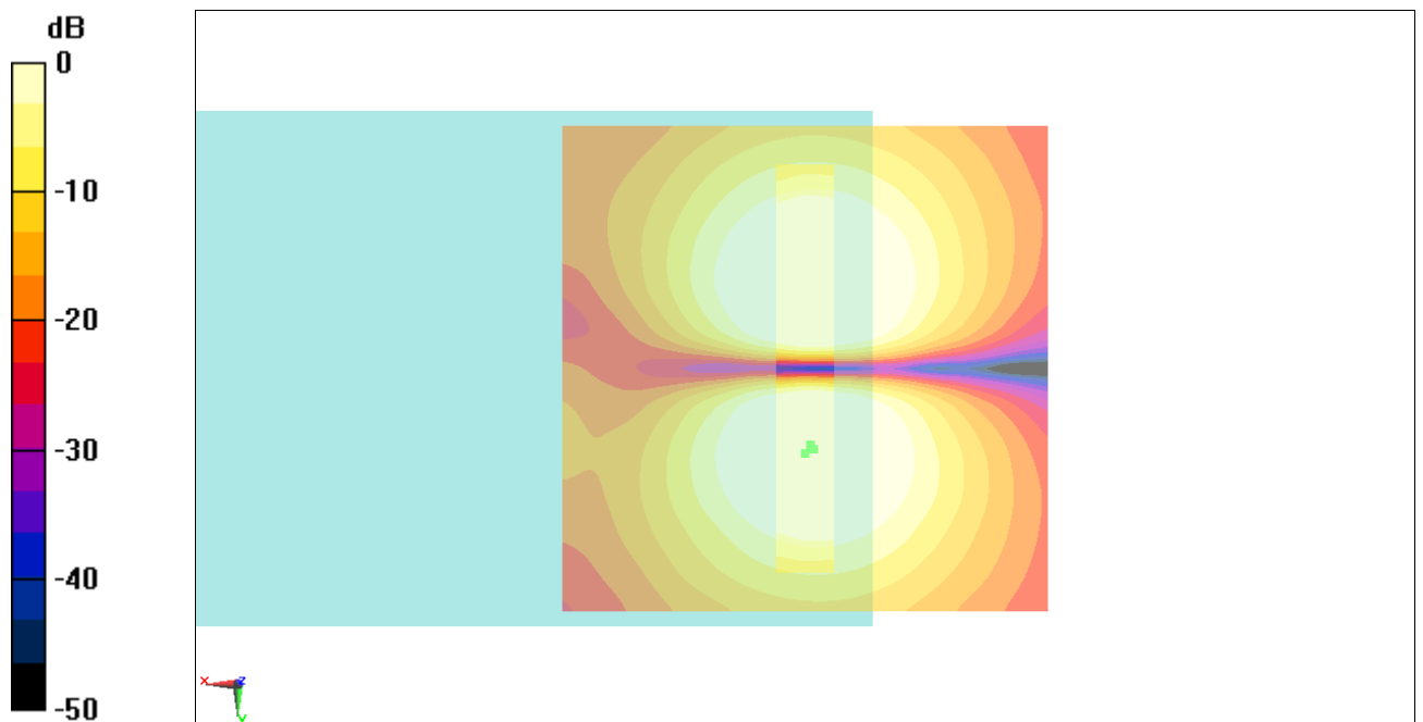
Fig B.2 T-Coil GSM 850
