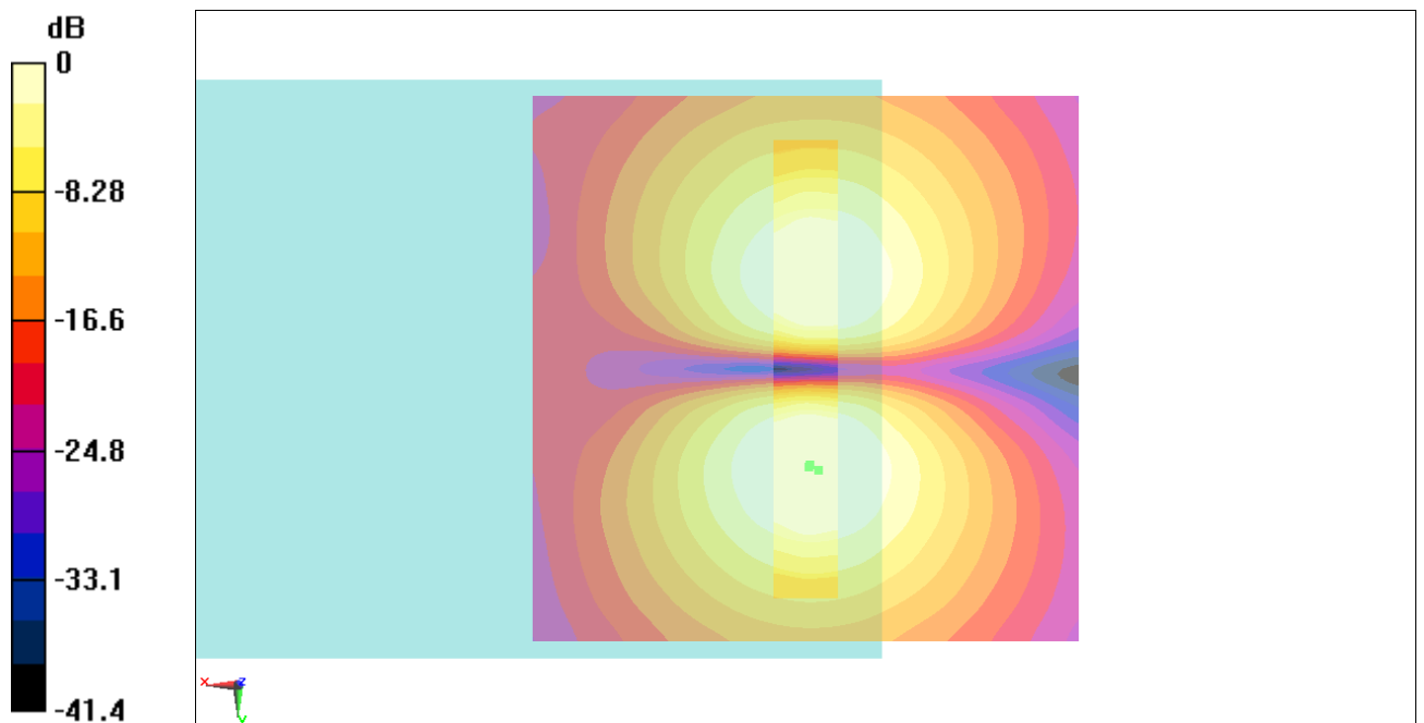
Fig B.5 T-Coil GSM 1900
