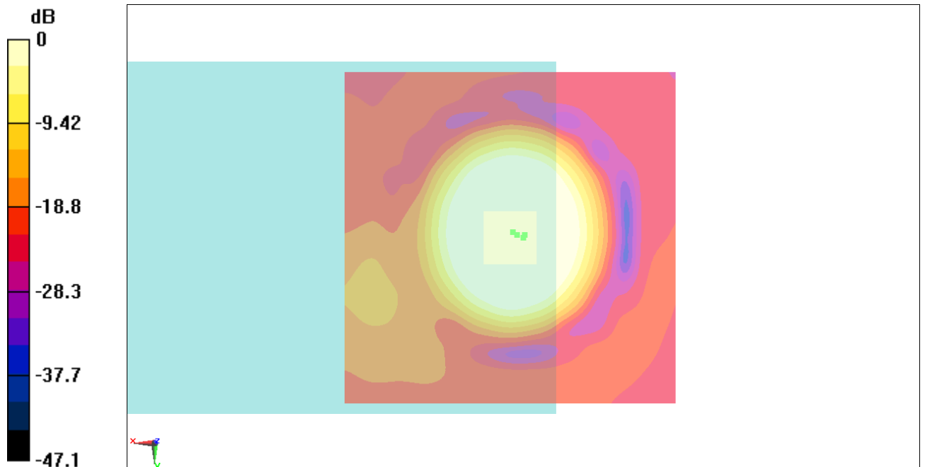
Fig B.6 T-Coil GSM 1900
