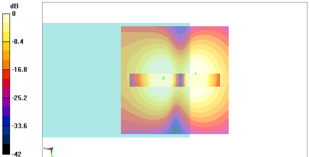
Fig B.4 T-Coil GSM 1900
