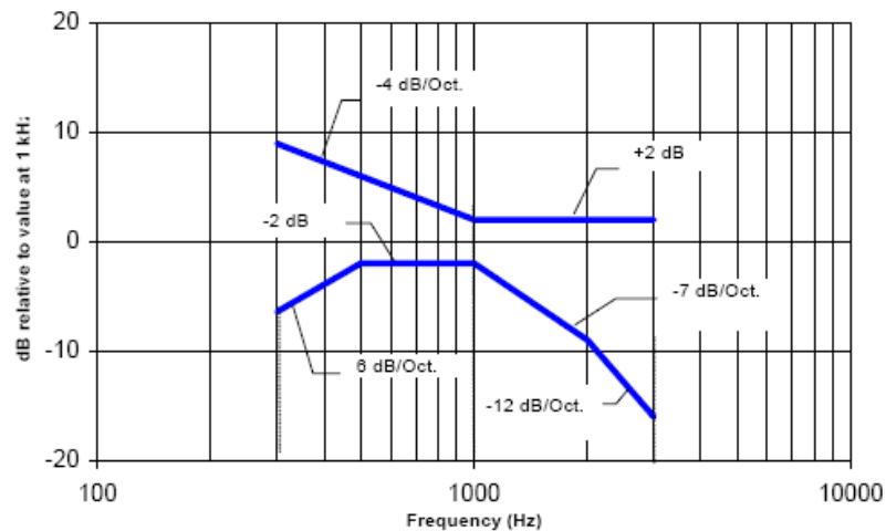
Figure 8.1—Magnetic field frequency response for WDs with a field \leq -15 dB (A/m) at 1 kHz
