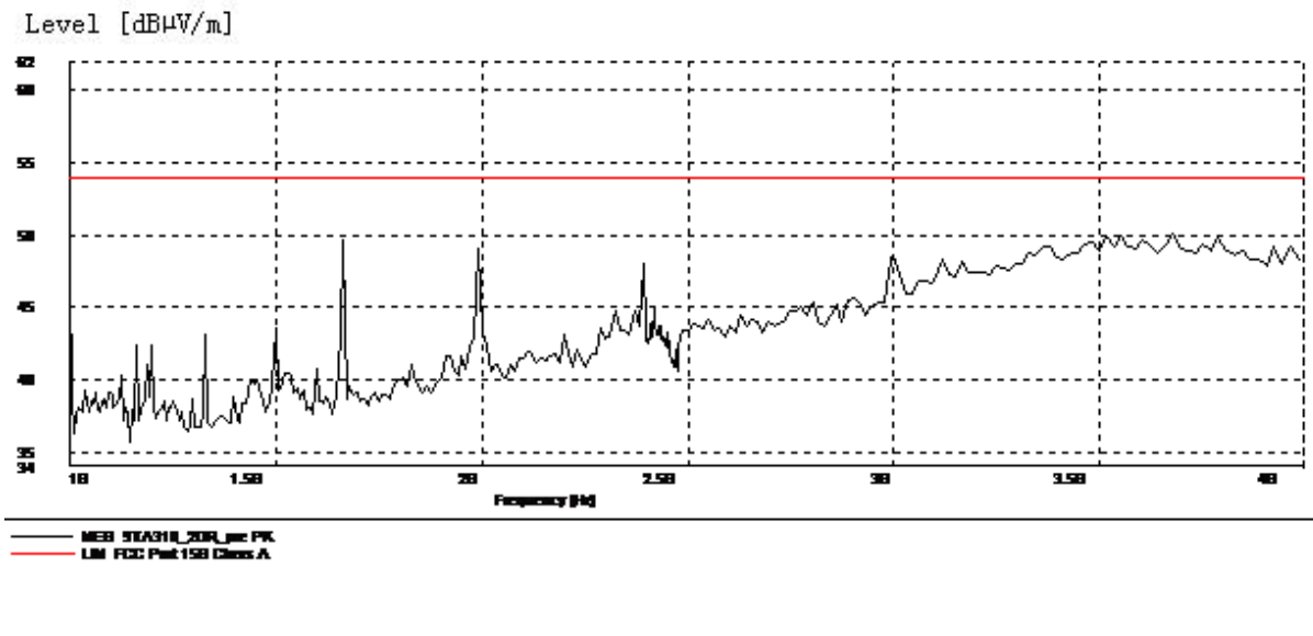
Figure A.2 Radiated Emission from 1GHz to 4GHz
