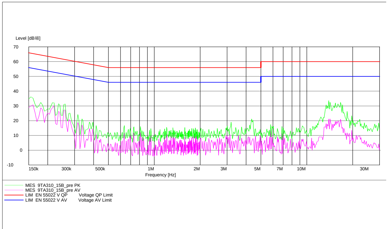
Figure A.3 Conducted Emission
