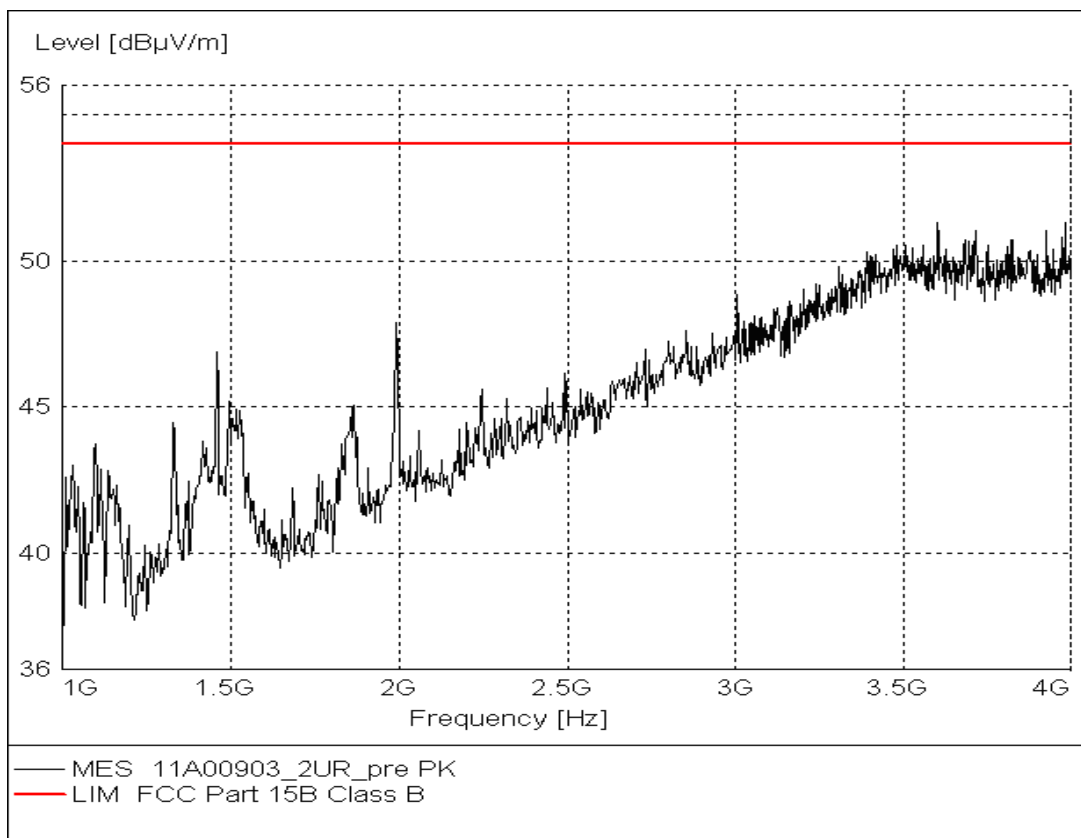
Figure A.4 Radiated Emission from 1GHz to 4GHz
