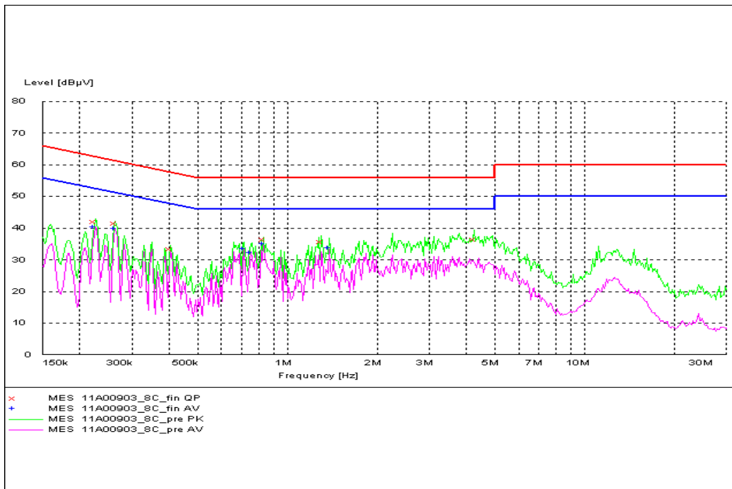
Figure A.6 Conducted Emission
