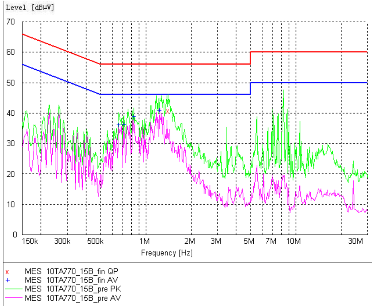
Figure A.6 Conducted Emission
