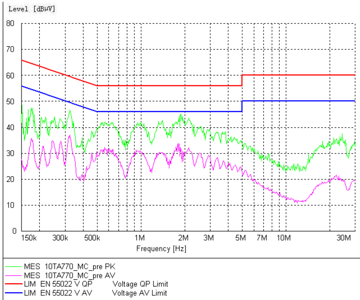
Figure A.5 Conducted Emission
