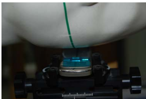
Fig 2 - Definition of the reference lines and points, on the phone and on the phantom and initial position
