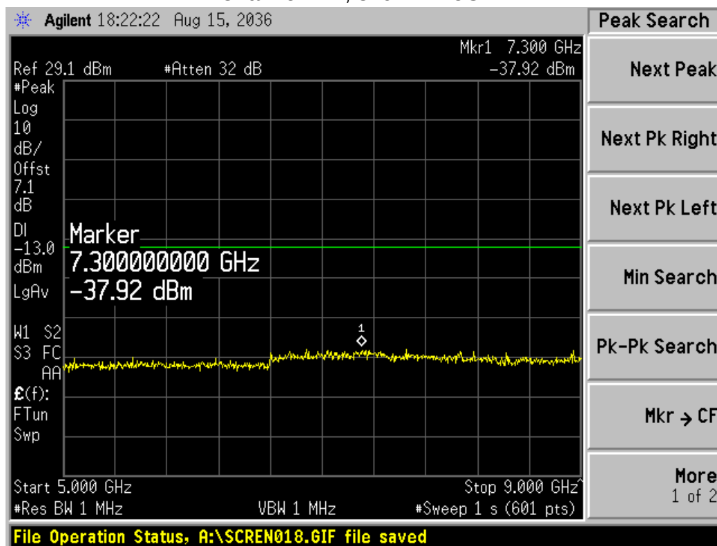
Channel 777, 5GHz~9GHz
