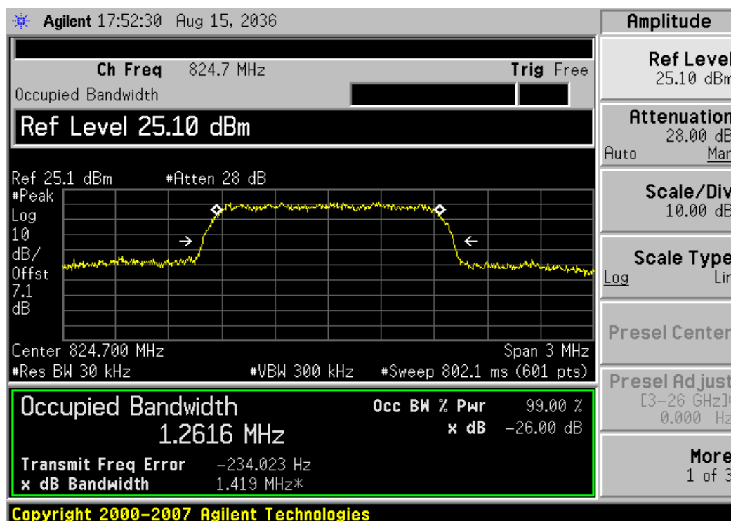
Channel 1013
