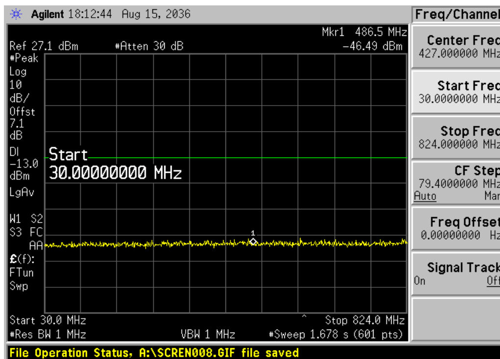
Channel 384, 30MHz~824MHz
