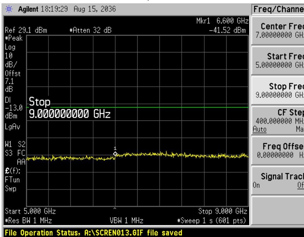
Channel 384, 5GHz~9GHz
