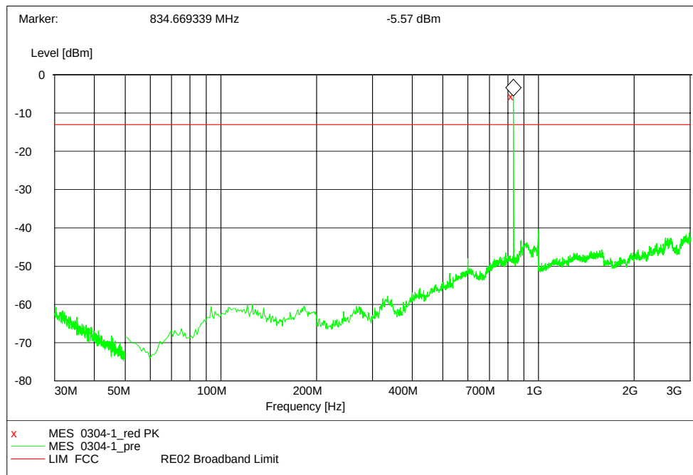
Channel 384, 30MHz~3GHz
