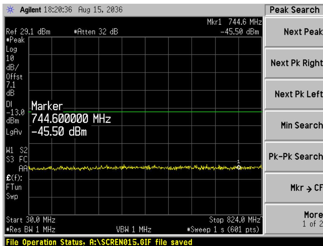
Channel 777, 30MHz~824MHz
