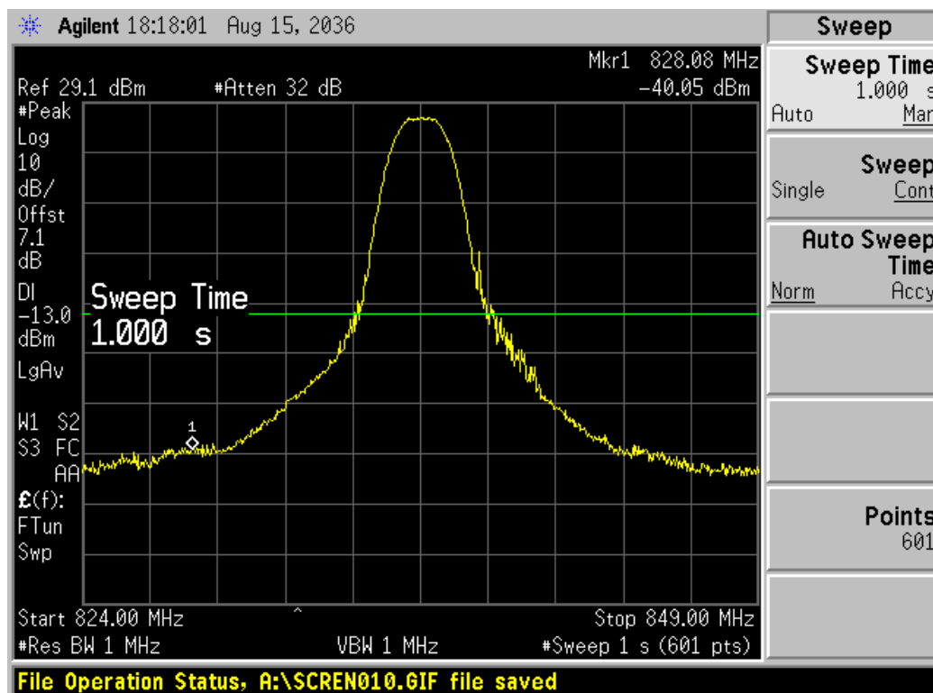
Channel 384, 824MHz~849MHz
