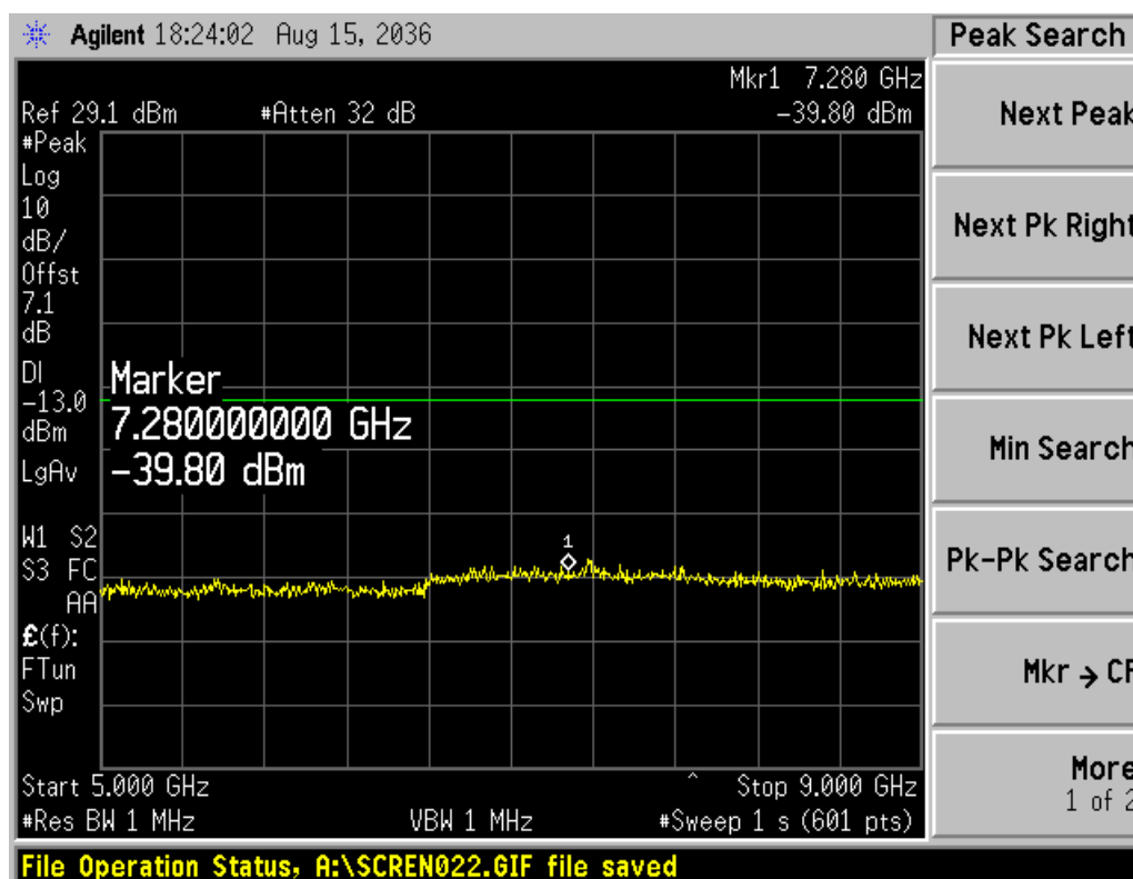
Channel 1013, 5GHz~9GHz
