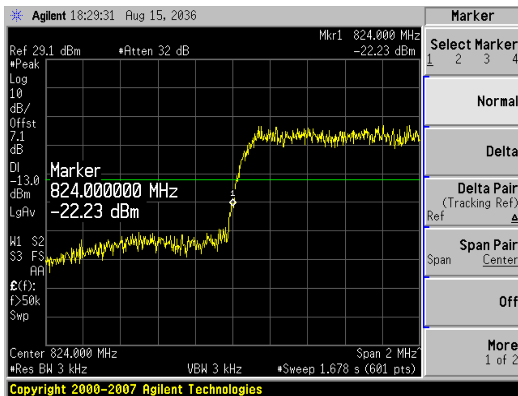
Channel 1013
