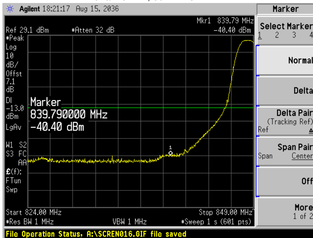
Channel 777, 824MHz~849MHz
