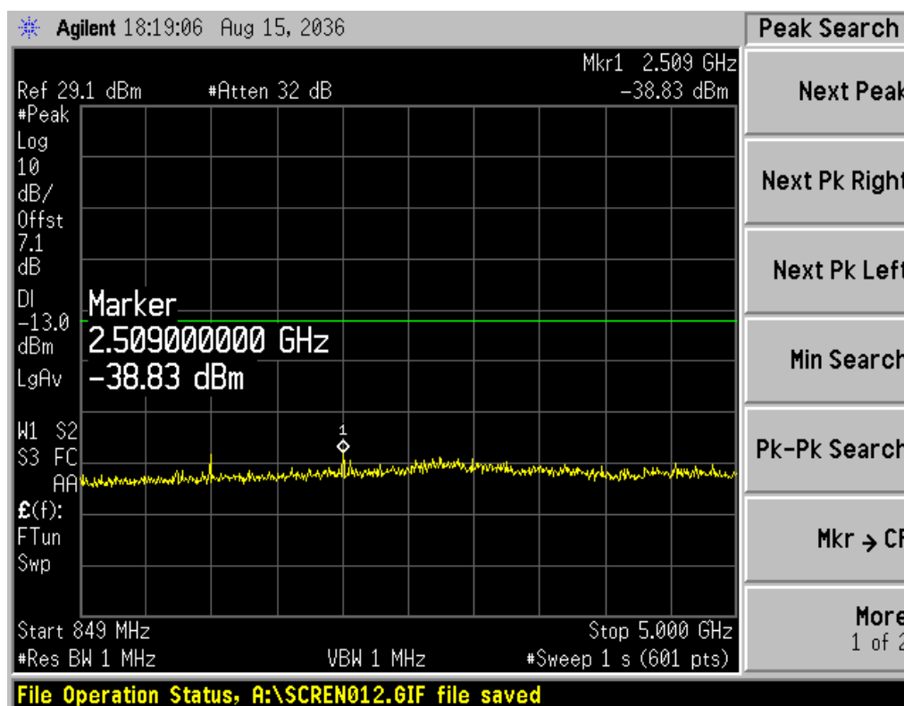
Channel 384, 849MHz~5GHz
