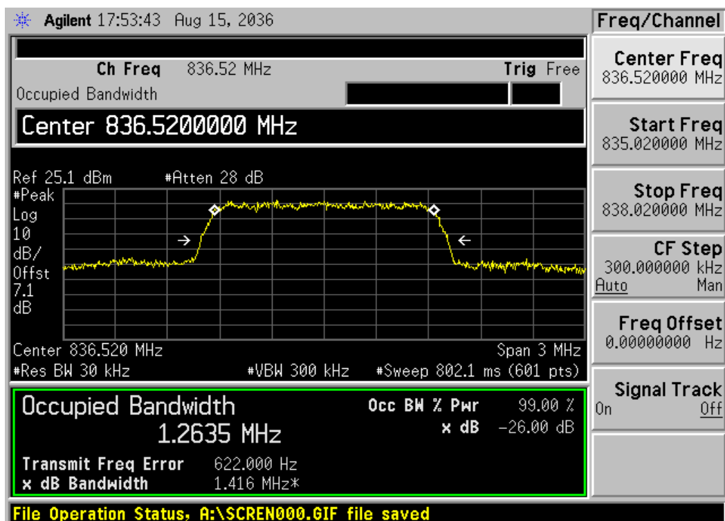
Channel 384
