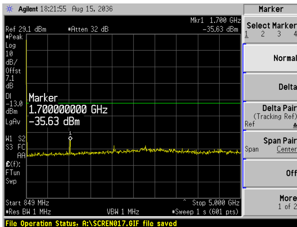
Channel 777, 849MHz~5GHz
