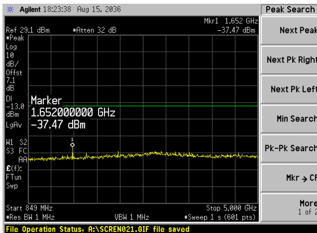
Channel 1013, 849MHz~5GHz
