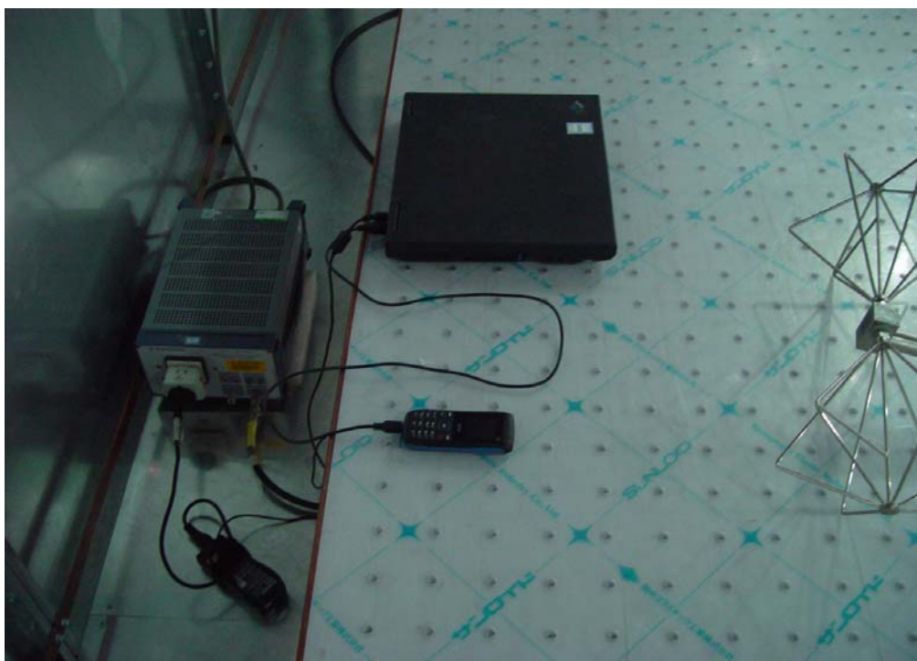
Conducted Emissions Test Setup
