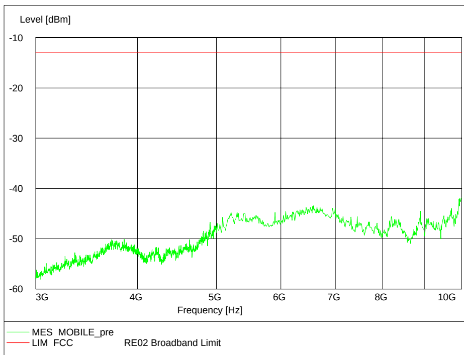
Channel 384, 3GHz~10GHz
