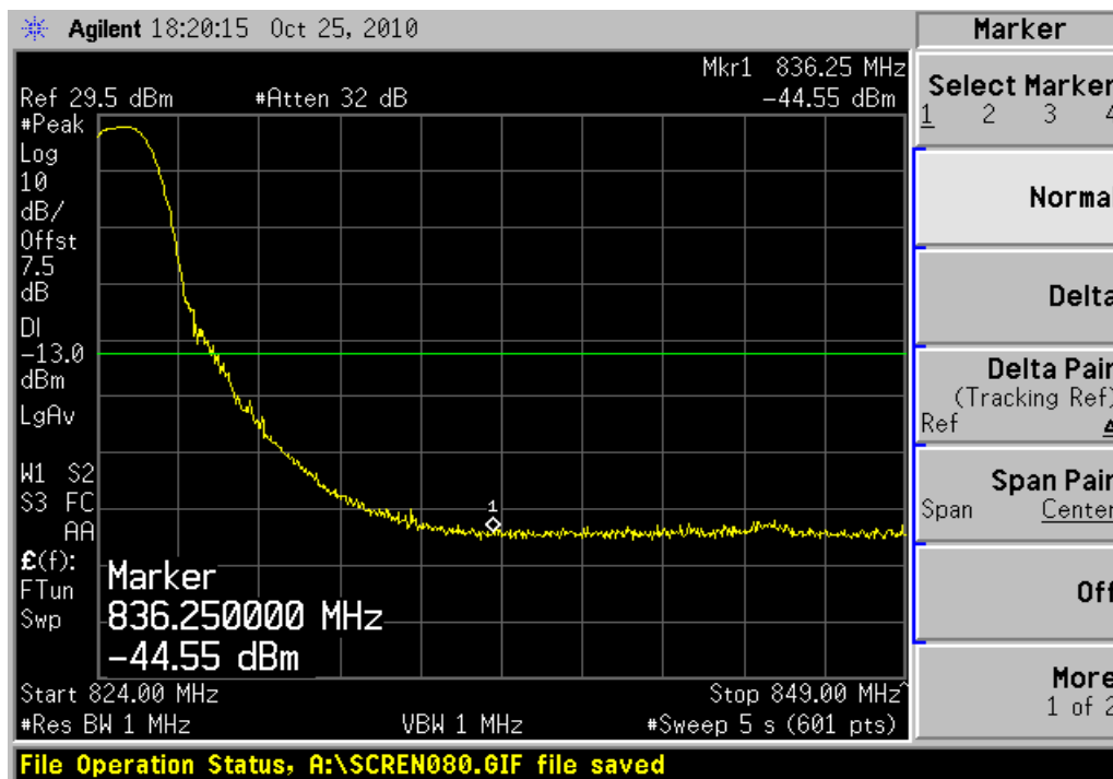
Channel 1013, 824MHz~849MHz
