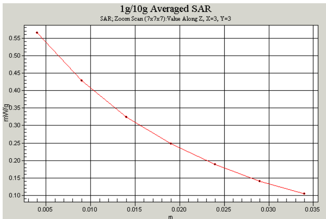
Z-Scan at power reference point (824.7 MHz CH1013)
