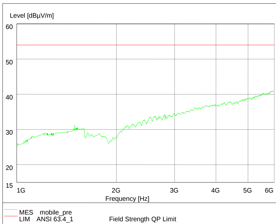
Pic.4 CDMA 1X (1GHz – 6GHz)
