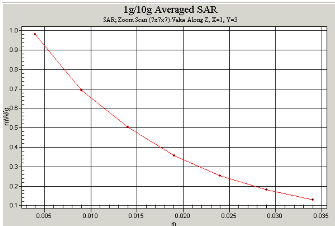
Z-Scan at power reference point (836.52 MHz CH384)
