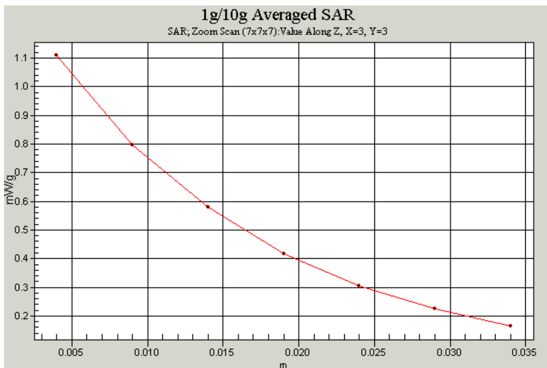
Z-Scan at power reference point (848.31 MHz CH777)
