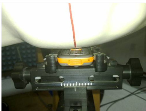
Definition of the reference lines and points, on the phone and on the phantom and initial position
