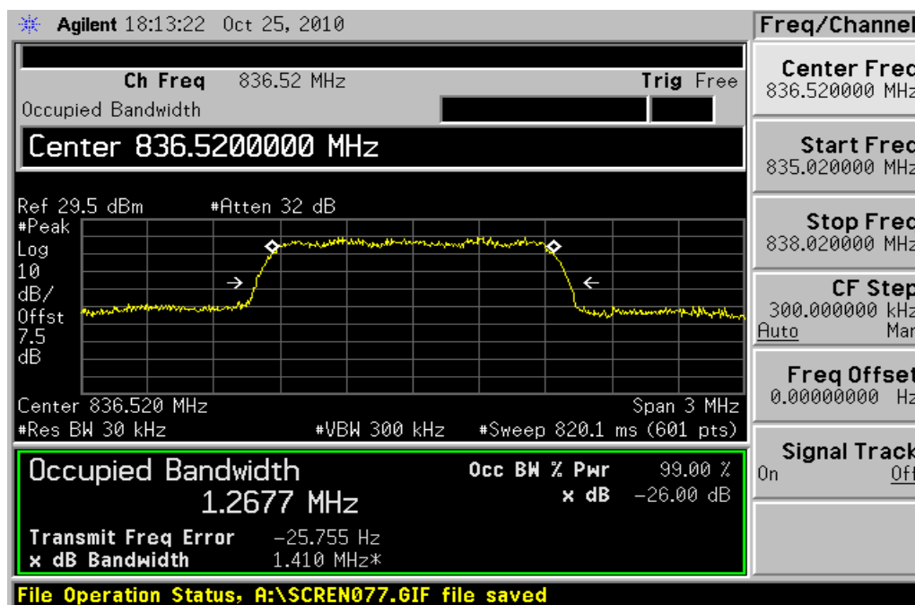
Channel 384
