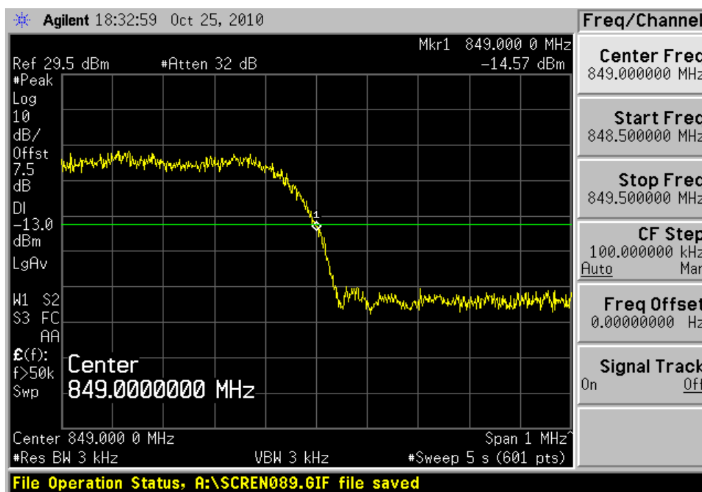
Channel 777
