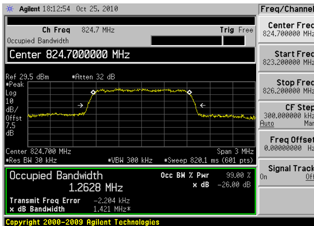
Channel 1013
