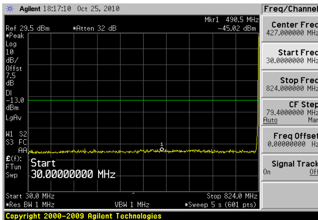
Channel 1013, 30MHz~824MHz
