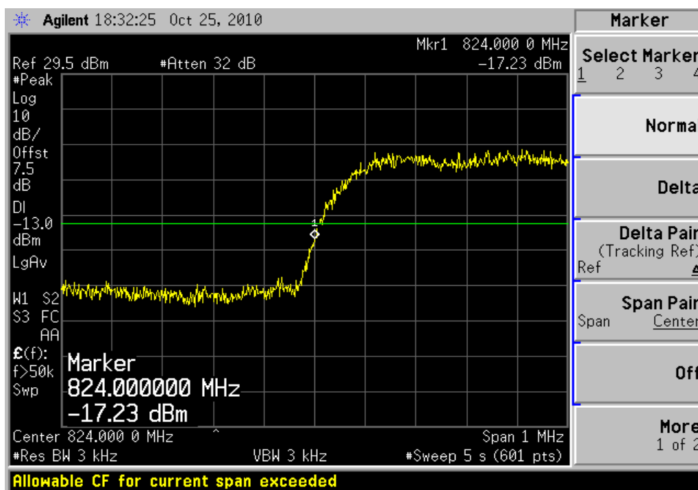
Channel 1013
