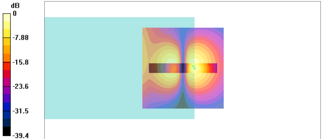
Fig B.4 T-Coil GSM 1900
