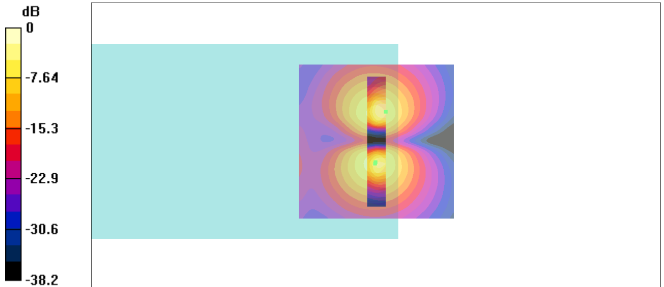
Fig B.2 T-Coil GSM 850
