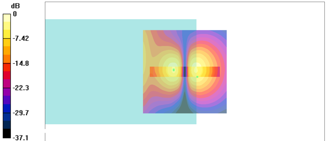
Fig B.1 T-Coil GSM 850
