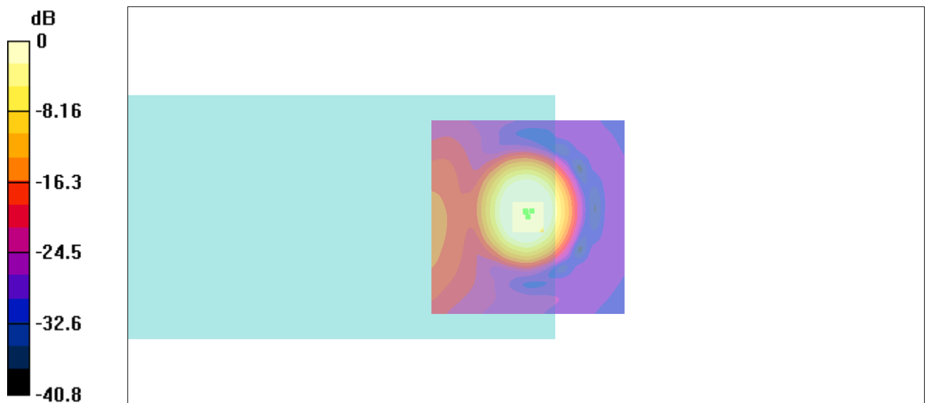
Fig B.6 T-Coil GSM 1900
