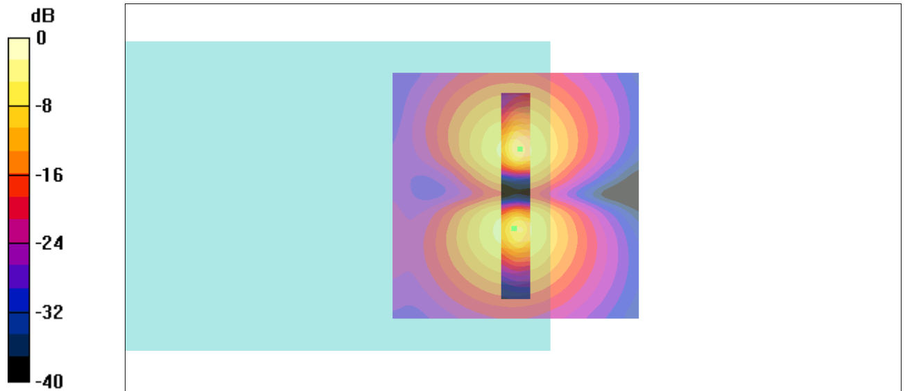
Fig B.5 T-Coil GSM 1900
