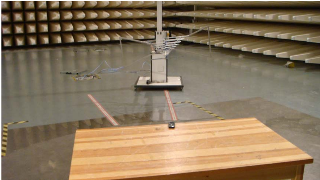
Pic 3 Radiated Emissions Test Setup
