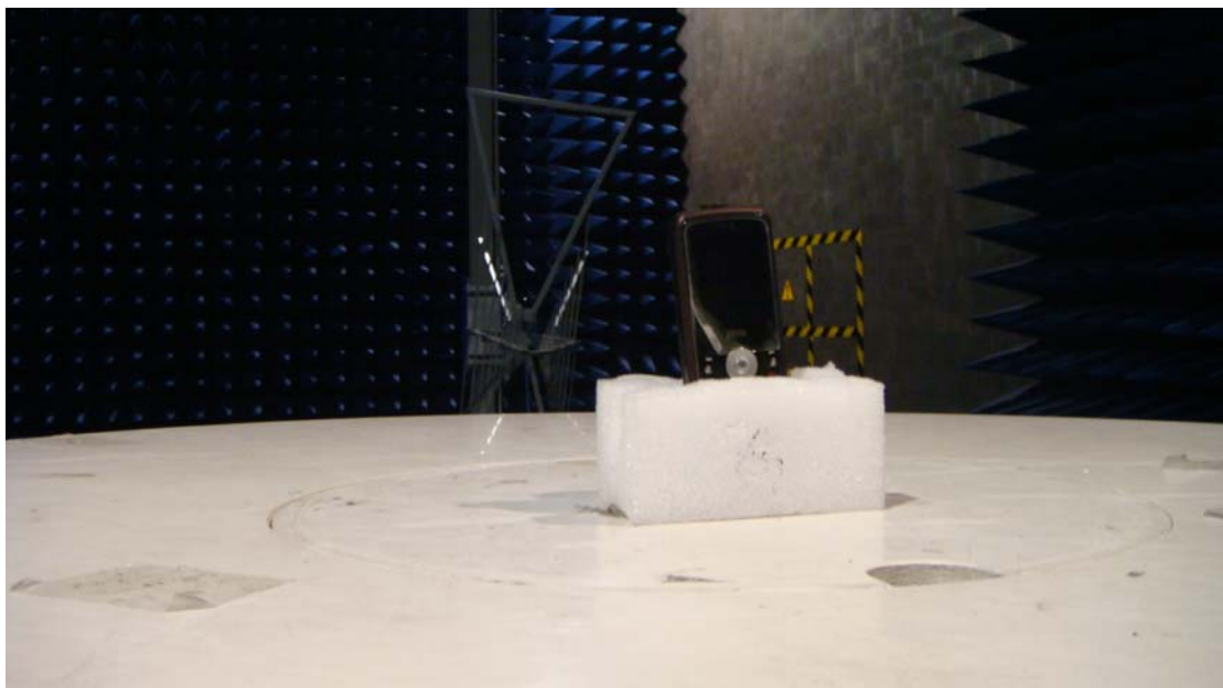
Pic 2 Radiated Spurious Emissions Test Setup
