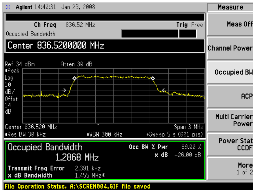
Channel 384
