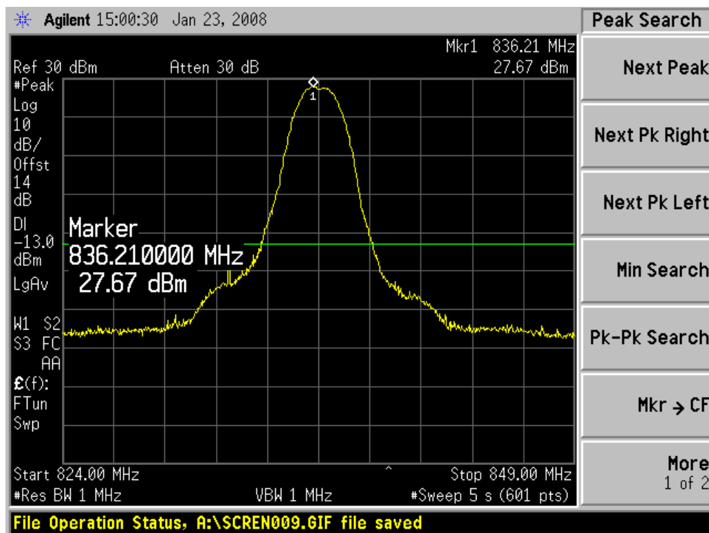
Channel 384, 824MHz~849MHz
