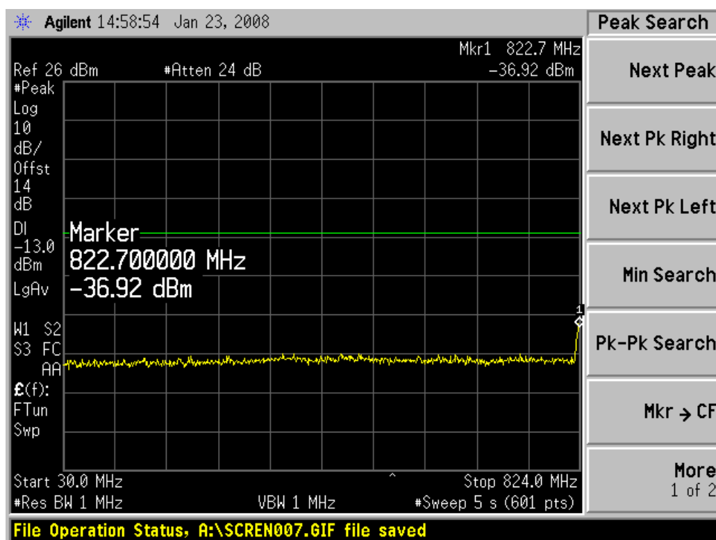
Channel 384, 30MHz~824MHz
