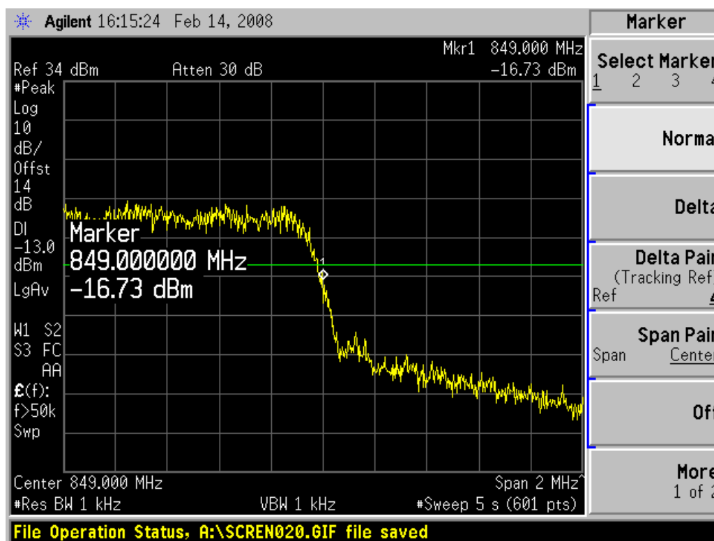
Channel 777
