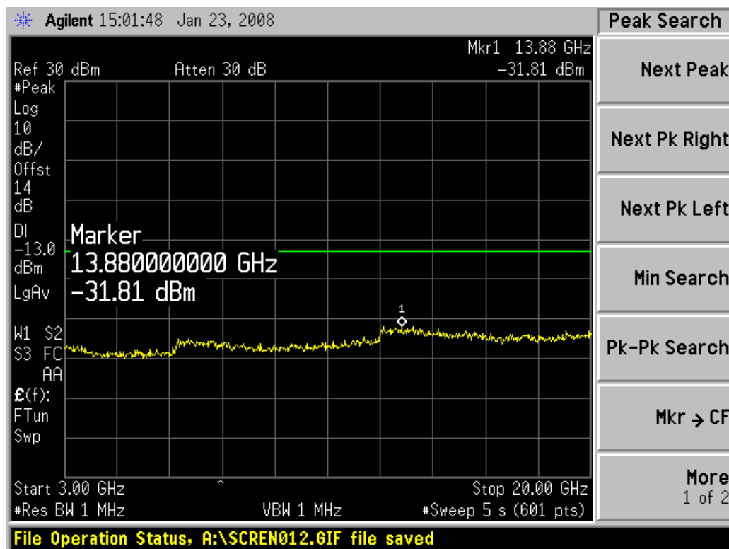
Channel 384, 3GHz~20GHz
