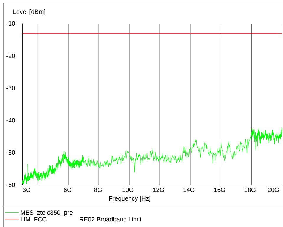
Channel 384, 3GHz~20GHz (Traffic Mode)
