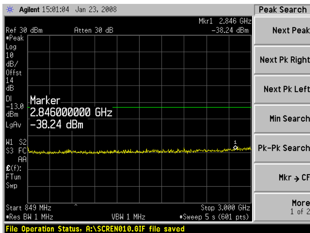
Channel 384, 849MHz~3GHz
