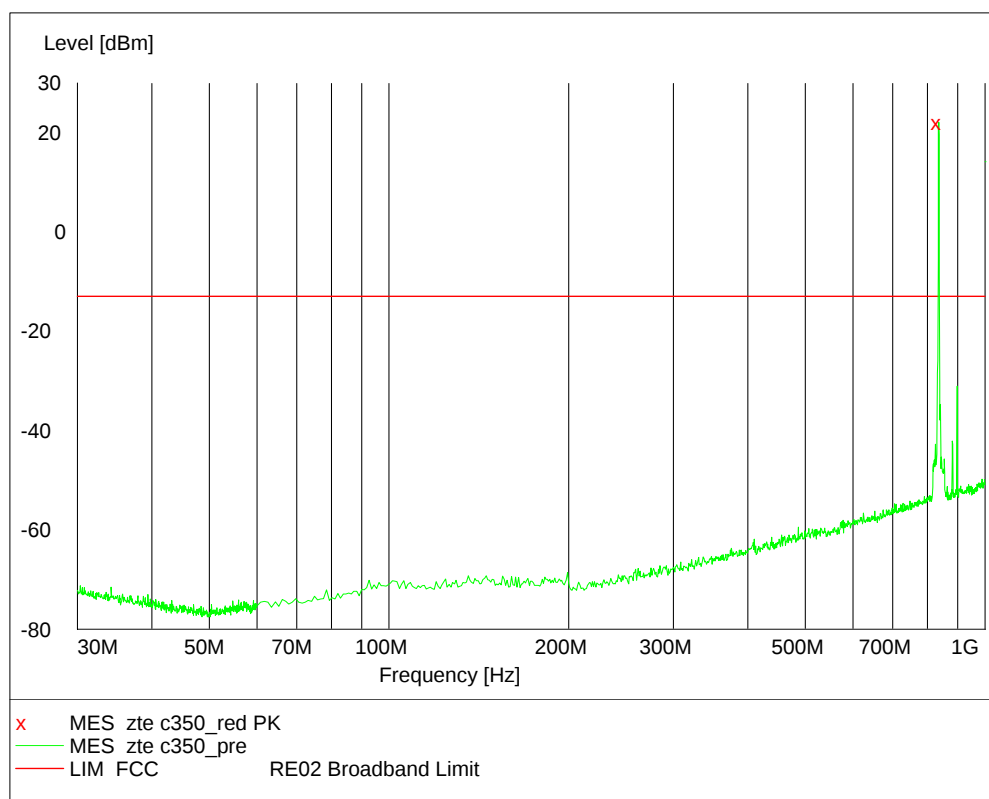
Channel 384, 30MHz~1GHz (Traffic Mode)
