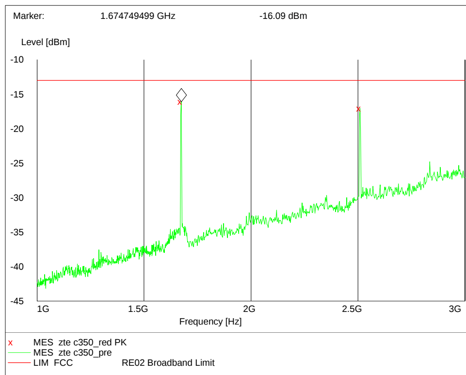
Channel 384, 1GHz~3GHz (Traffic Mode)
